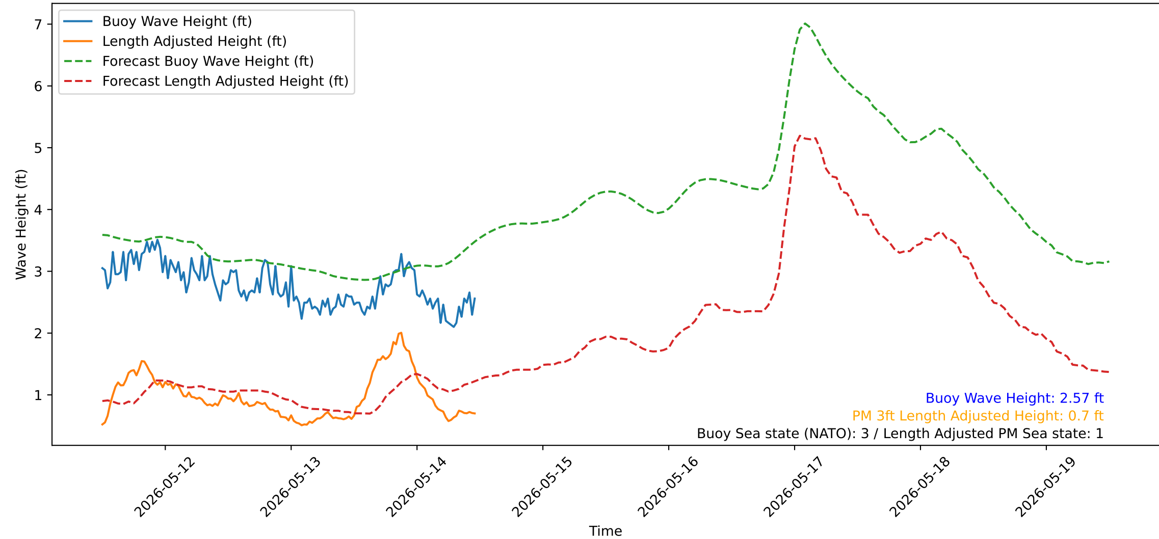
Wave Heights over Time for Green Beach at 2026-05-14 11:51:15
