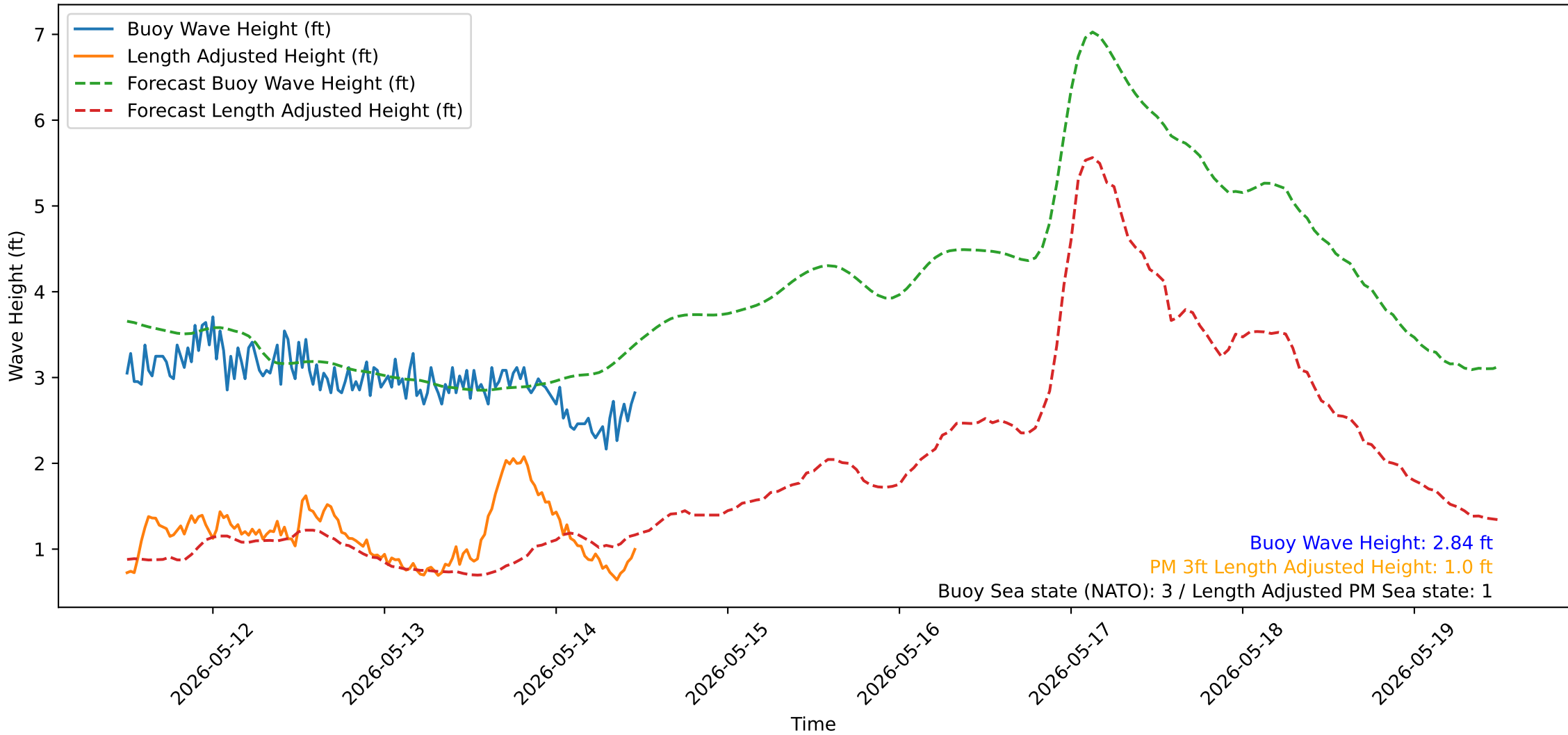
Wave Heights over Time for Oceanside Harbor at 2026-05-14 11:50:32
