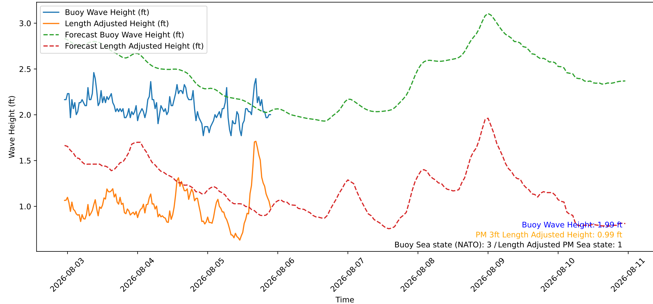
Wave Heights over Time for Red Beach at 2026-08-05 22:40:46
