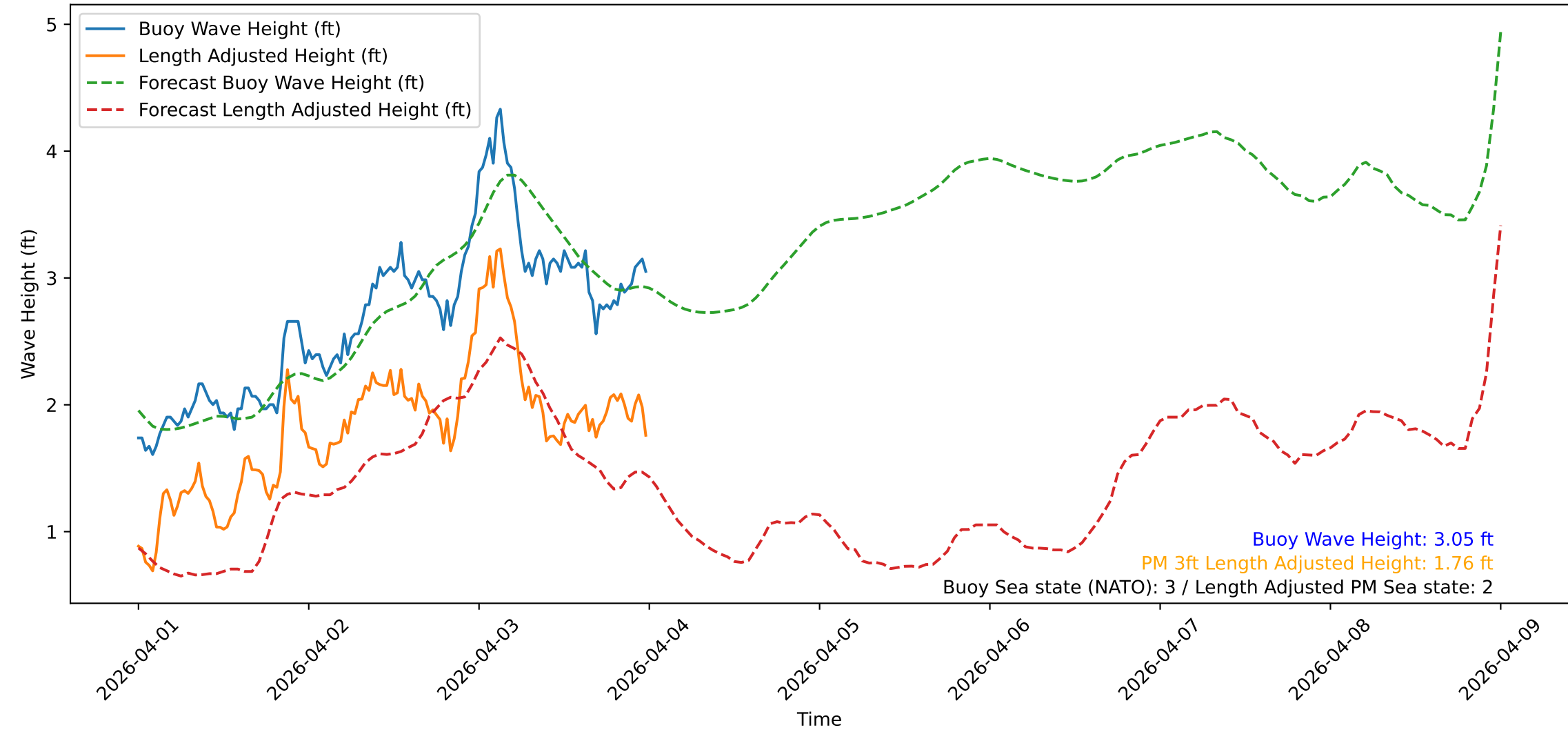
Wave Heights over Time for Green Beach at 2026-04-04 00:11:15
