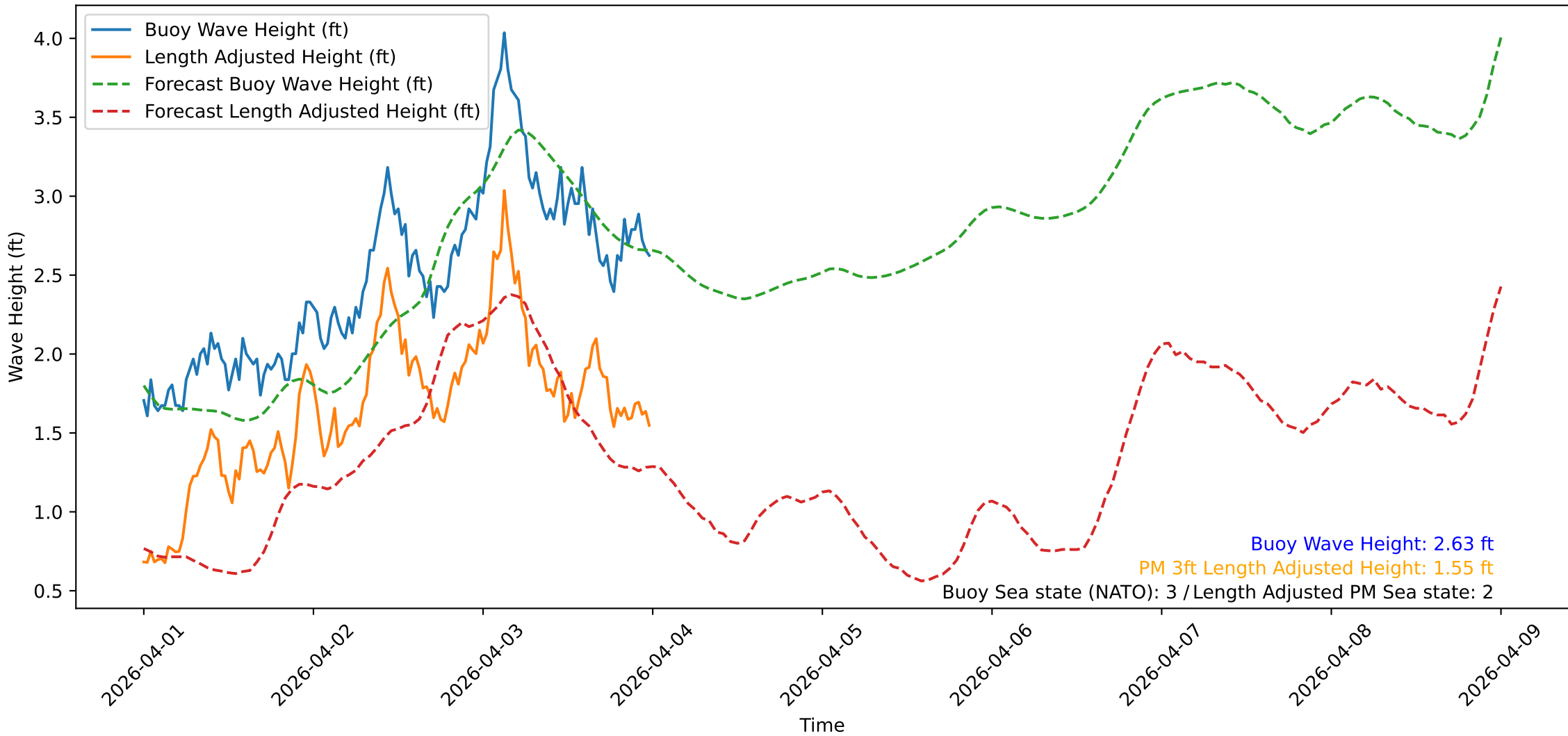
Wave Heights over Time for Oceanside Harbor at 2026-04-04 00:10:33
