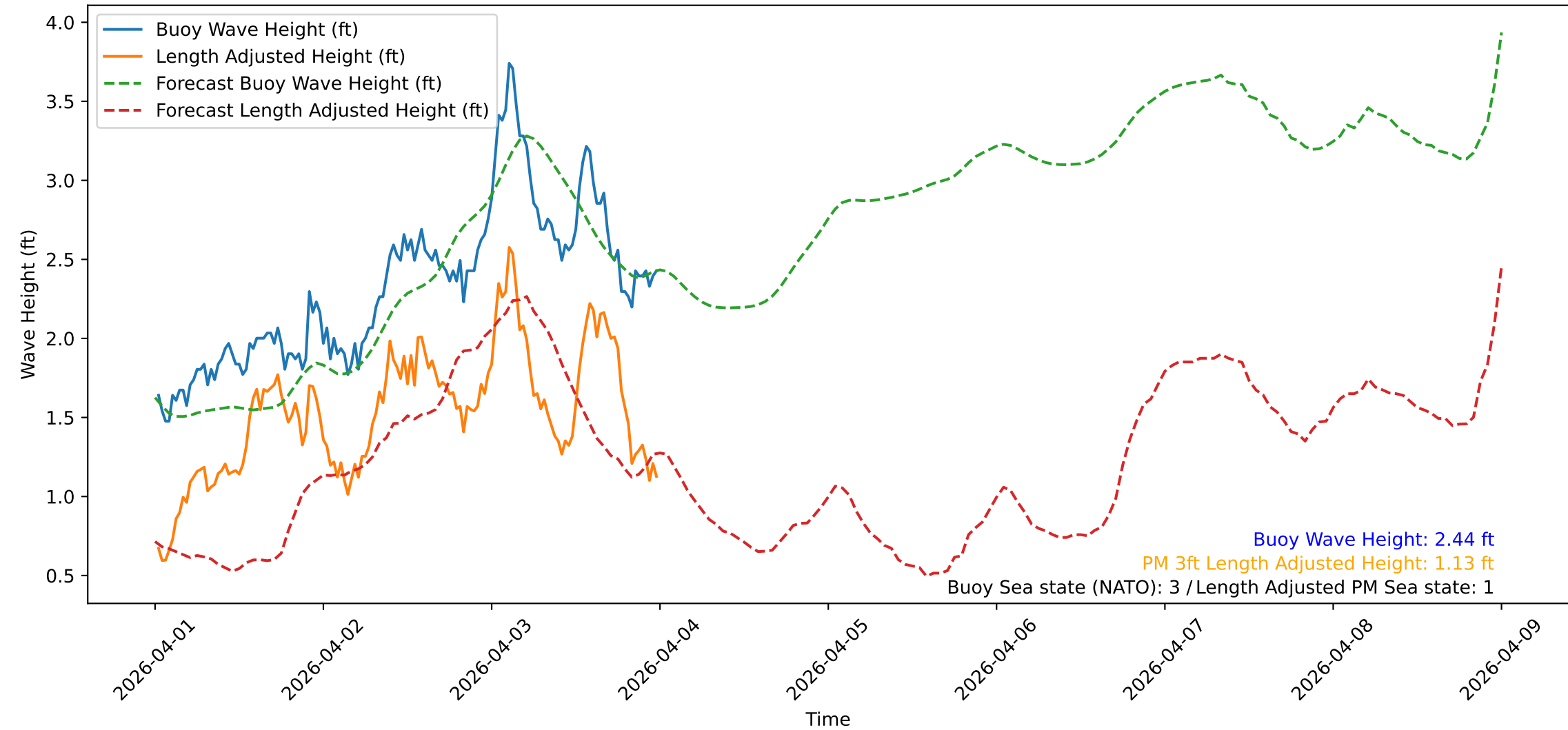
Wave Heights over Time for Red Beach at 2026-04-04 00:10:50
