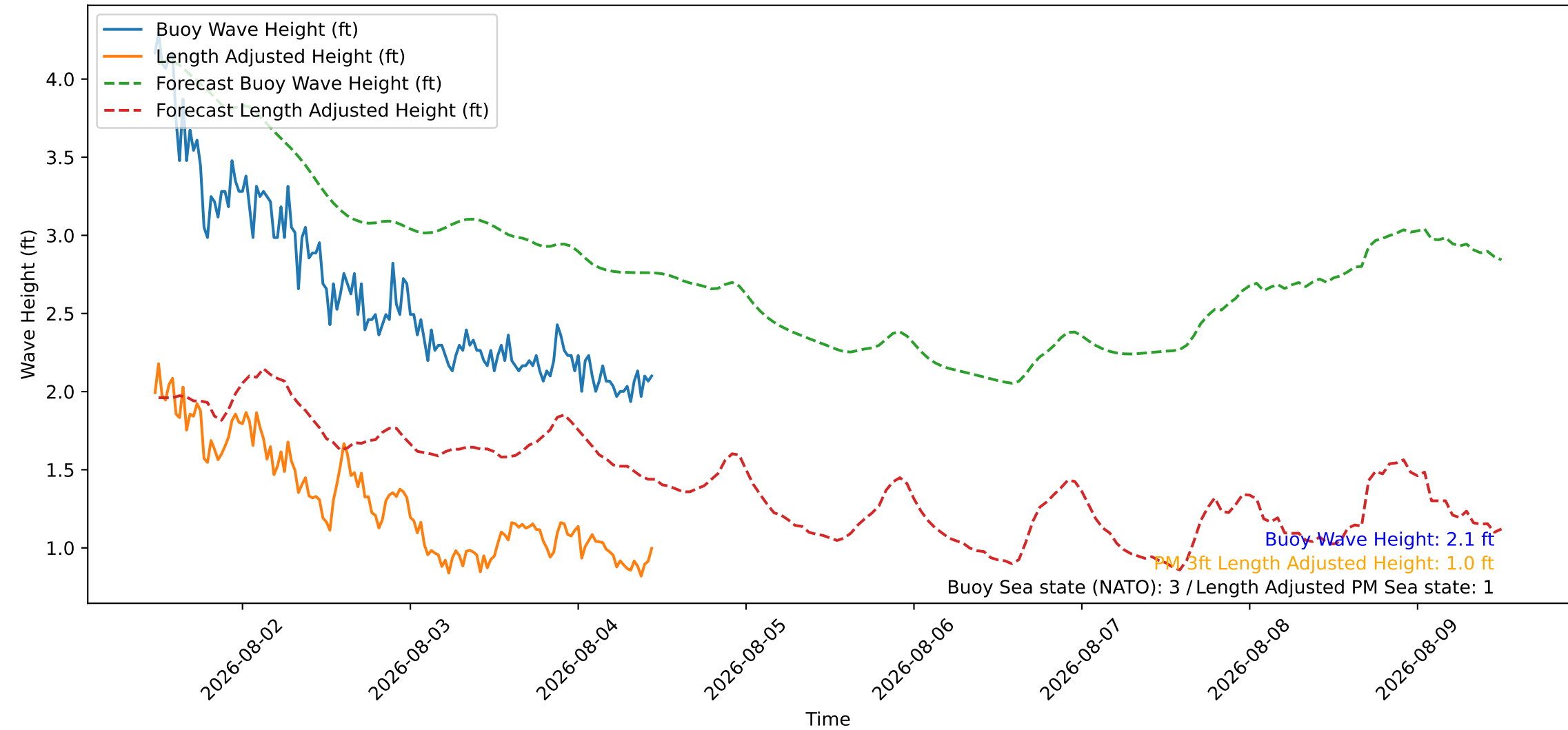
Wave Heights over Time for Green Beach at 2026-08-04 11:31:07
