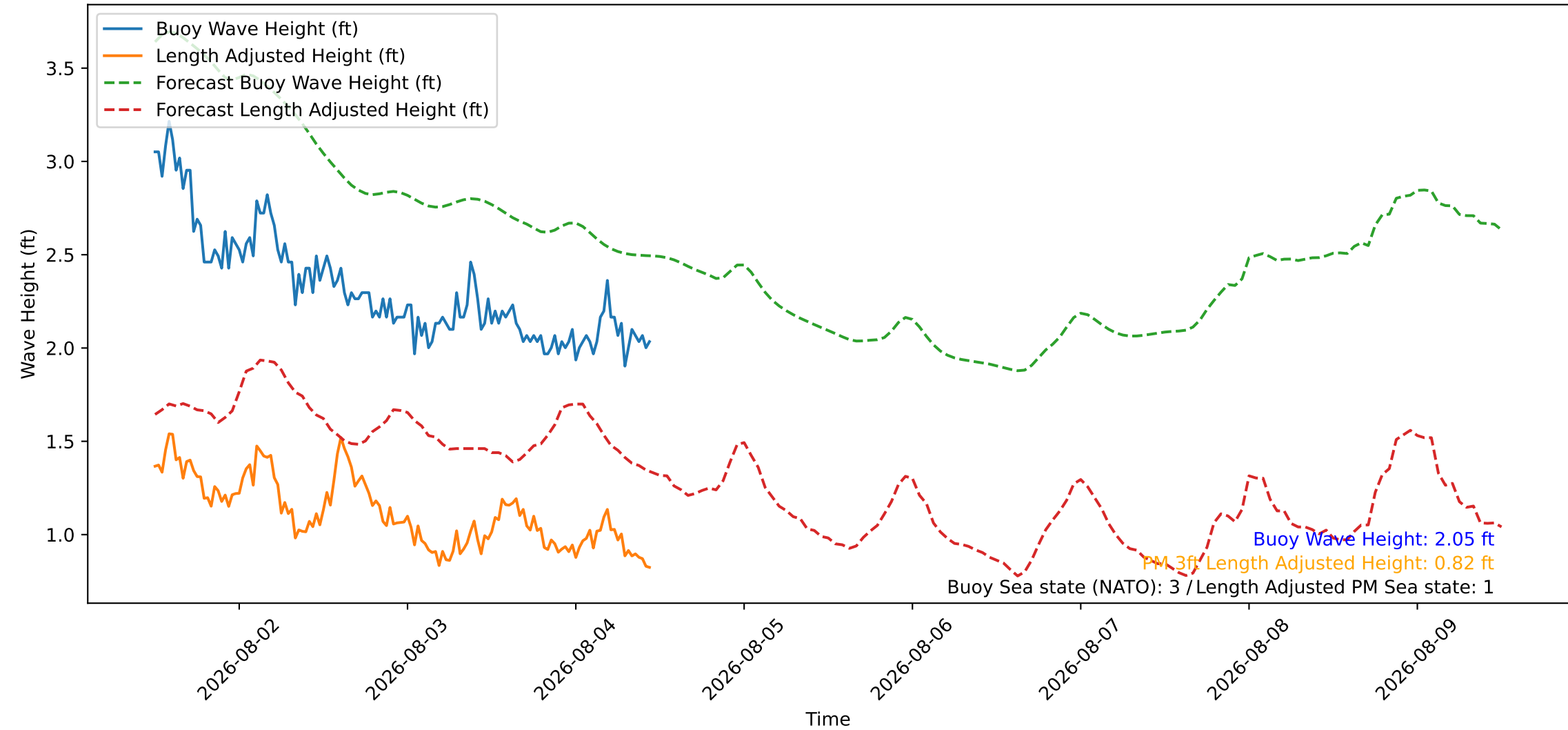
Wave Heights over Time for Red Beach at 2026-08-04 11:30:45
