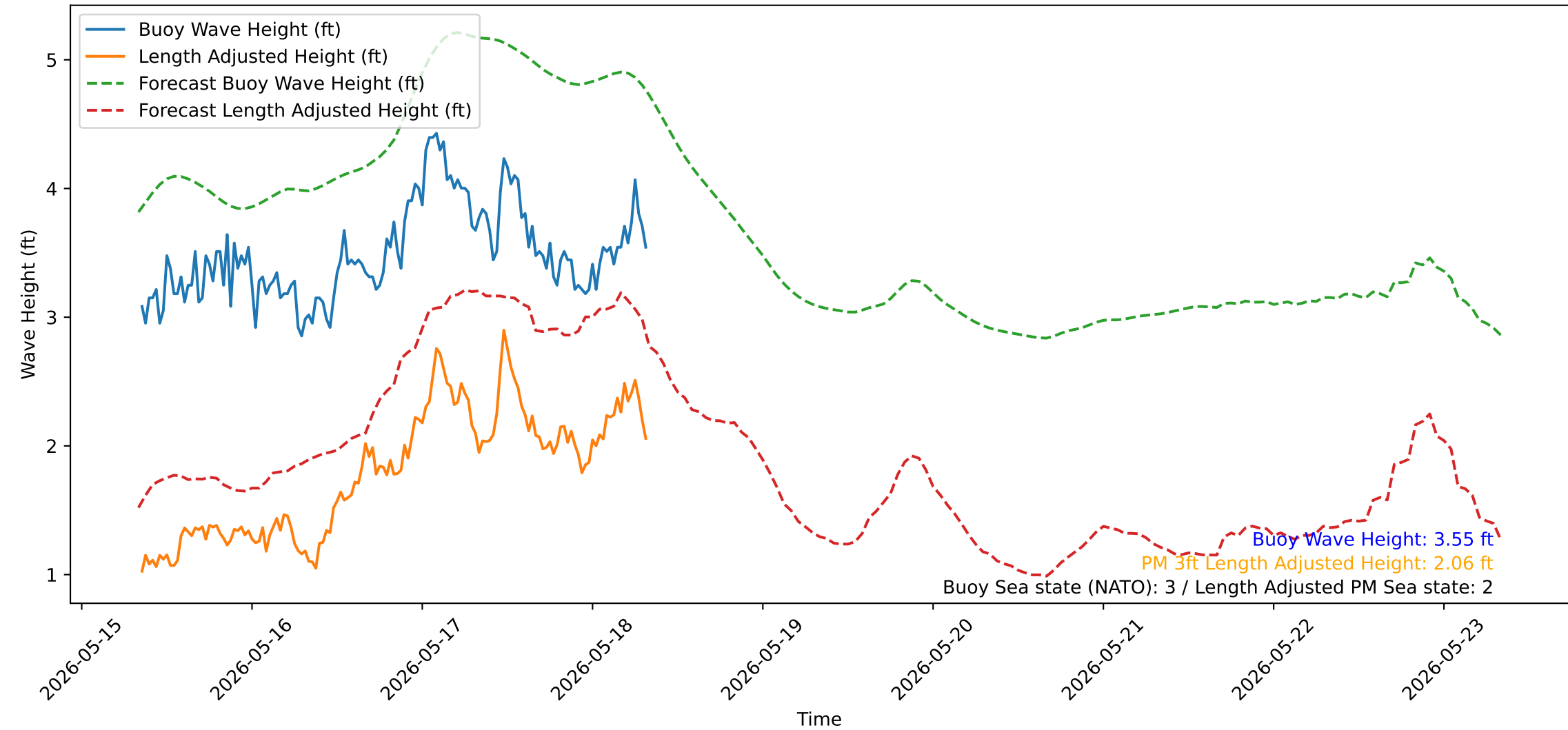
Wave Heights over Time for Green Beach at 2026-05-18 08:21:15
