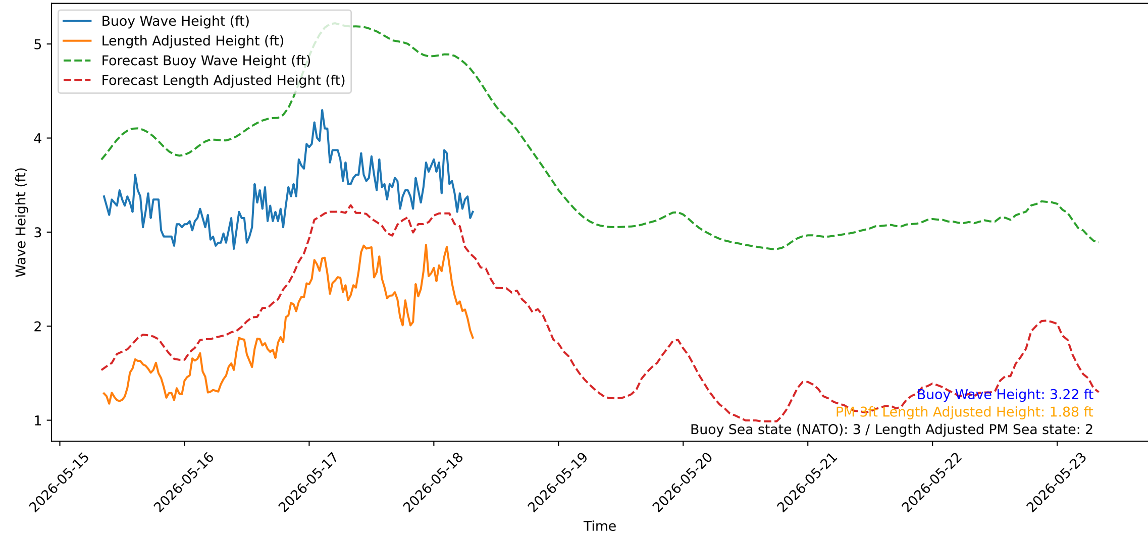
Wave Heights over Time for Oceanside Harbor at 2026-05-18 08:20:32
