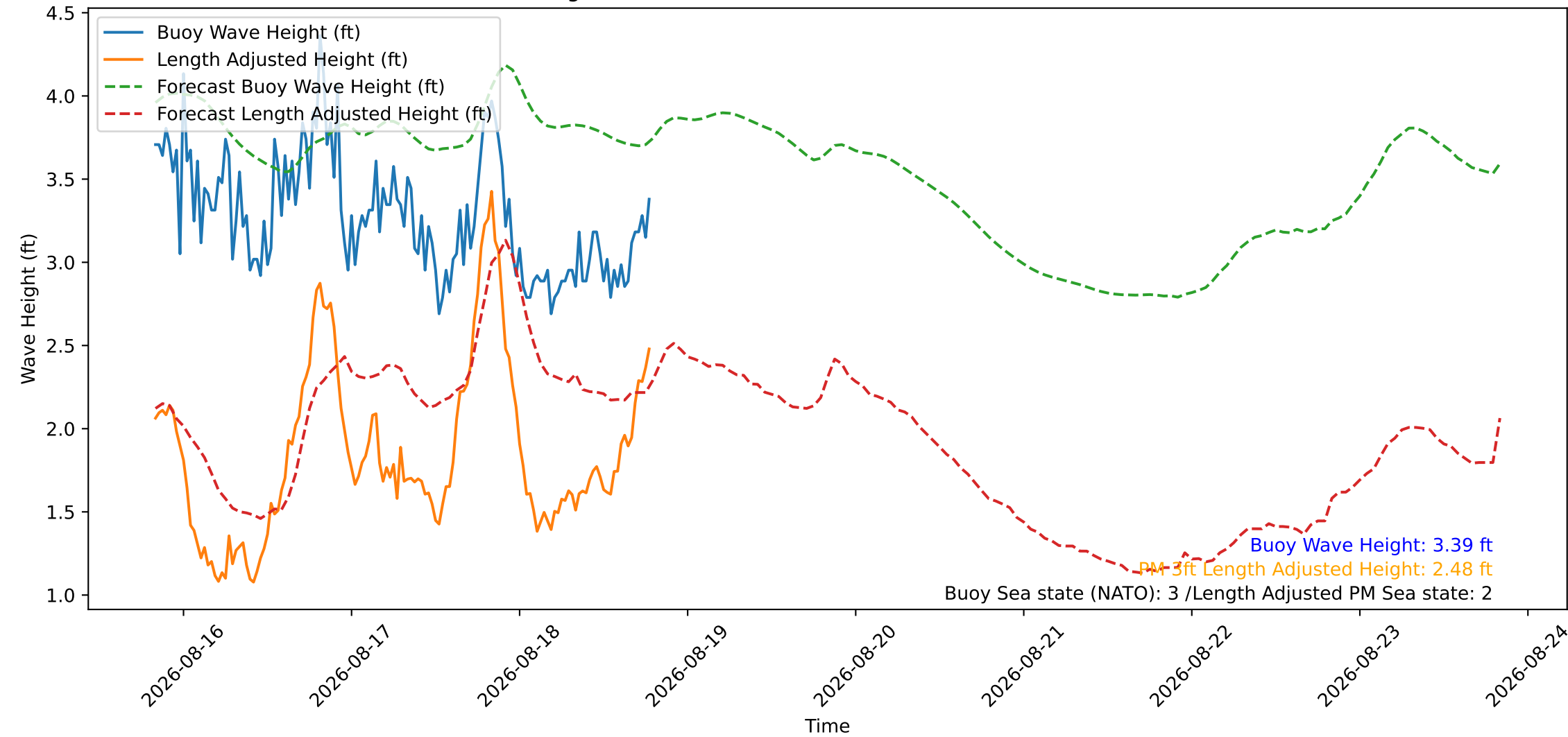
Wave Heights over Time for Green Beach at 2026-08-18 19:41:09
