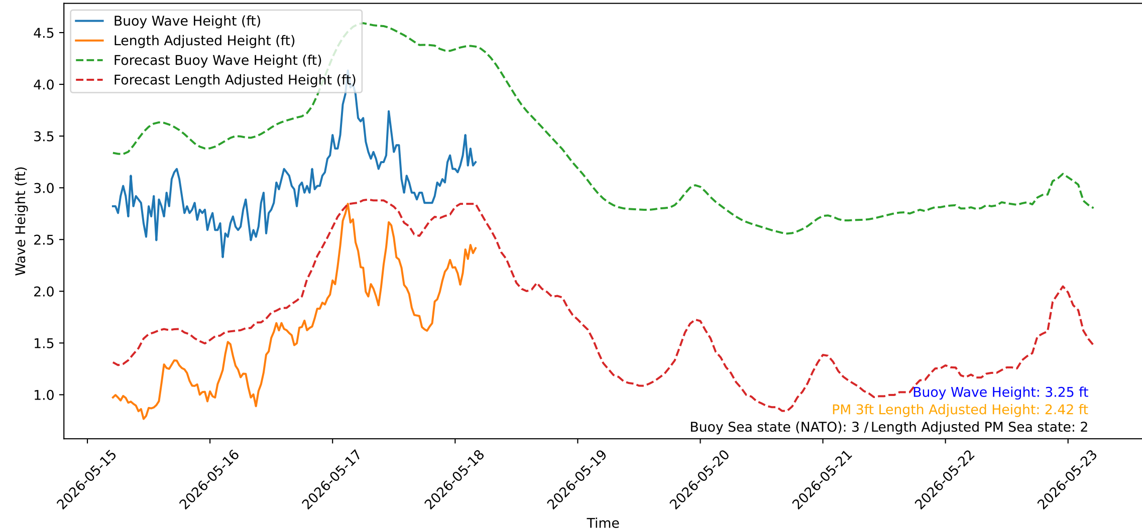
Wave Heights over Time for Red Beach at 2026-05-18 04:40:51
