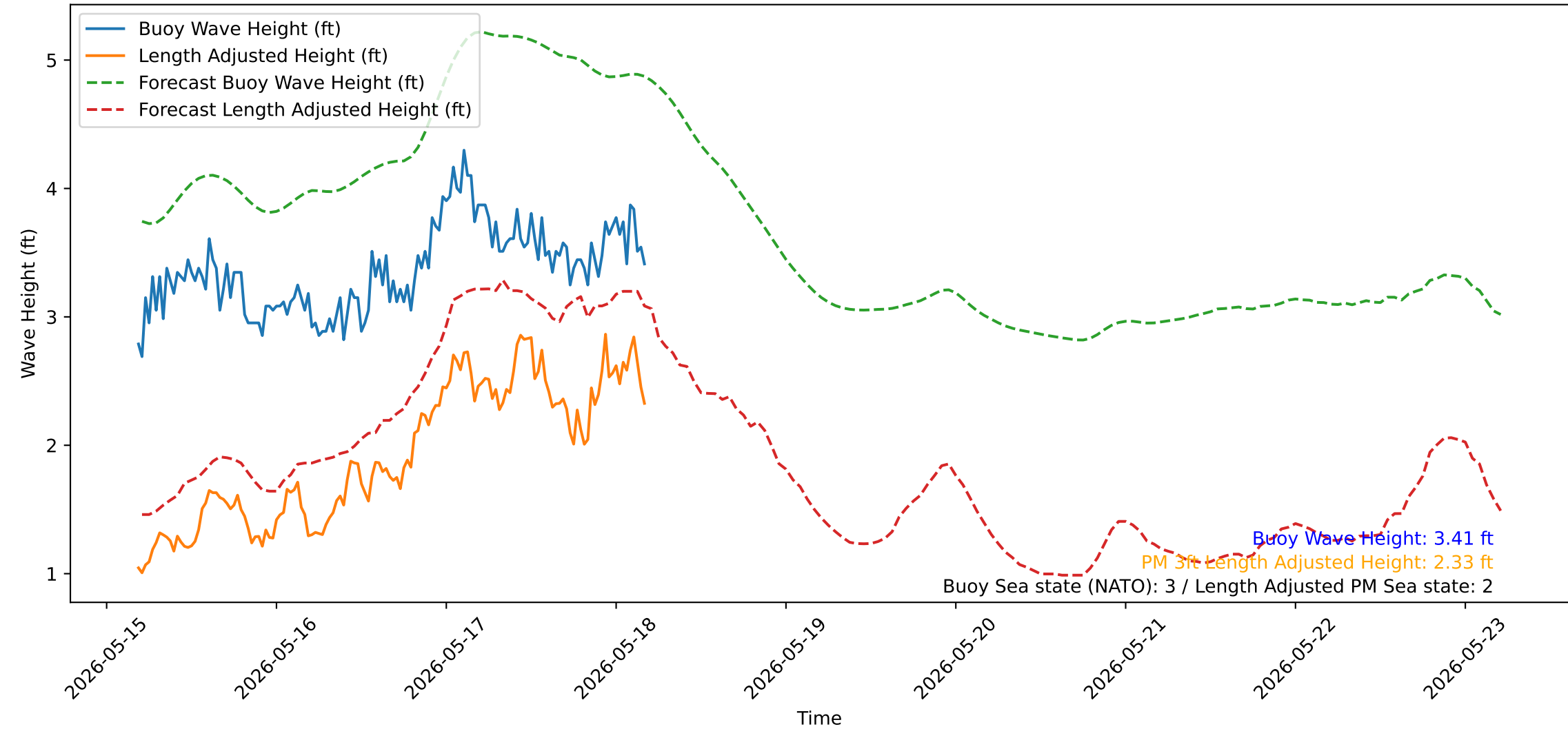
Wave Heights over Time for Oceanside Harbor at 2026-05-18 04:40:32
