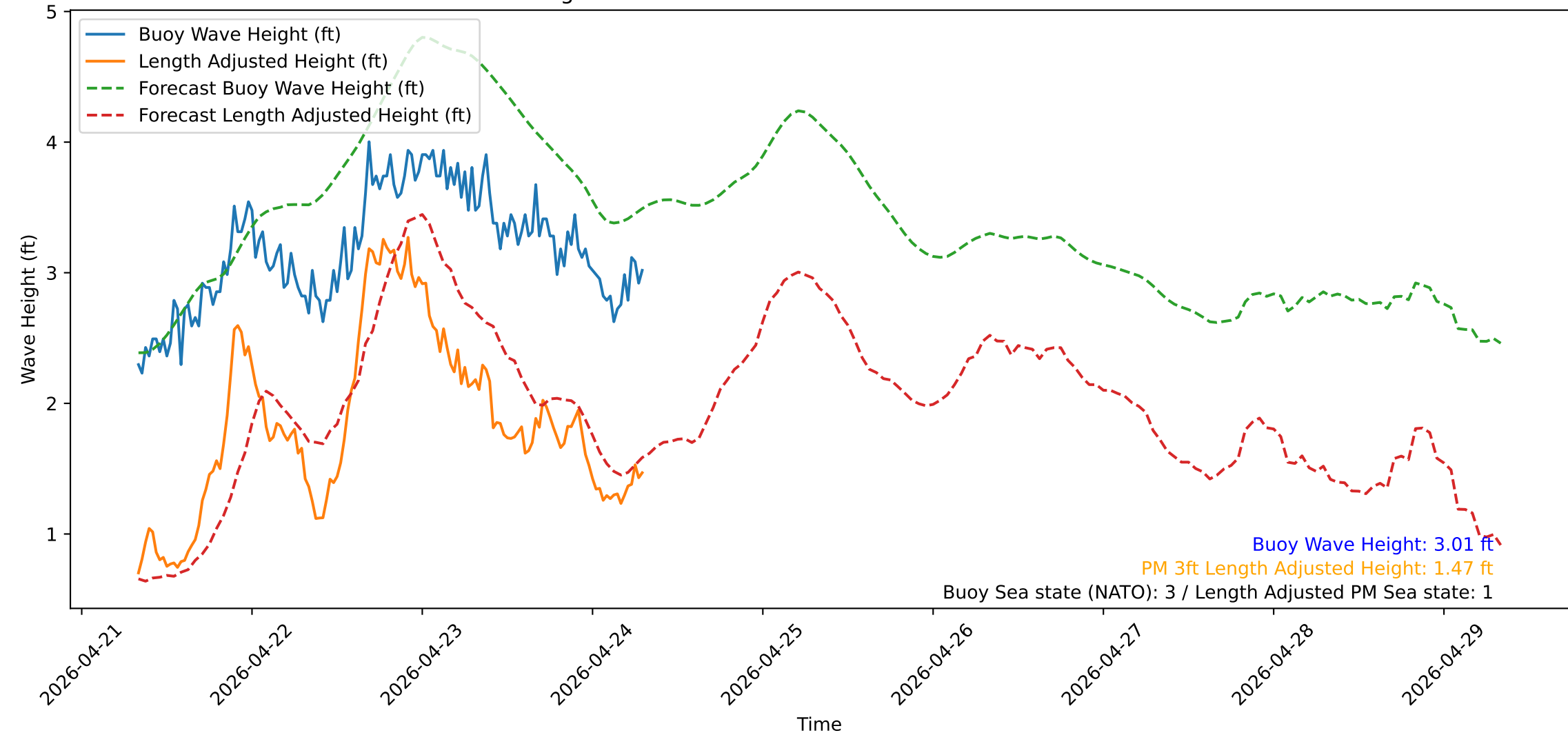
Wave Heights over Time for Green Beach at 2026-04-24 07:51:12
