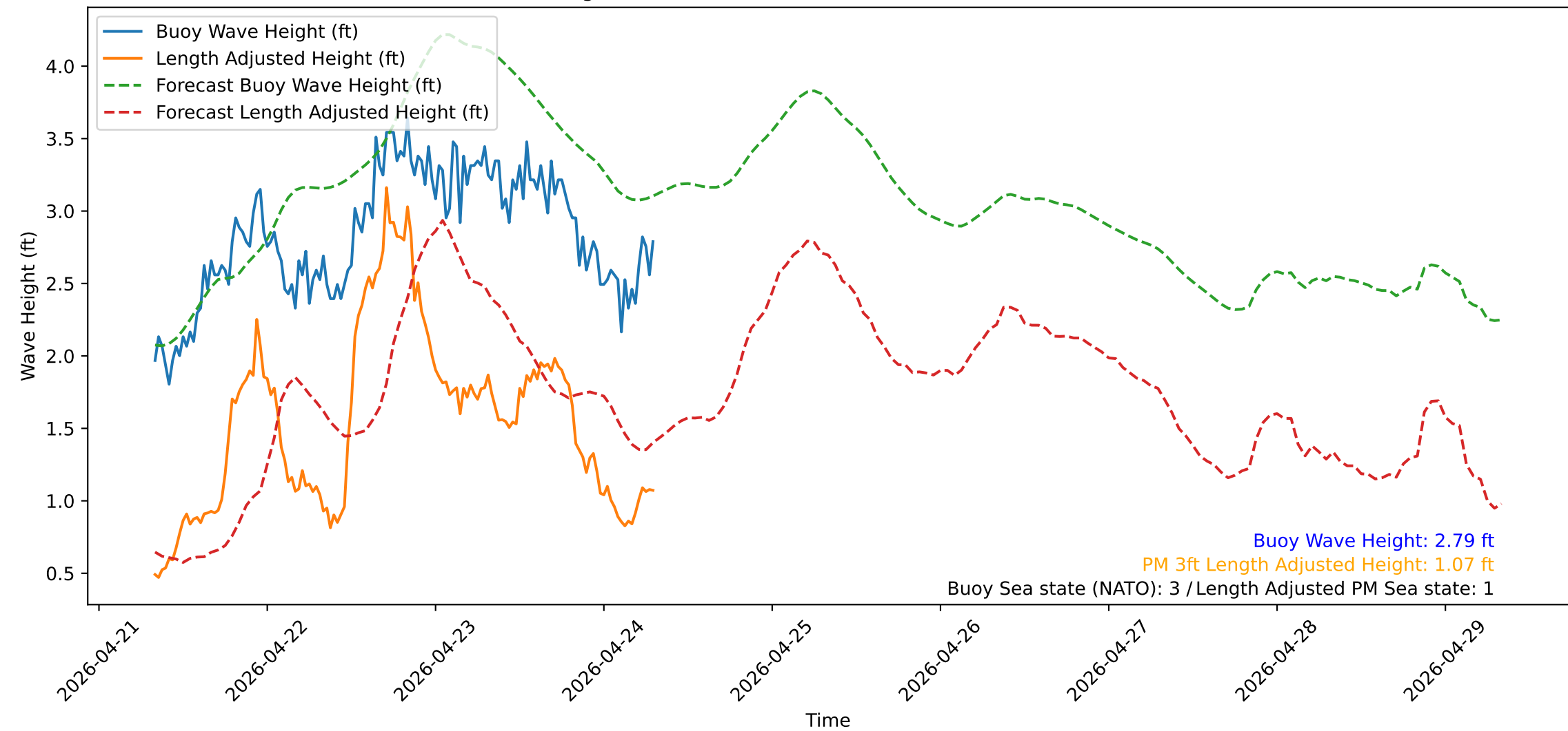
Wave Heights over Time for Red Beach at 2026-04-24 07:50:51
