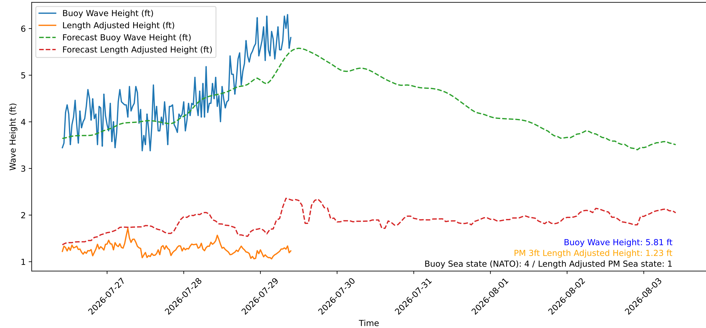
Wave Heights over Time for Green Beach at 2026-07-29 10:11:08
