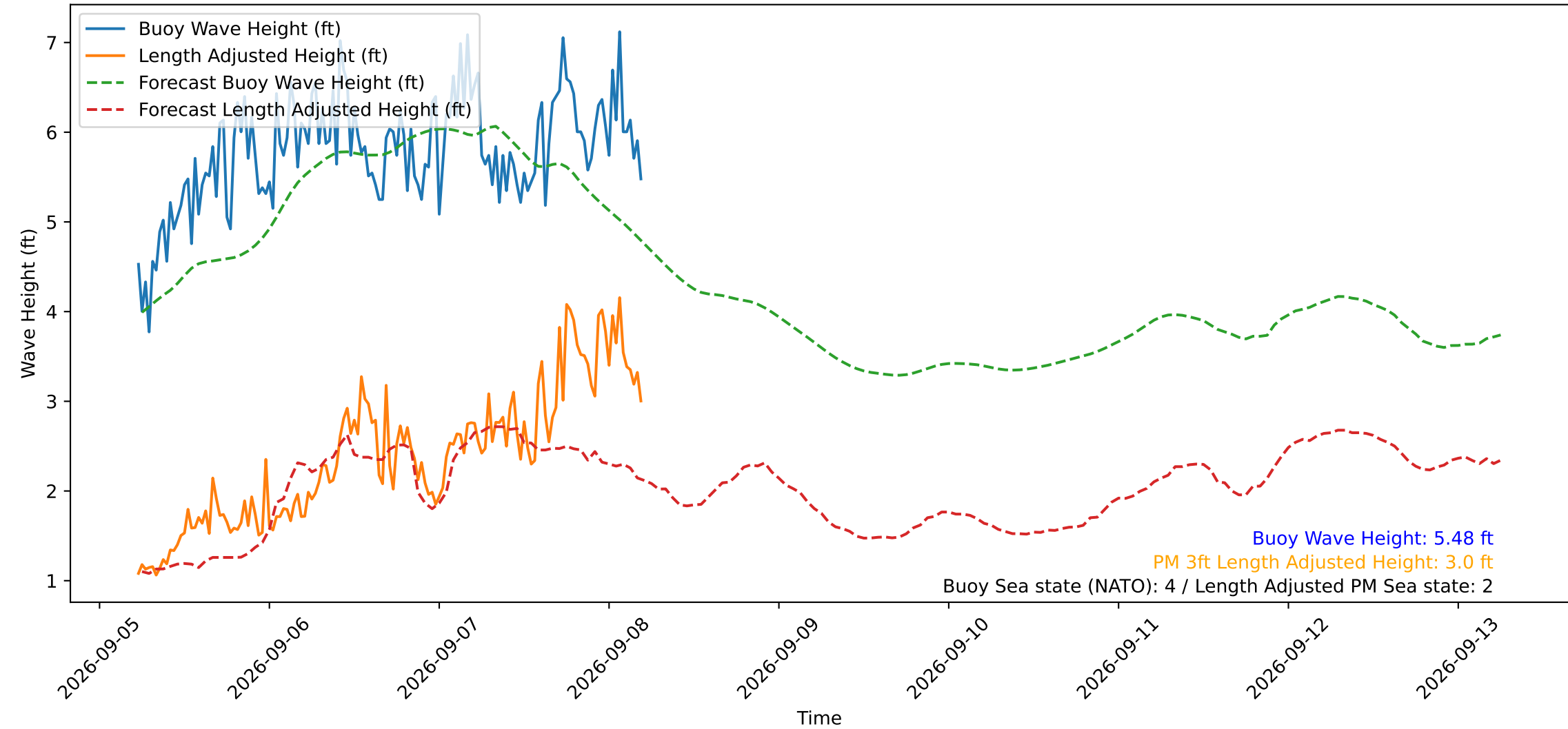
Wave Heights over Time for Oceanside Harbor at 2026-09-08 05:30:30
