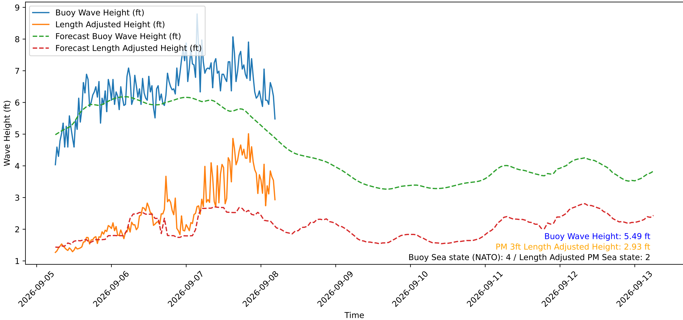
Wave Heights over Time for Green Beach at 2026-09-08 05:31:11
