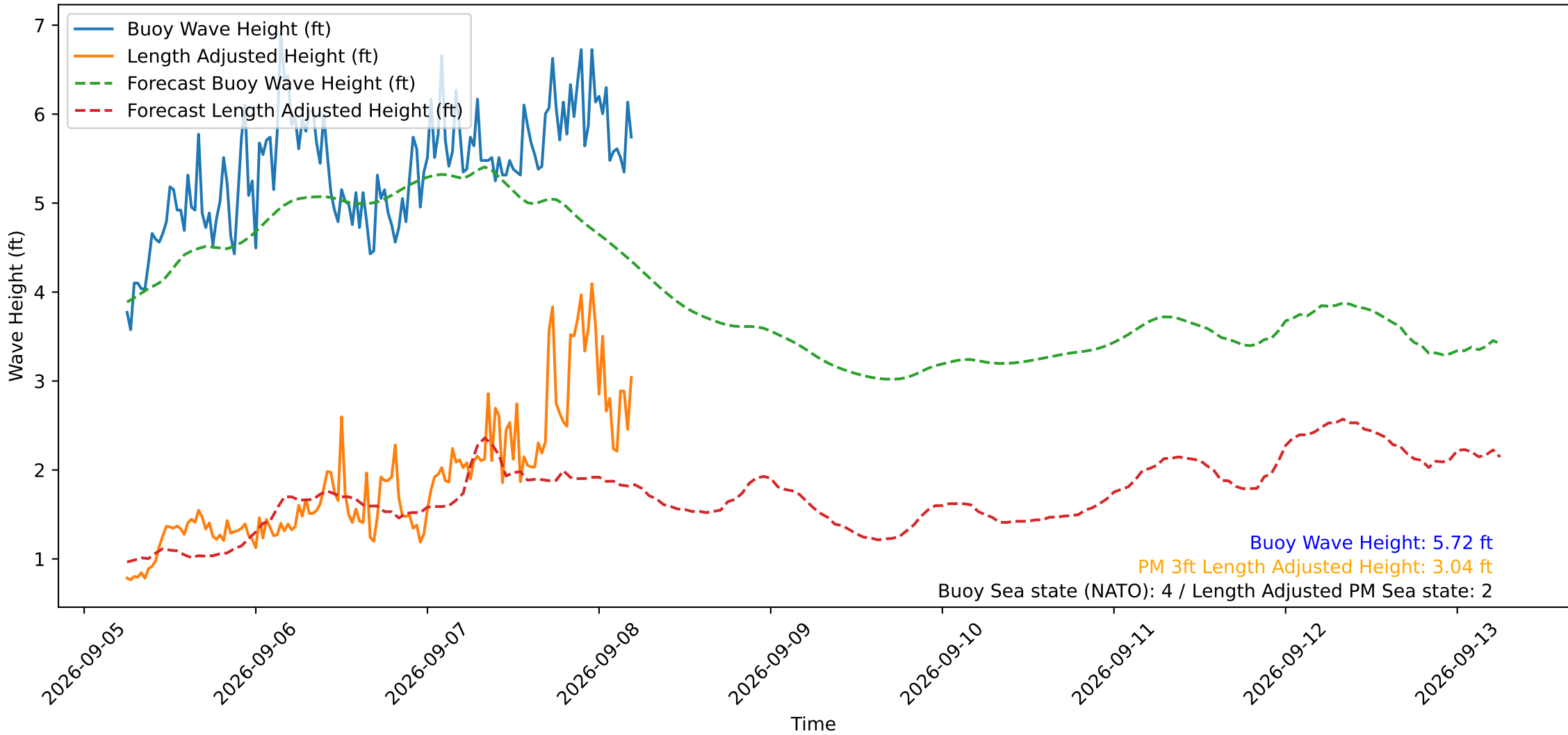
Wave Heights over Time for Red Beach at 2026-09-08 05:30:49
