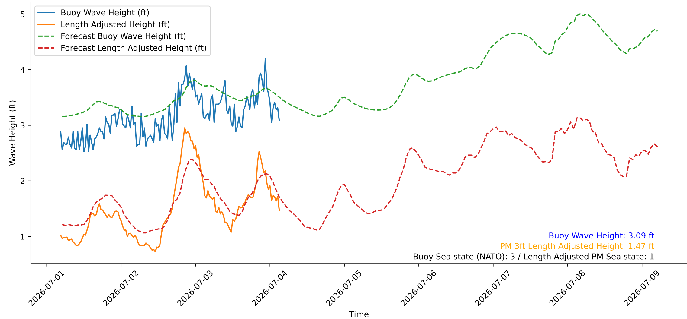
Wave Heights over Time for Green Beach at 2026-07-04 04:31:09
