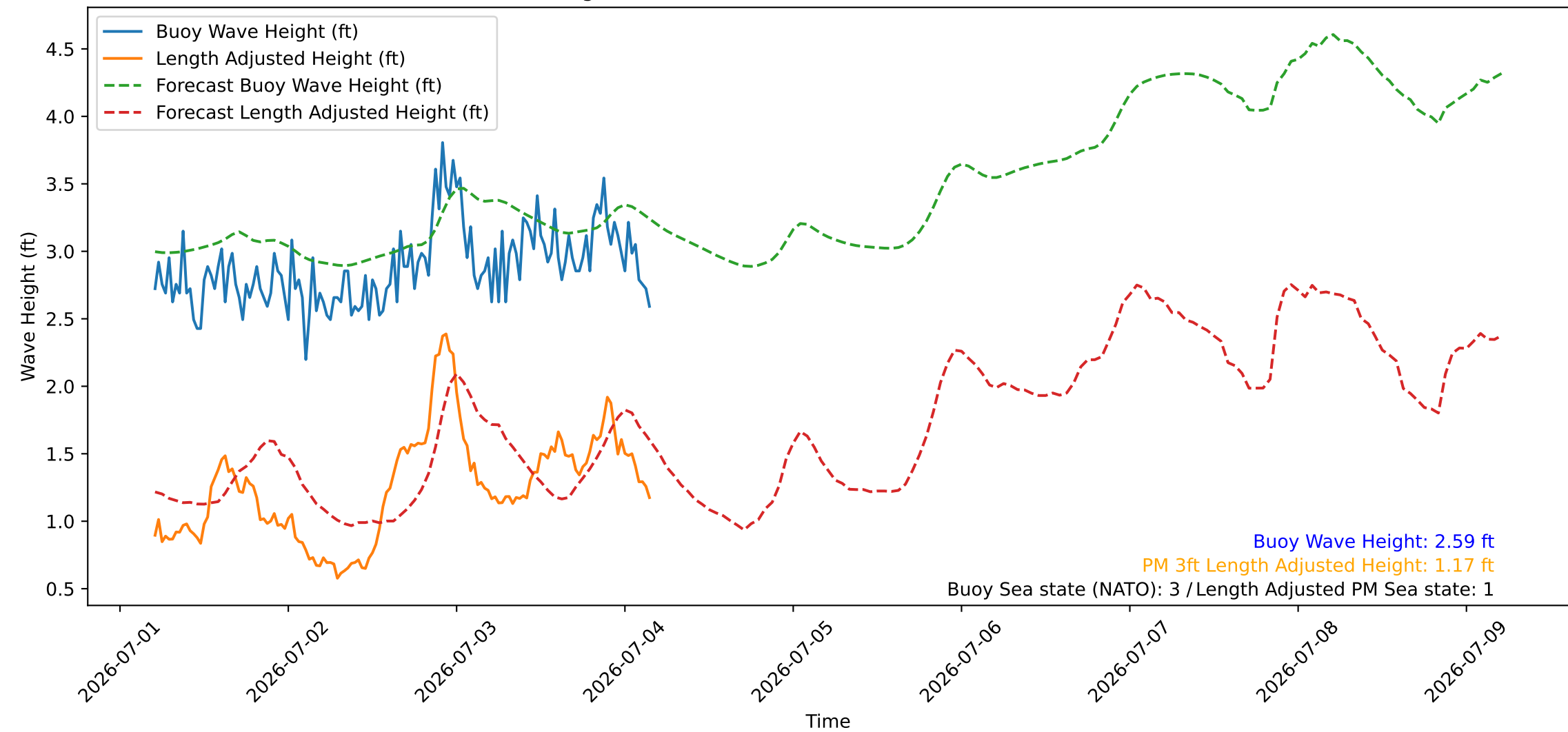
Wave Heights over Time for Red Beach at 2026-07-04 04:30:46
