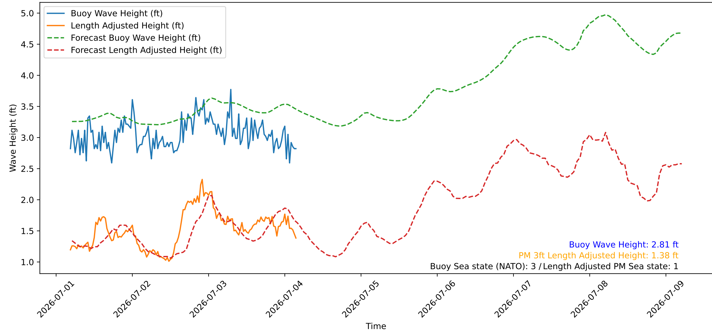
Wave Heights over Time for Oceanside Harbor at 2026-07-04 04:30:26
