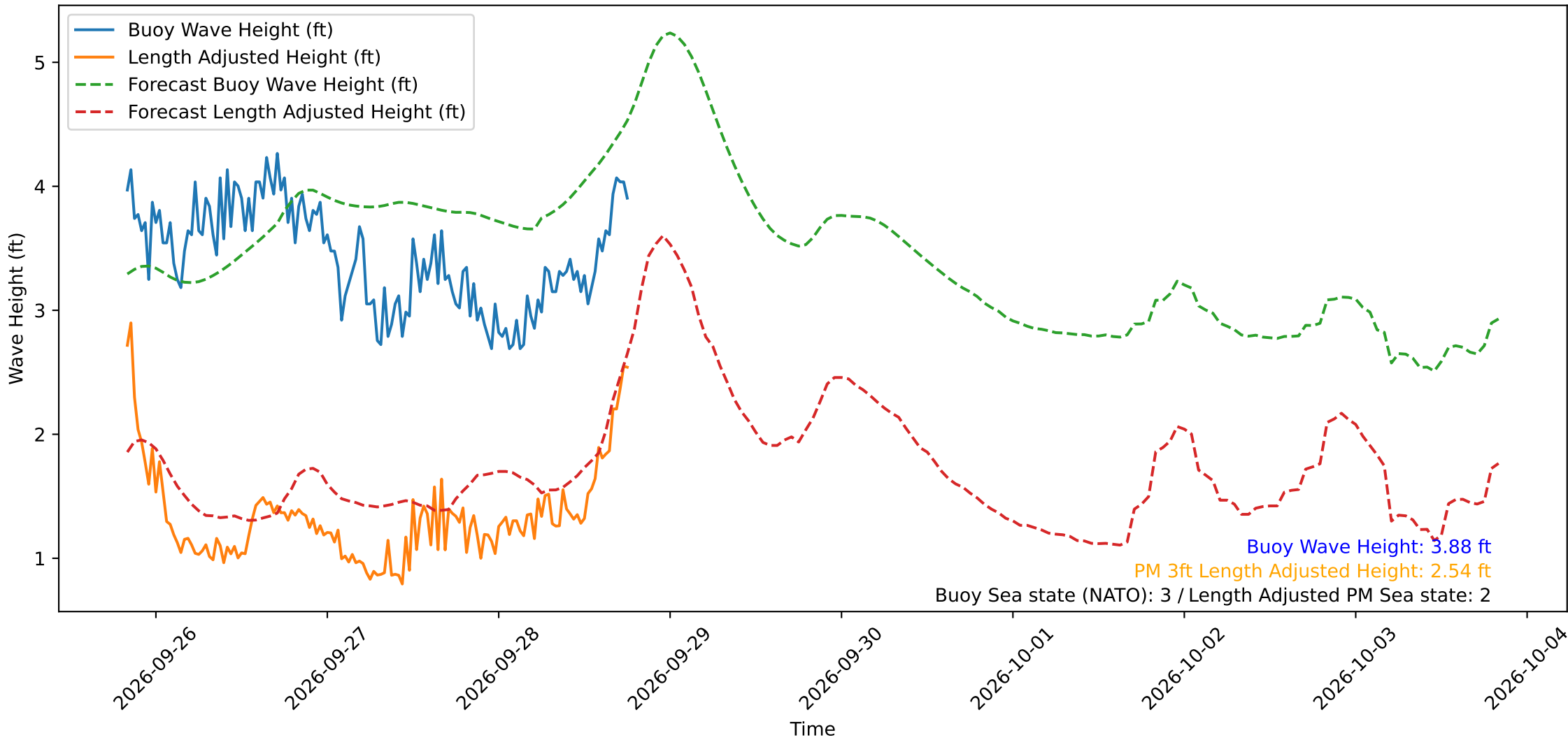
Wave Heights over Time for Green Beach at 2026-09-28 19:31:13
