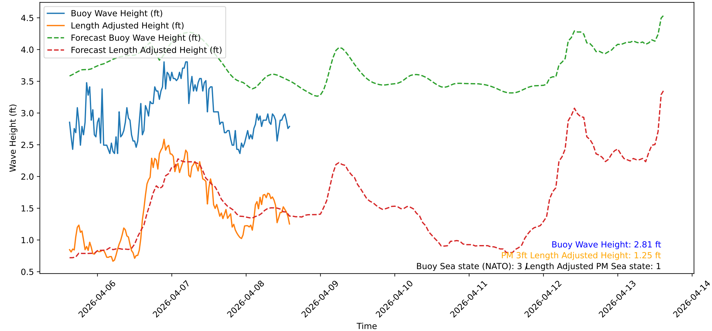
Wave Heights over Time for Green Beach at 2026-04-08 14:51:10
