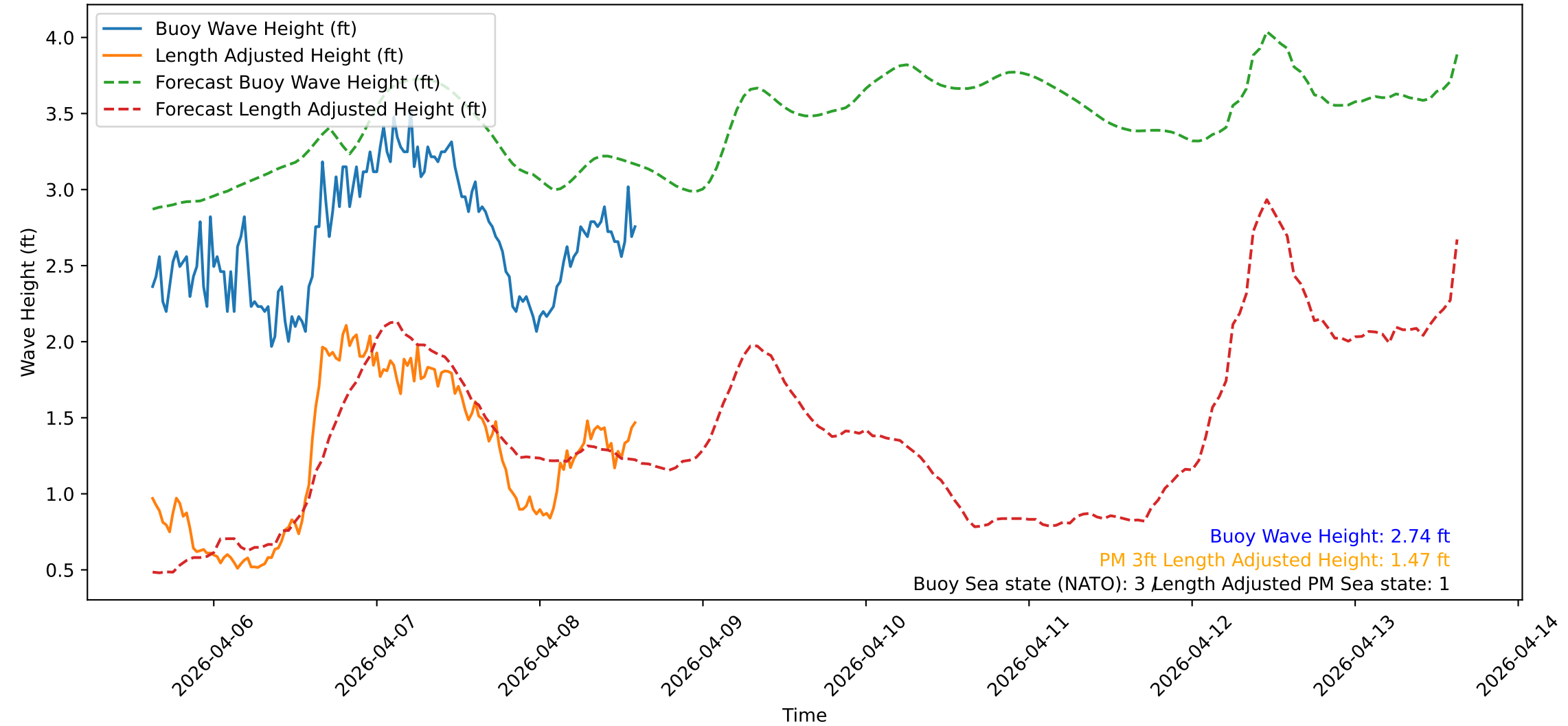
Wave Heights over Time for Red Beach at 2026-04-08 14:50:47
