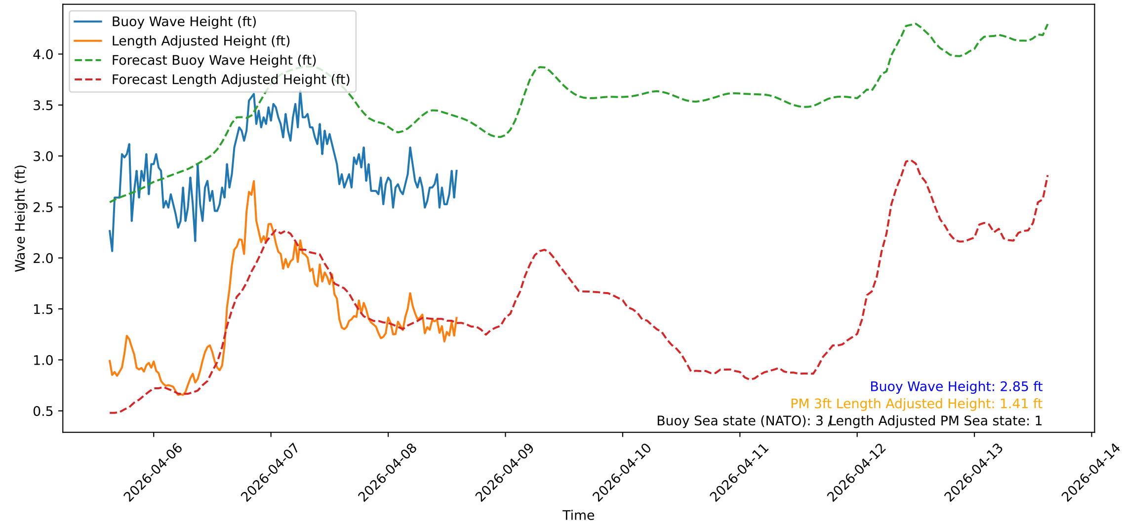
Wave Heights over Time for Oceanside Harbor at 2026-04-08 14:50:31
