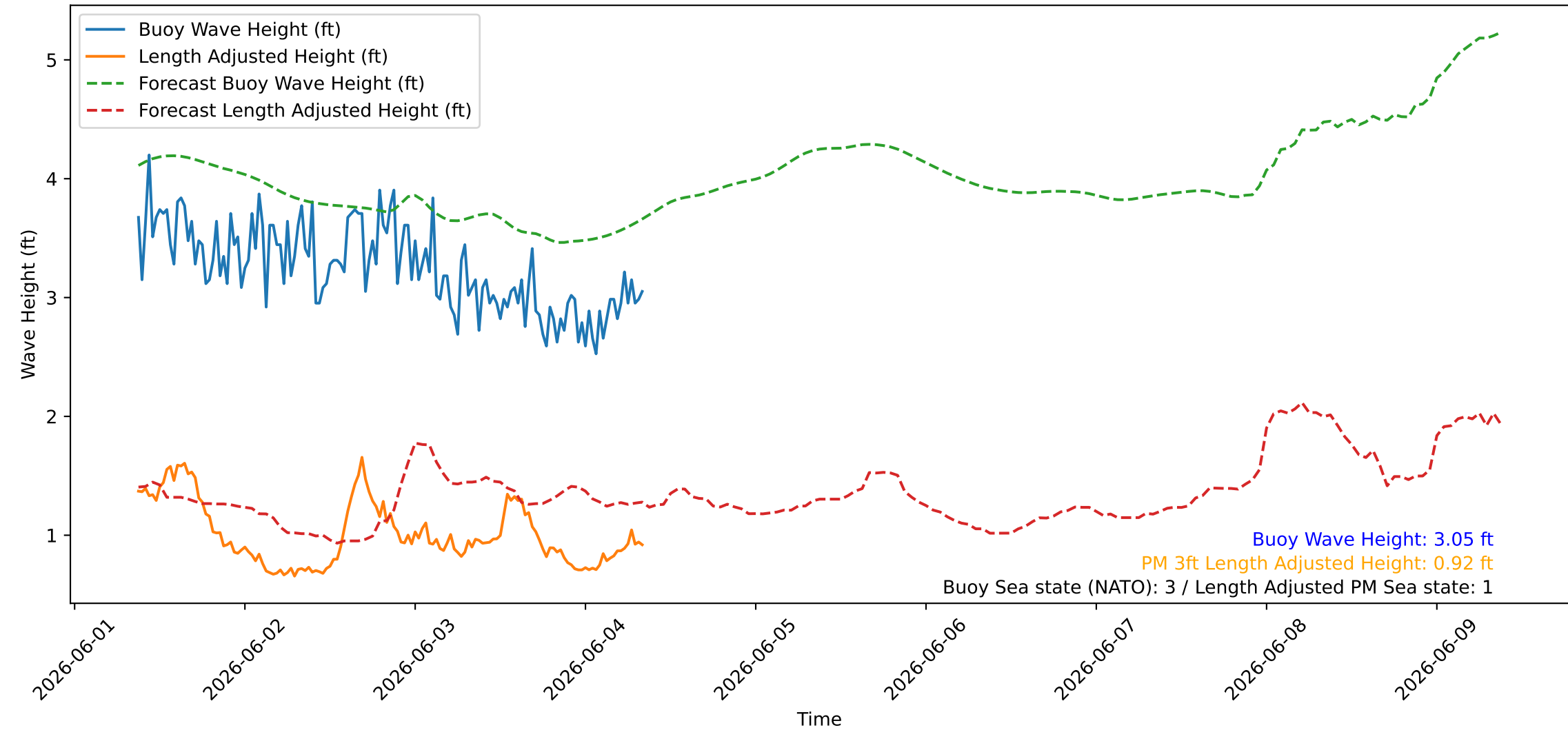
Wave Heights over Time for Red Beach at 2026-06-04 08:40:46
