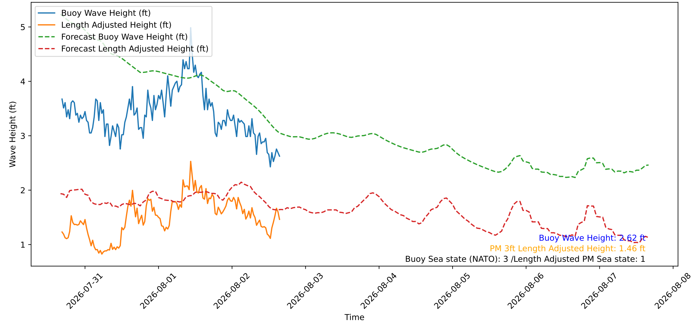
Wave Heights over Time for Green Beach at 2026-08-02 16:21:10
