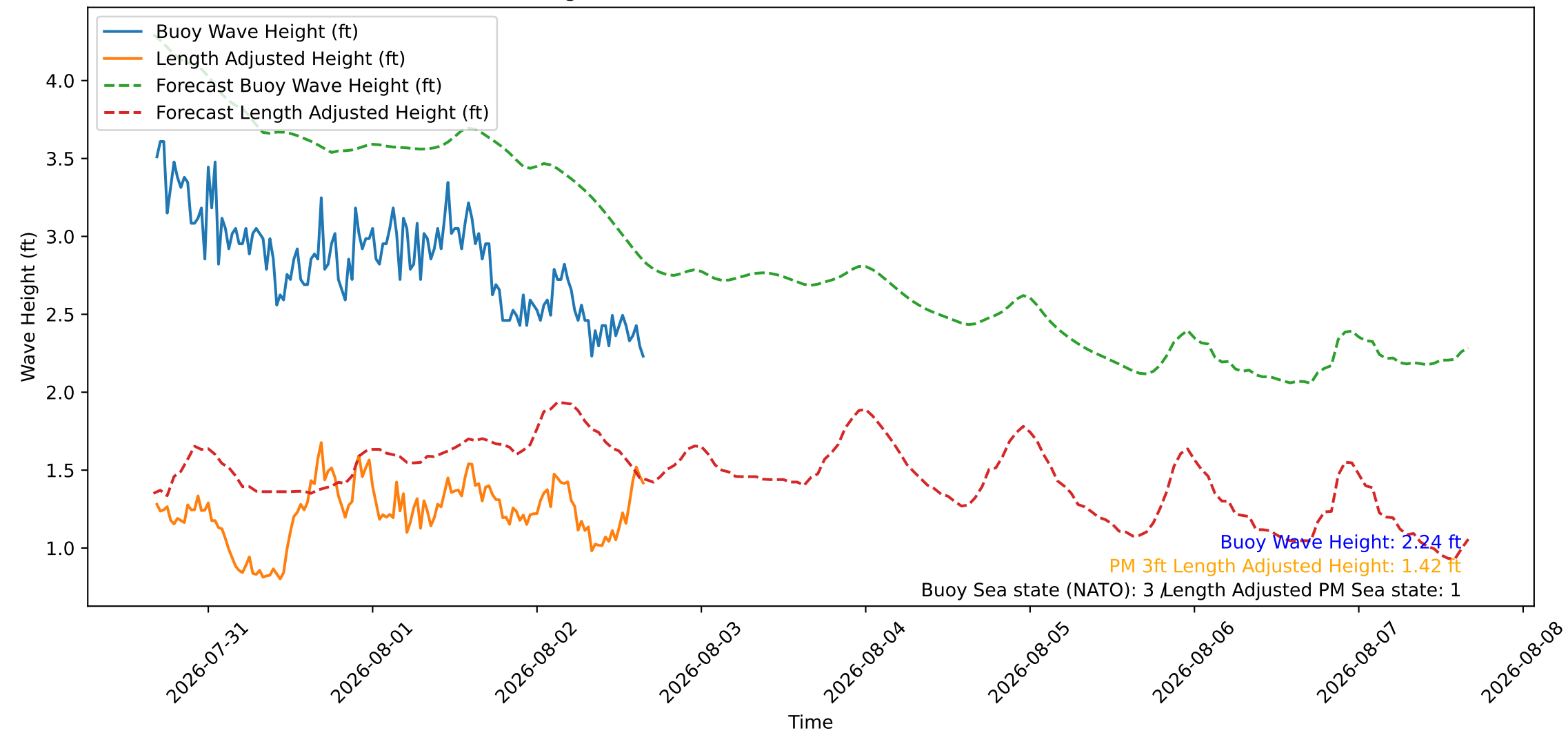
Wave Heights over Time for Red Beach at 2026-08-02 16:20:48
