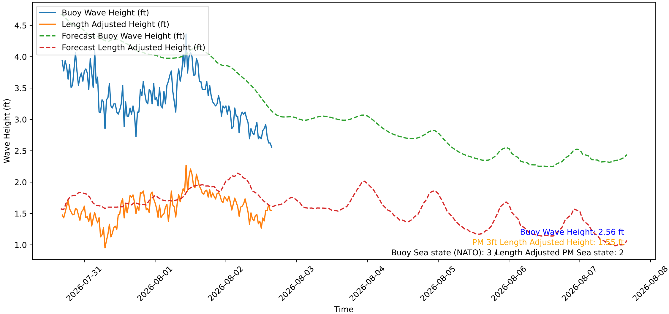
Wave Heights over Time for Oceanside Harbor at 2026-08-02 16:20:27
