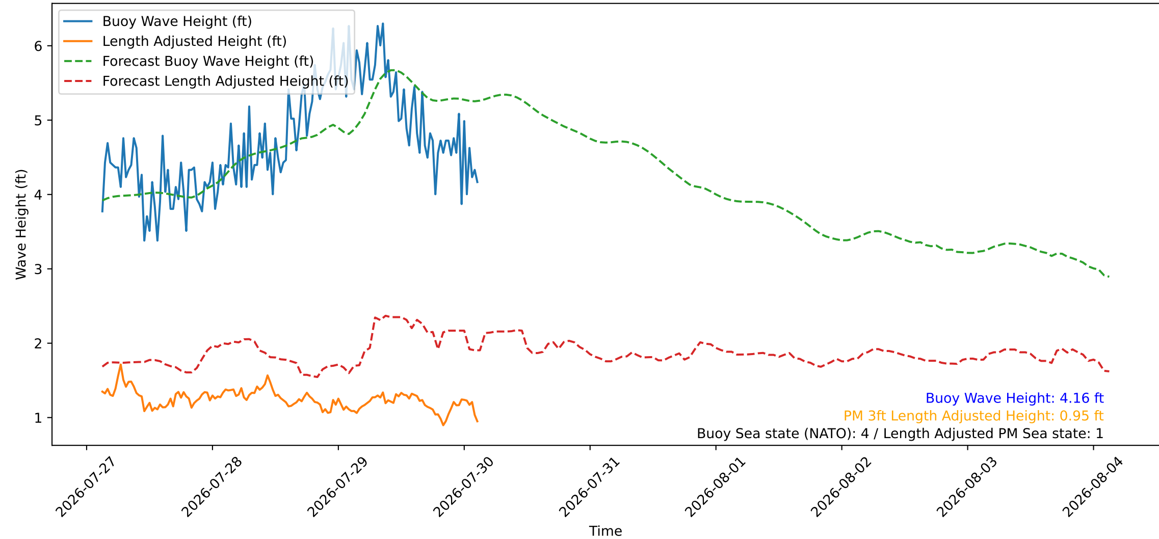
Wave Heights over Time for Green Beach at 2026-07-30 03:11:09
