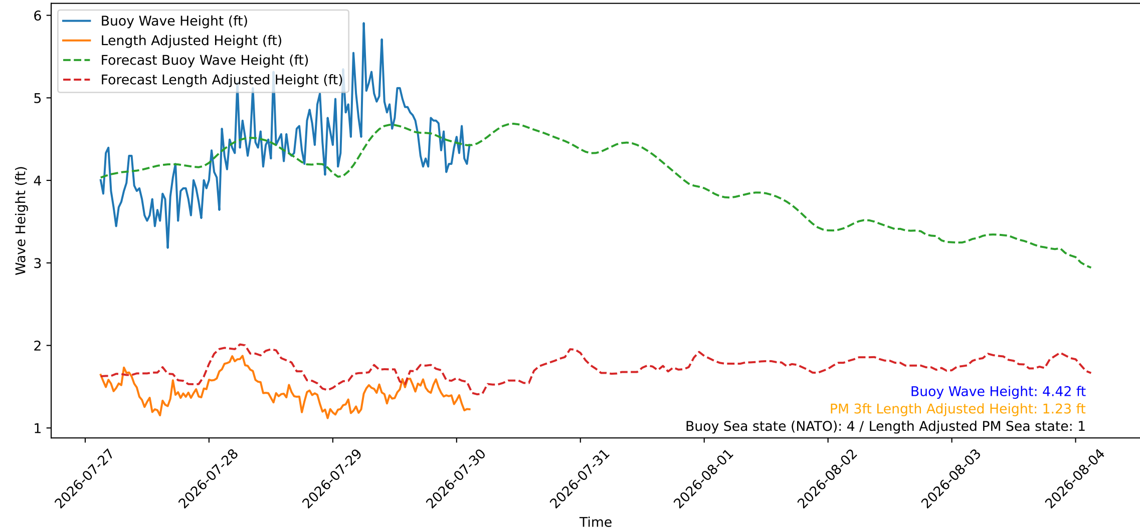
Wave Heights over Time for Oceanside Harbor at 2026-07-30 03:10:26
