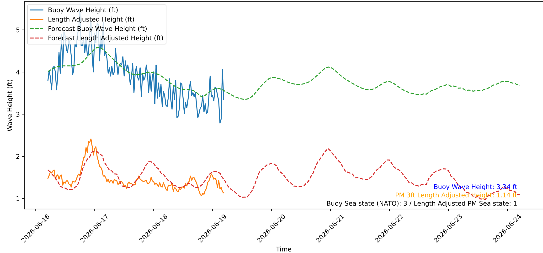
Wave Heights over Time for Oceanside Harbor at 2026-06-19 05:00:25
