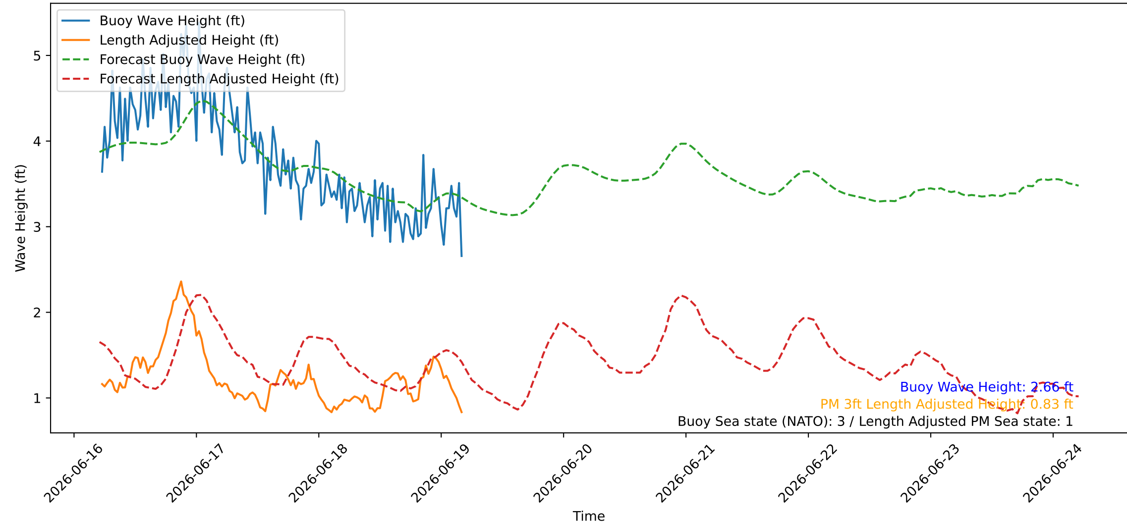
Wave Heights over Time for Red Beach at 2026-06-19 05:00:45
