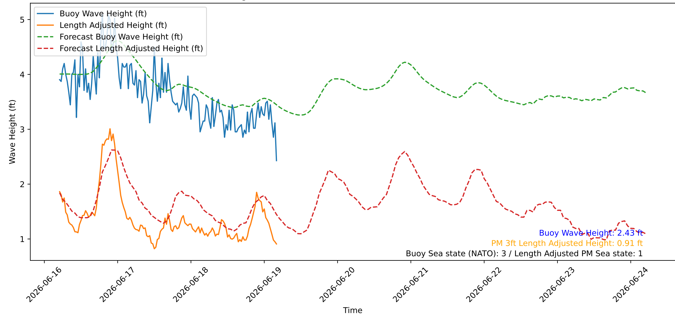
Wave Heights over Time for Green Beach at 2026-06-19 05:01:07
