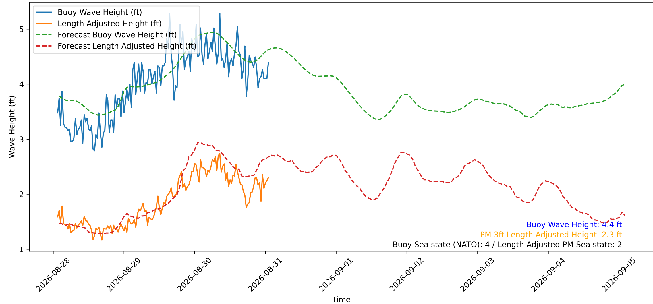
Wave Heights over Time for Oceanside Harbor at 2026-08-31 01:30:29
