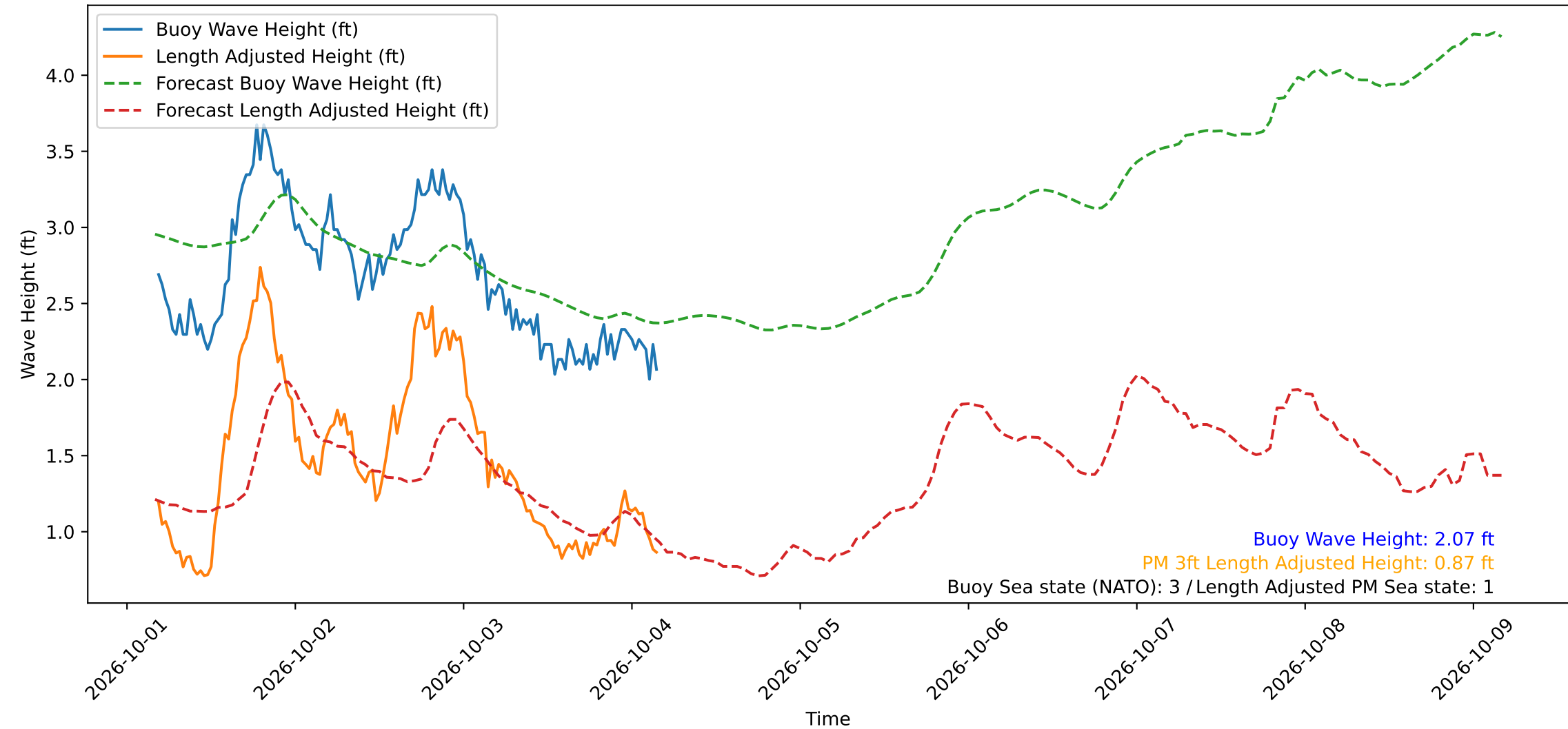
Wave Heights over Time for Green Beach at 2026-10-04 04:21:14
