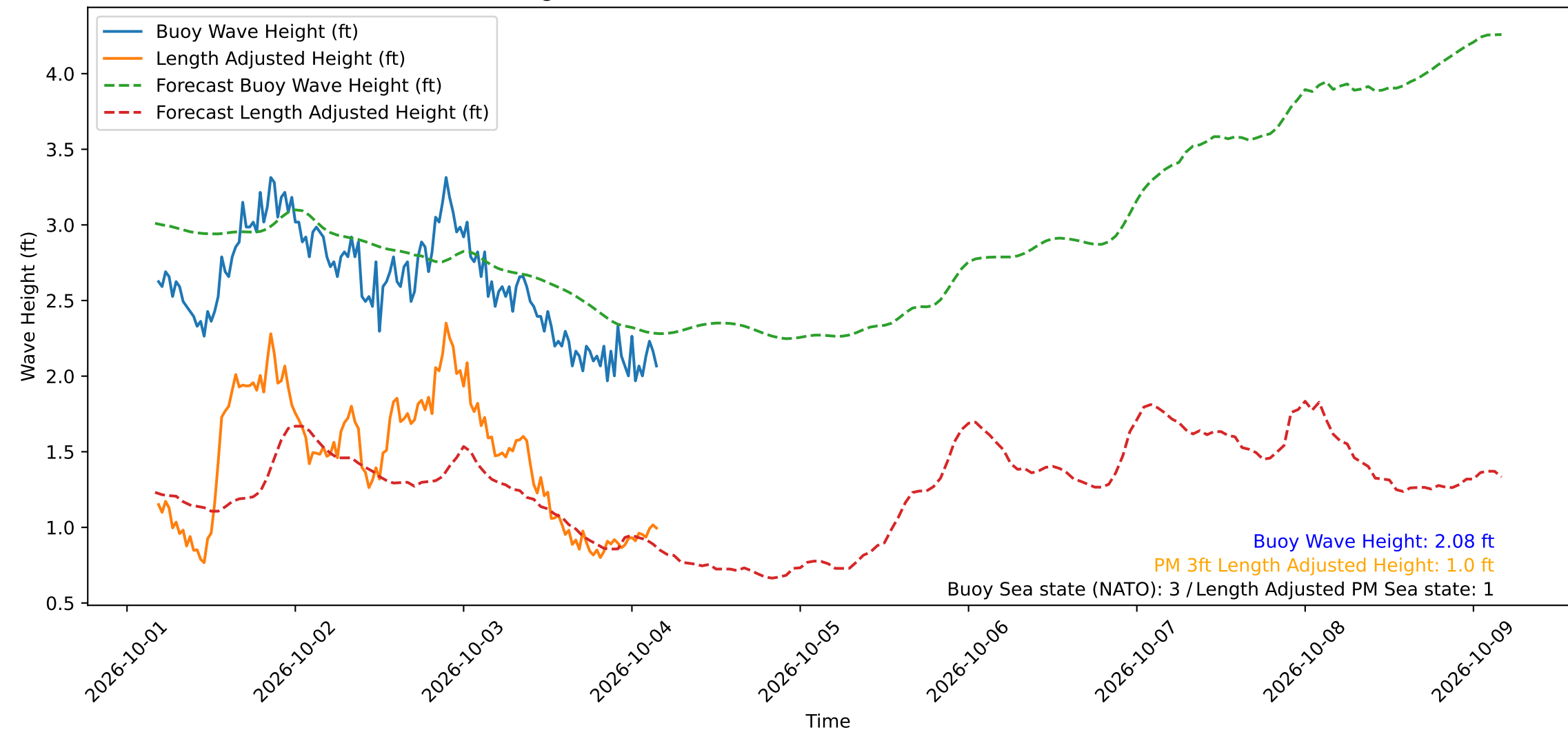
Wave Heights over Time for Oceanside Harbor at 2026-10-04 04:20:29
