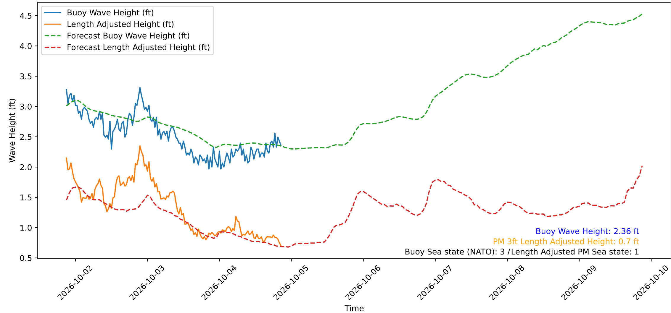
Wave Heights over Time for Oceanside Harbor at 2026-10-04 21:10:29
