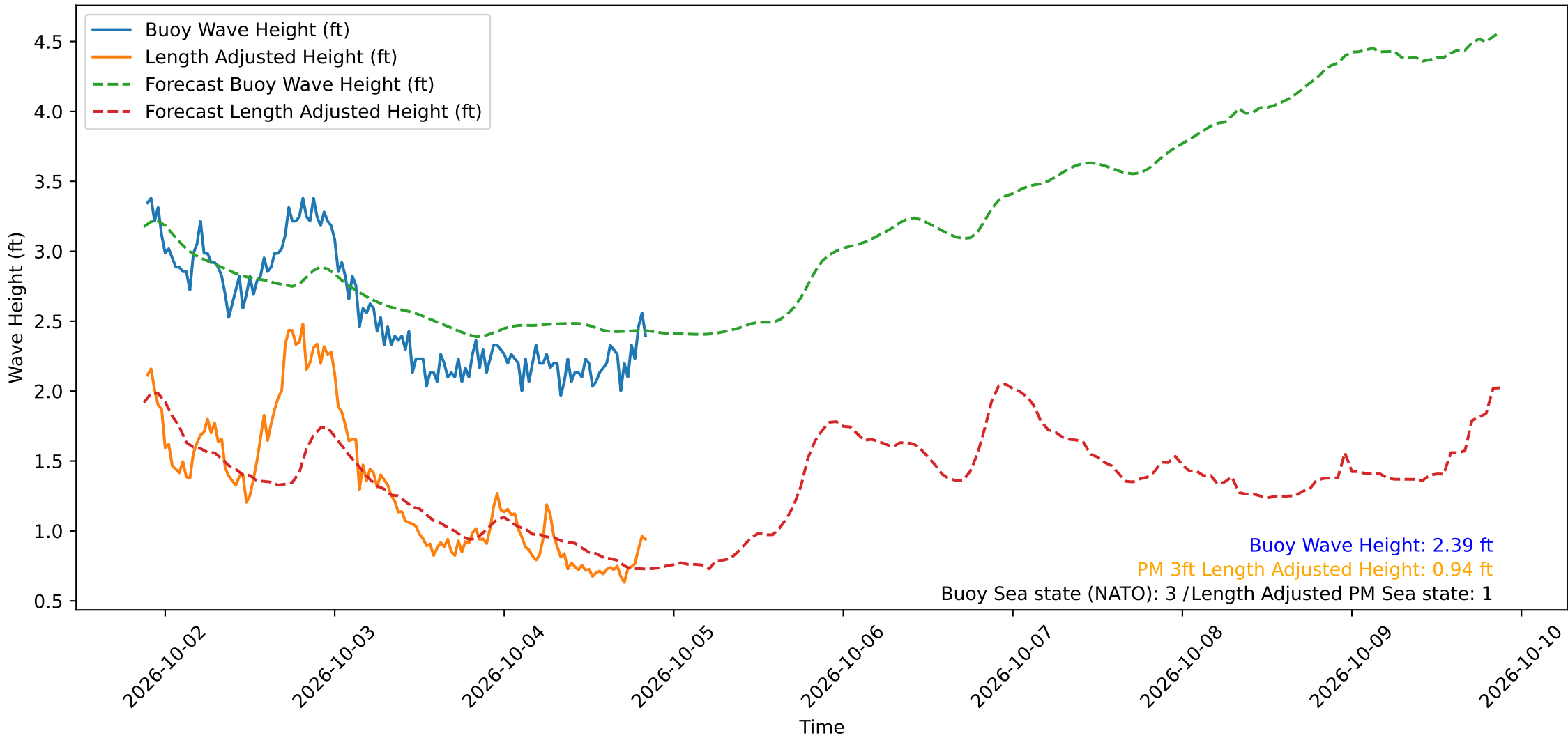
Wave Heights over Time for Green Beach at 2026-10-04 21:11:10
