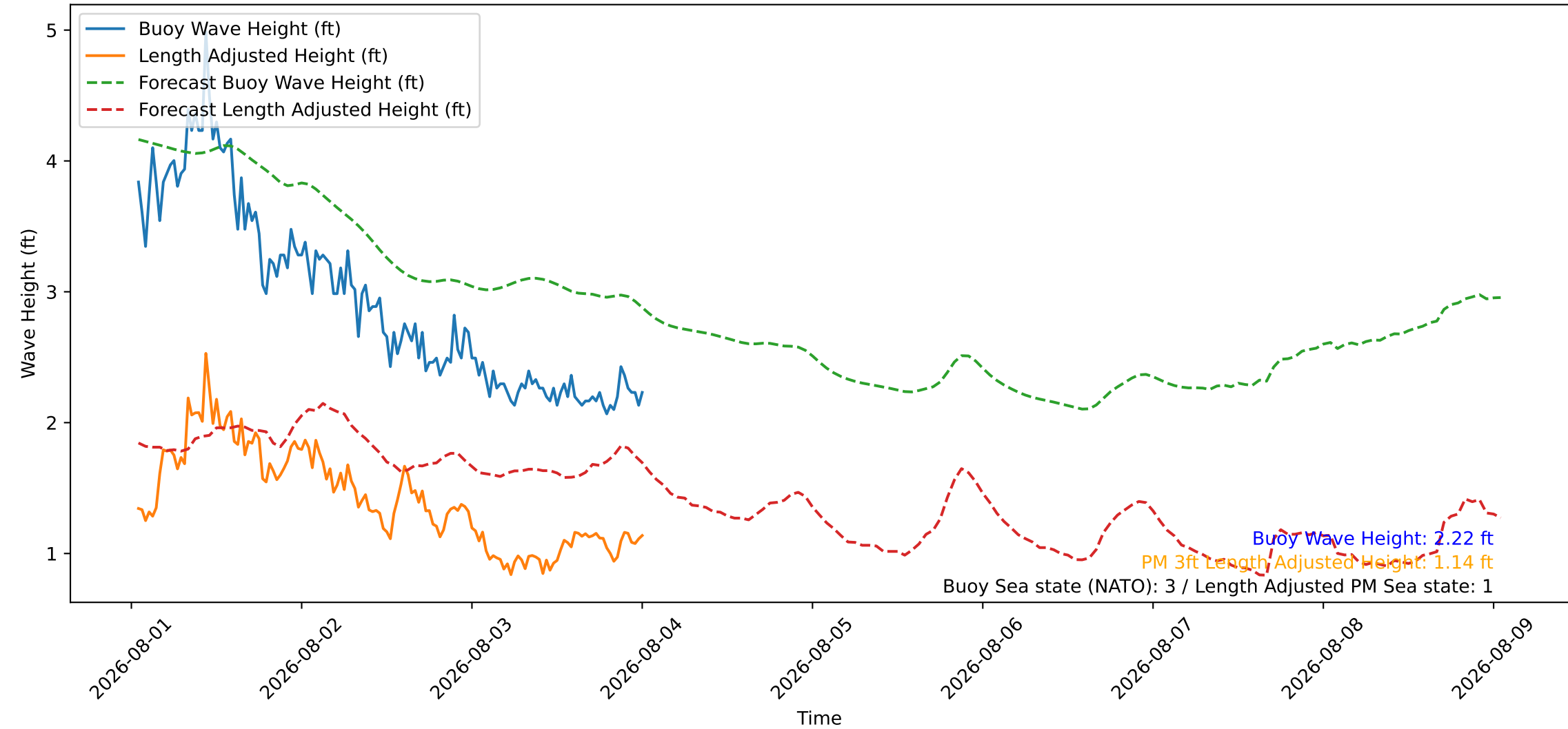
Wave Heights over Time for Green Beach at 2026-08-04 00:51:09
