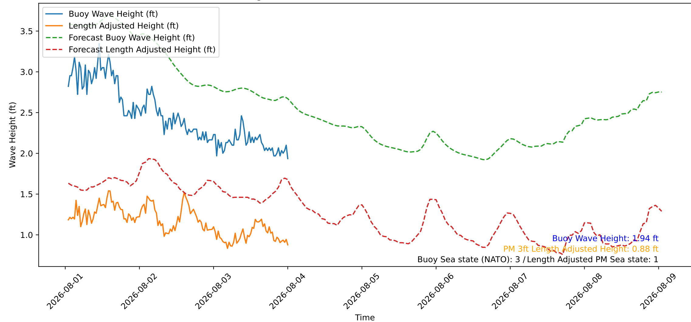
Wave Heights over Time for Red Beach at 2026-08-04 00:50:47
