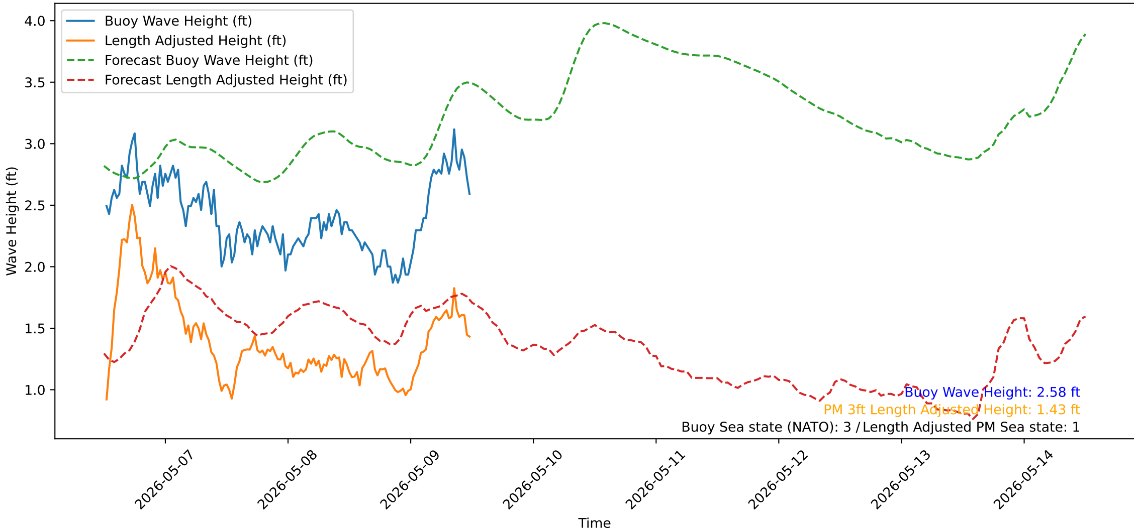
Wave Heights over Time for Oceanside Harbor at 2026-05-09 12:20:32
