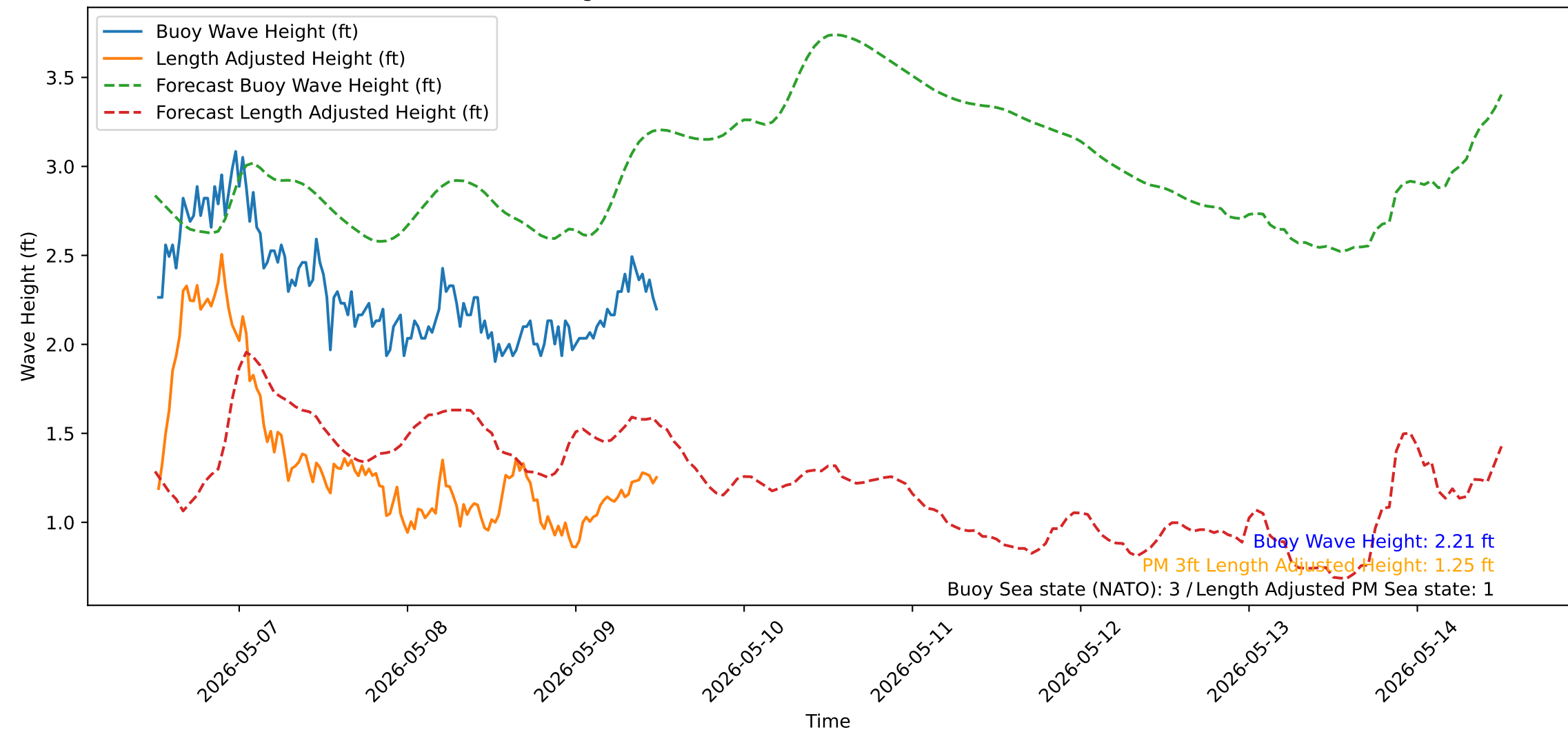
Wave Heights over Time for Red Beach at 2026-05-09 12:20:53
