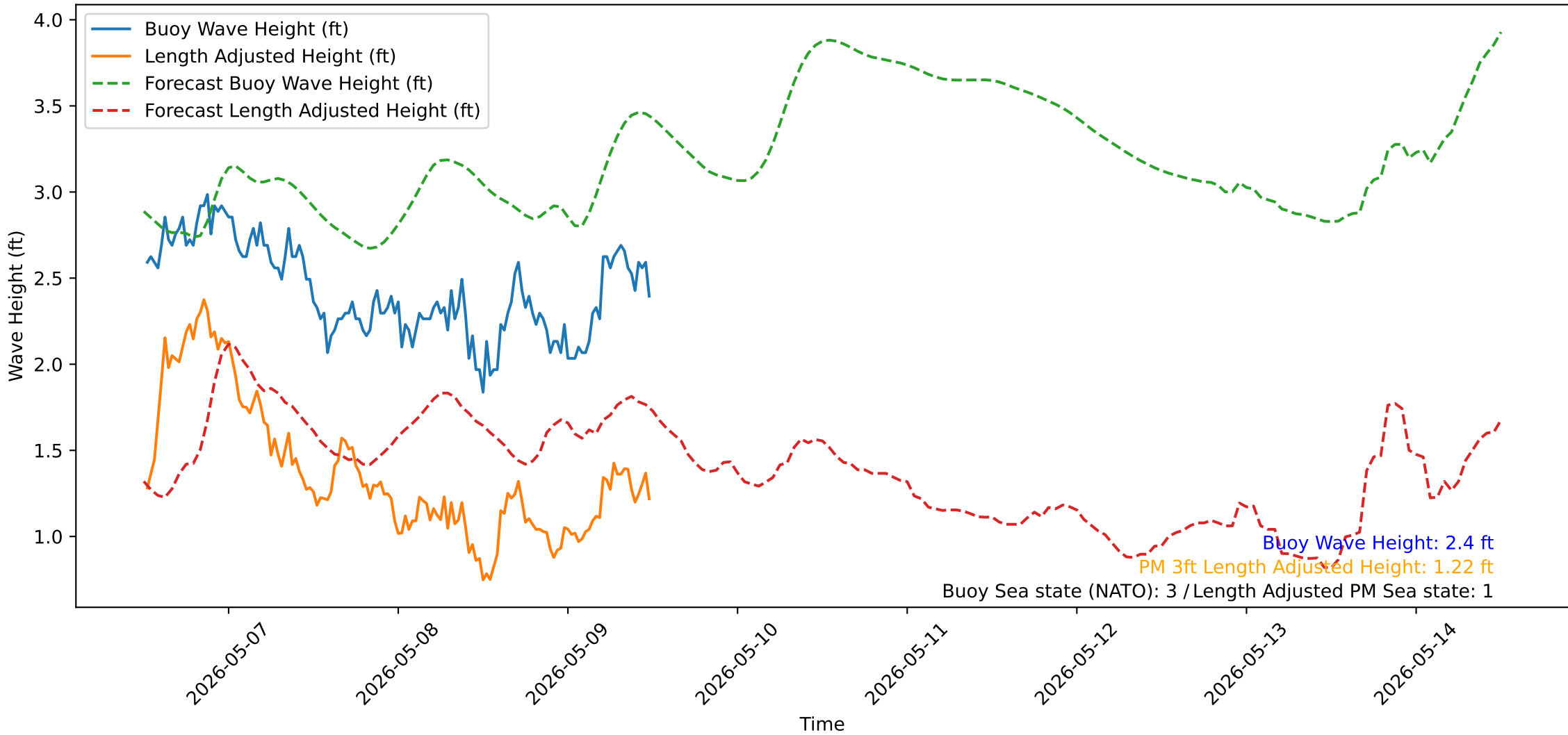
Wave Heights over Time for Green Beach at 2026-05-09 12:21:15
