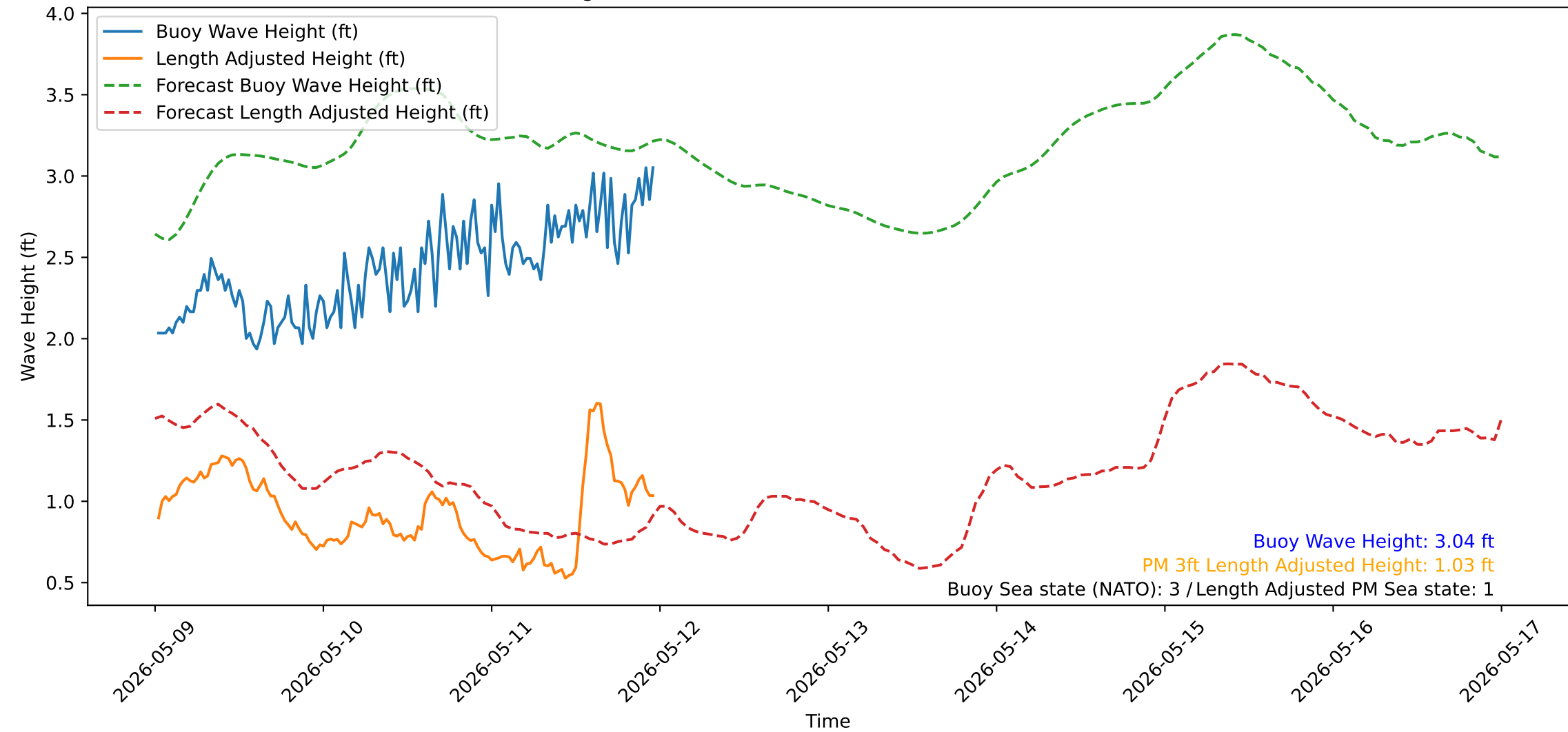
Wave Heights over Time for Red Beach at 2026-05-12 00:00:50
