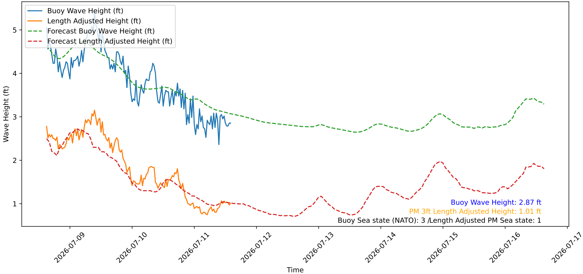
Wave Heights over Time for Oceanside Harbor at 2026-07-11 15:00:27
