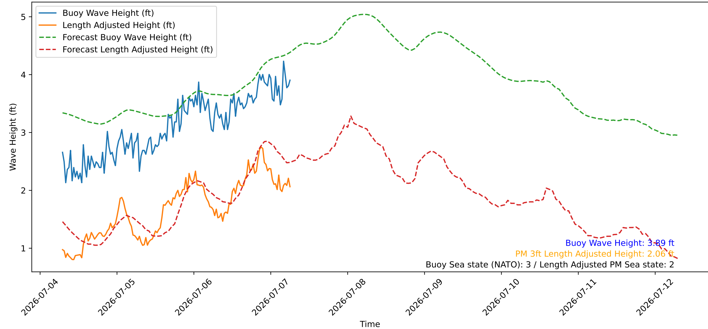
Wave Heights over Time for Oceanside Harbor at 2026-07-07 07:00:27
