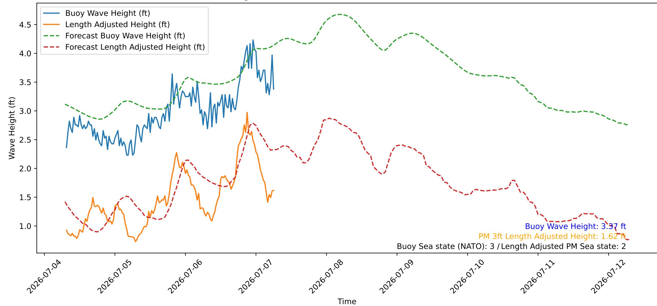
Wave Heights over Time for Red Beach at 2026-07-07 07:00:46
