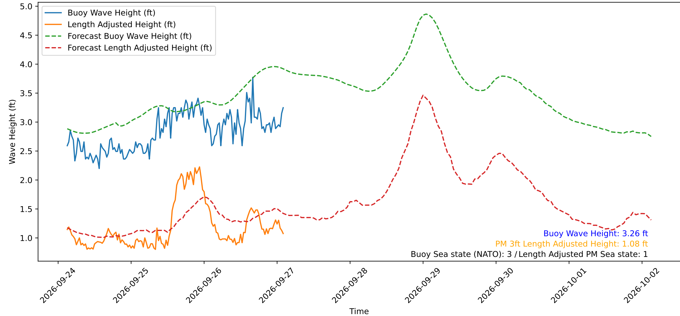
Wave Heights over Time for Oceanside Harbor at 2026-09-27 02:50:30
