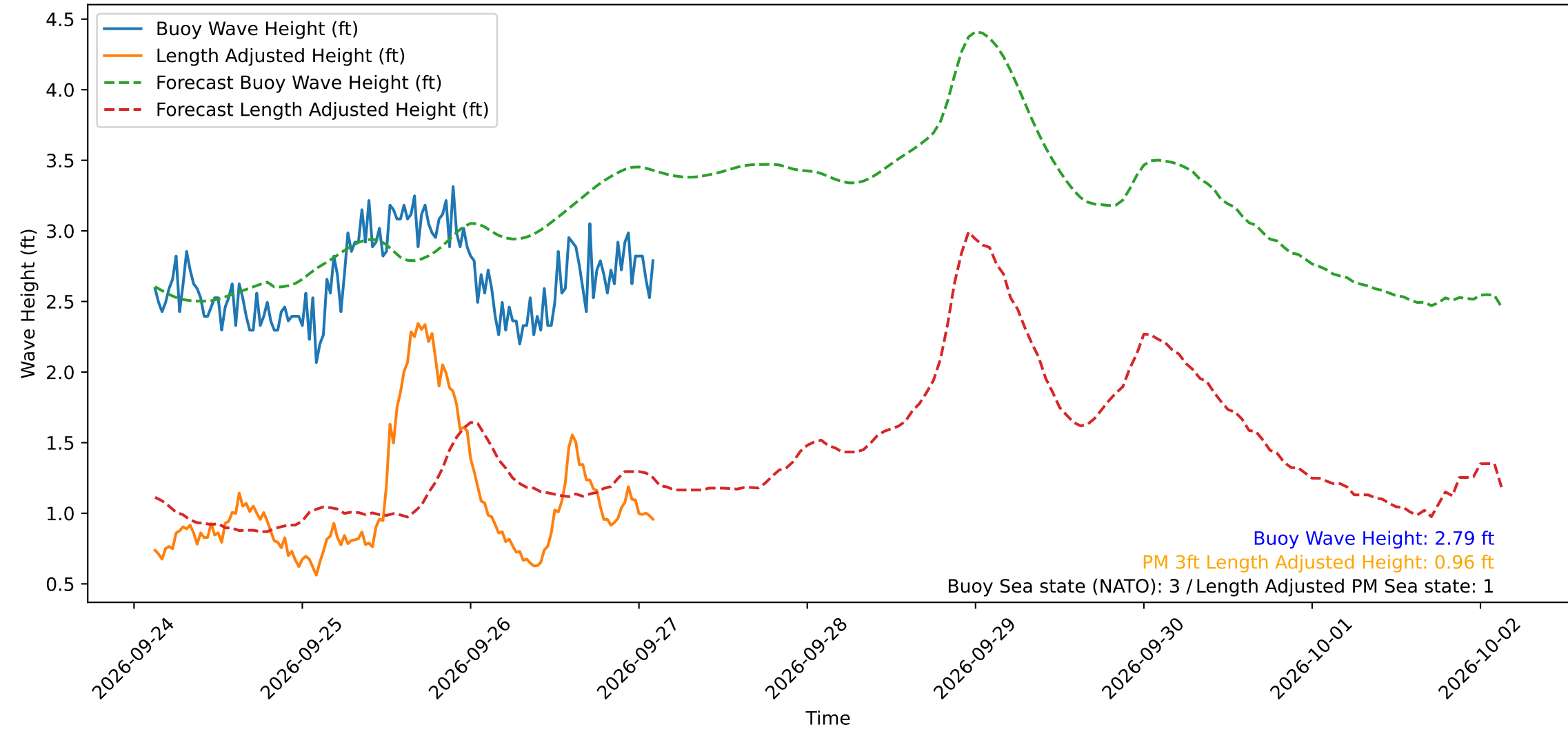
Wave Heights over Time for Red Beach at 2026-09-27 02:50:51
