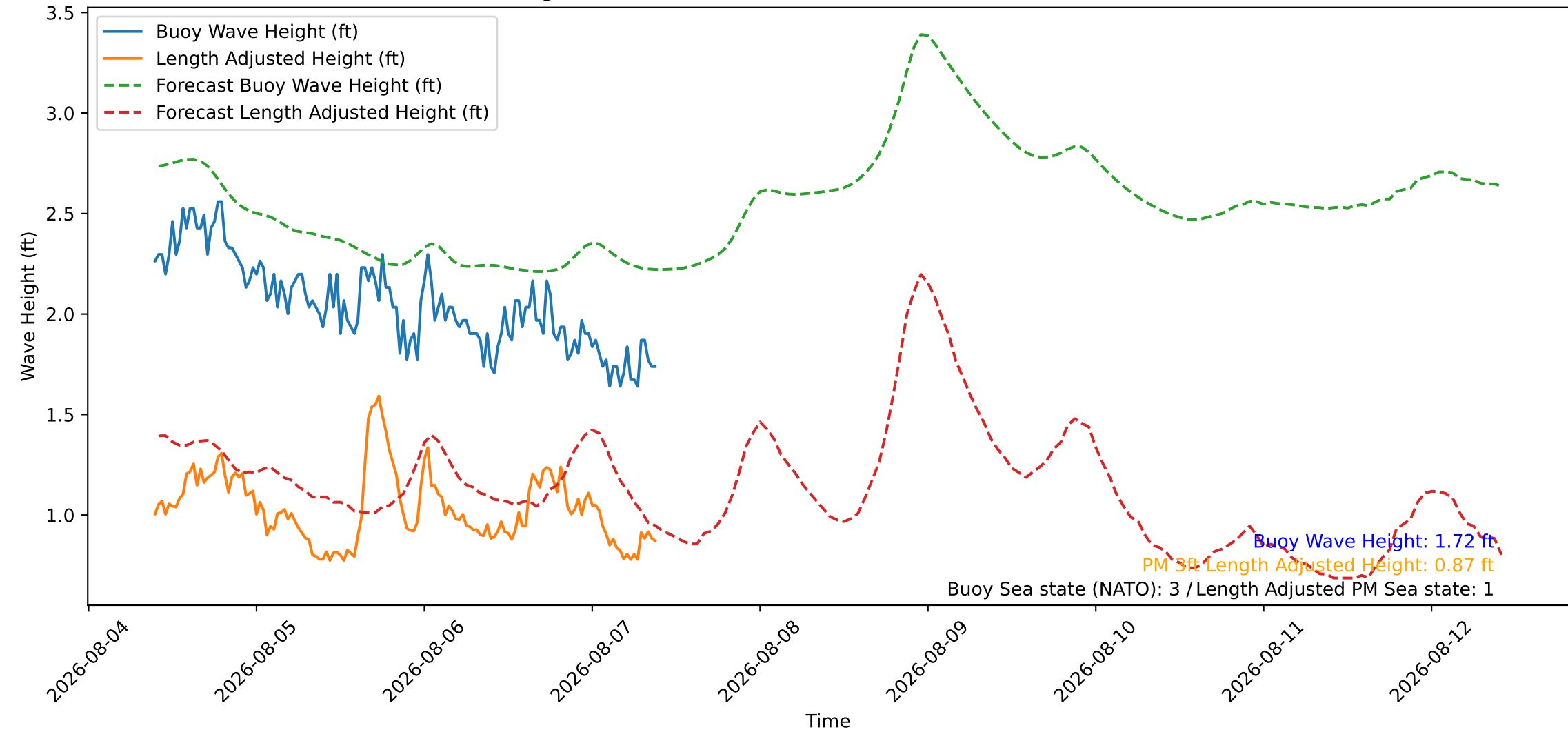
Wave Heights over Time for Oceanside Harbor at 2026-08-07 09:30:26
