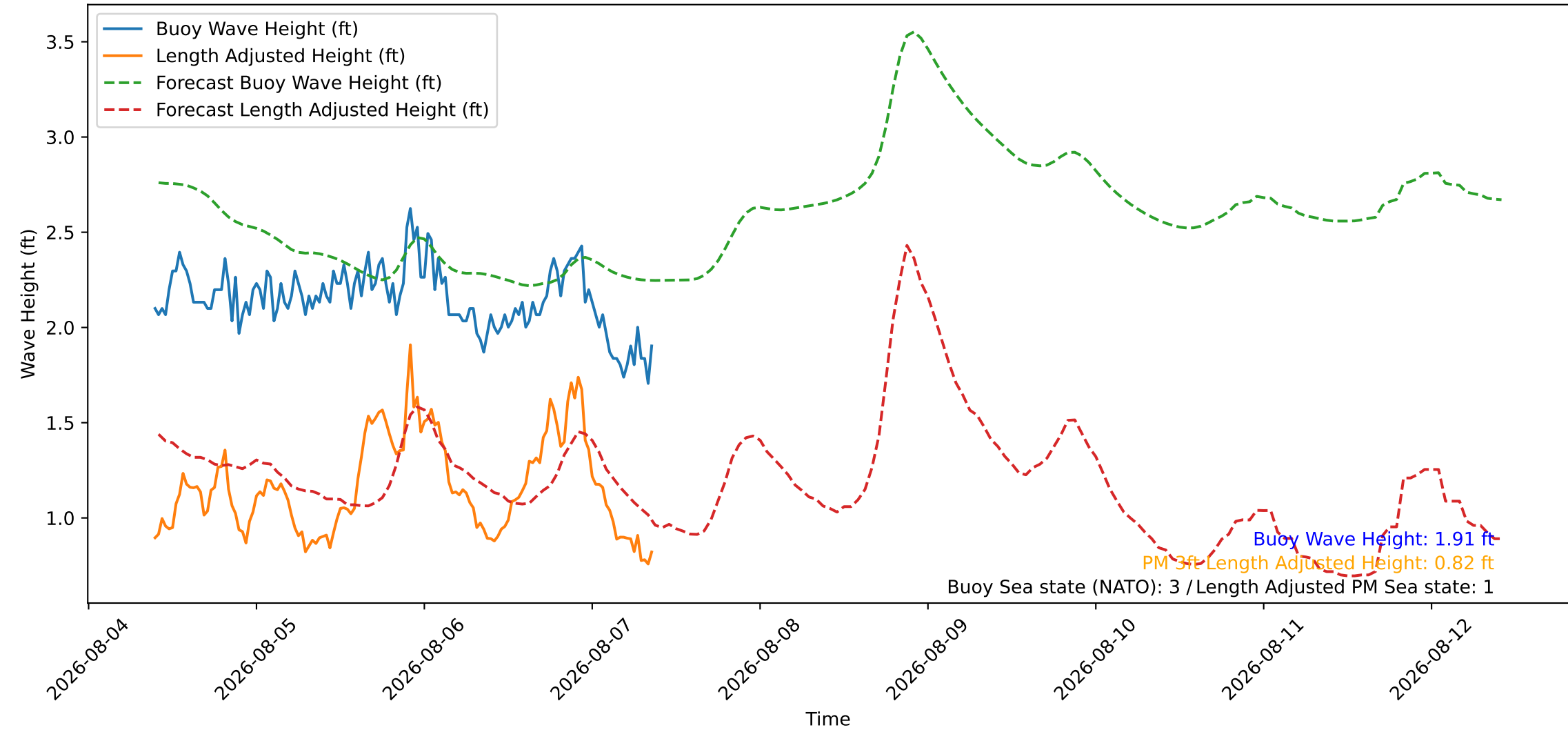
Wave Heights over Time for Green Beach at 2026-08-07 09:31:08
