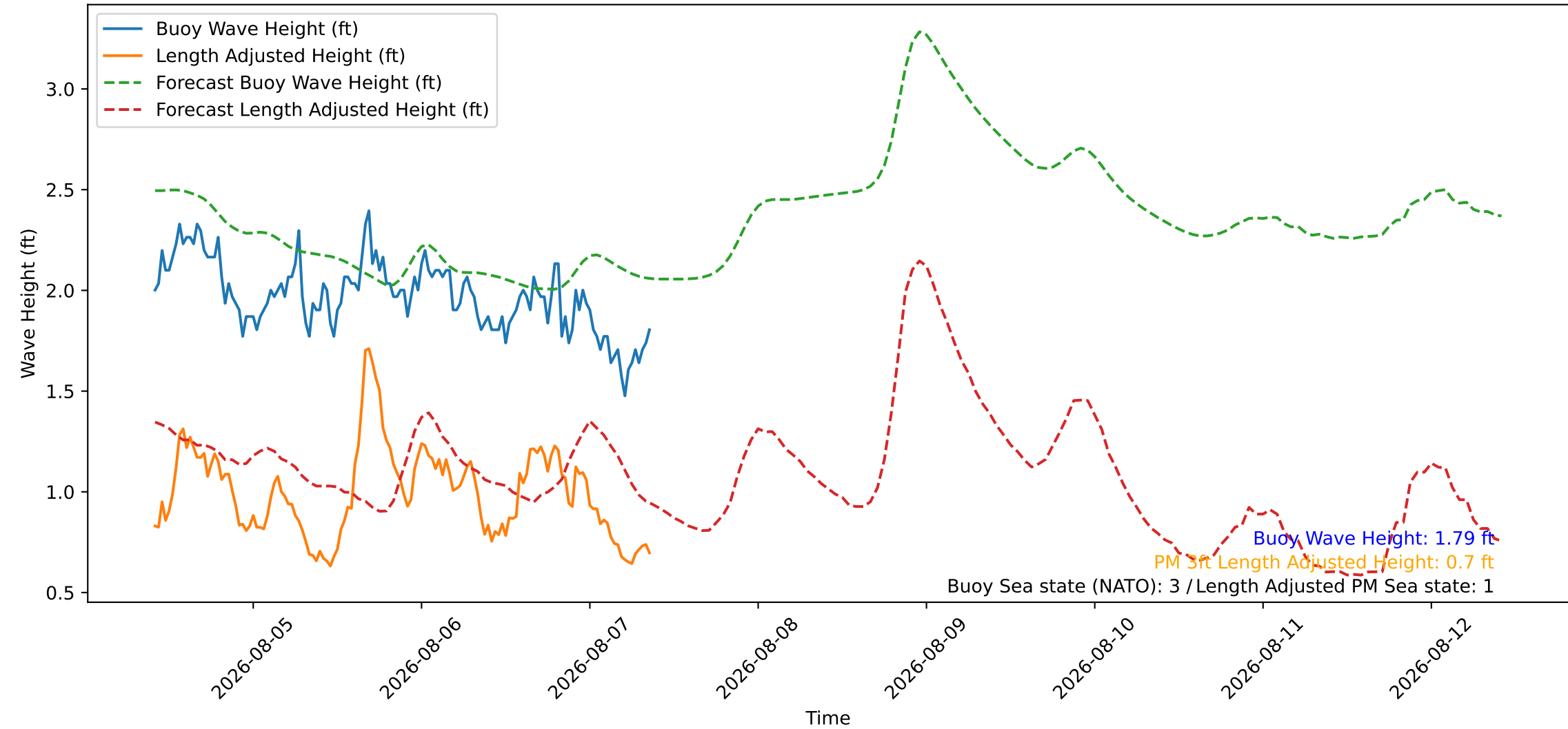
Wave Heights over Time for Red Beach at 2026-08-07 09:30:46
