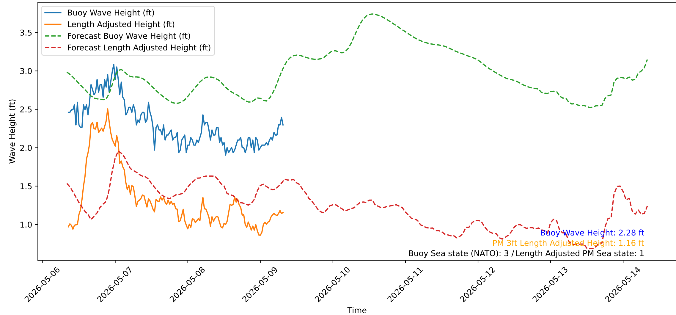
Wave Heights over Time for Red Beach at 2026-05-09 08:10:51
