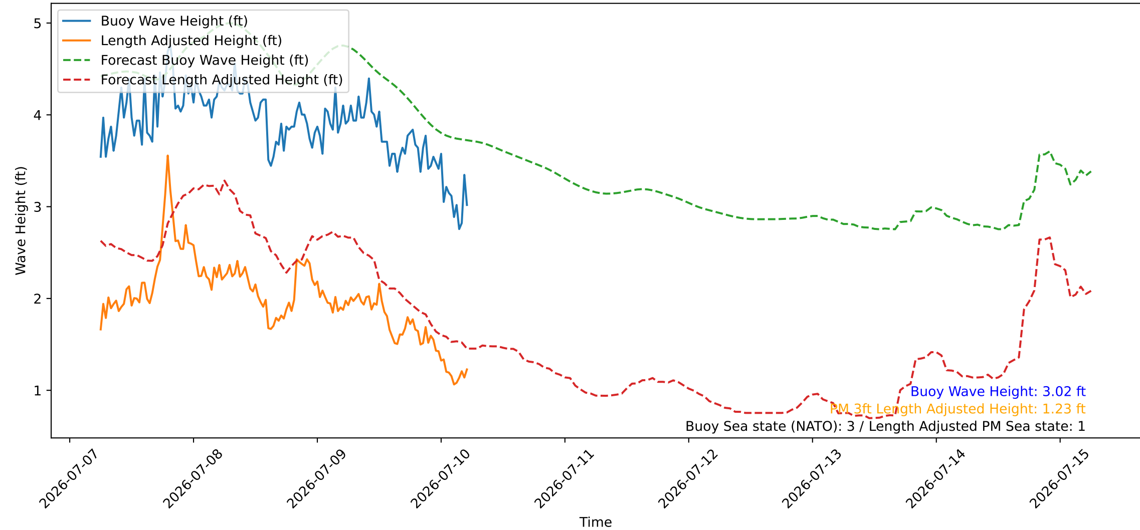
Wave Heights over Time for Green Beach at 2026-07-10 06:01:08
