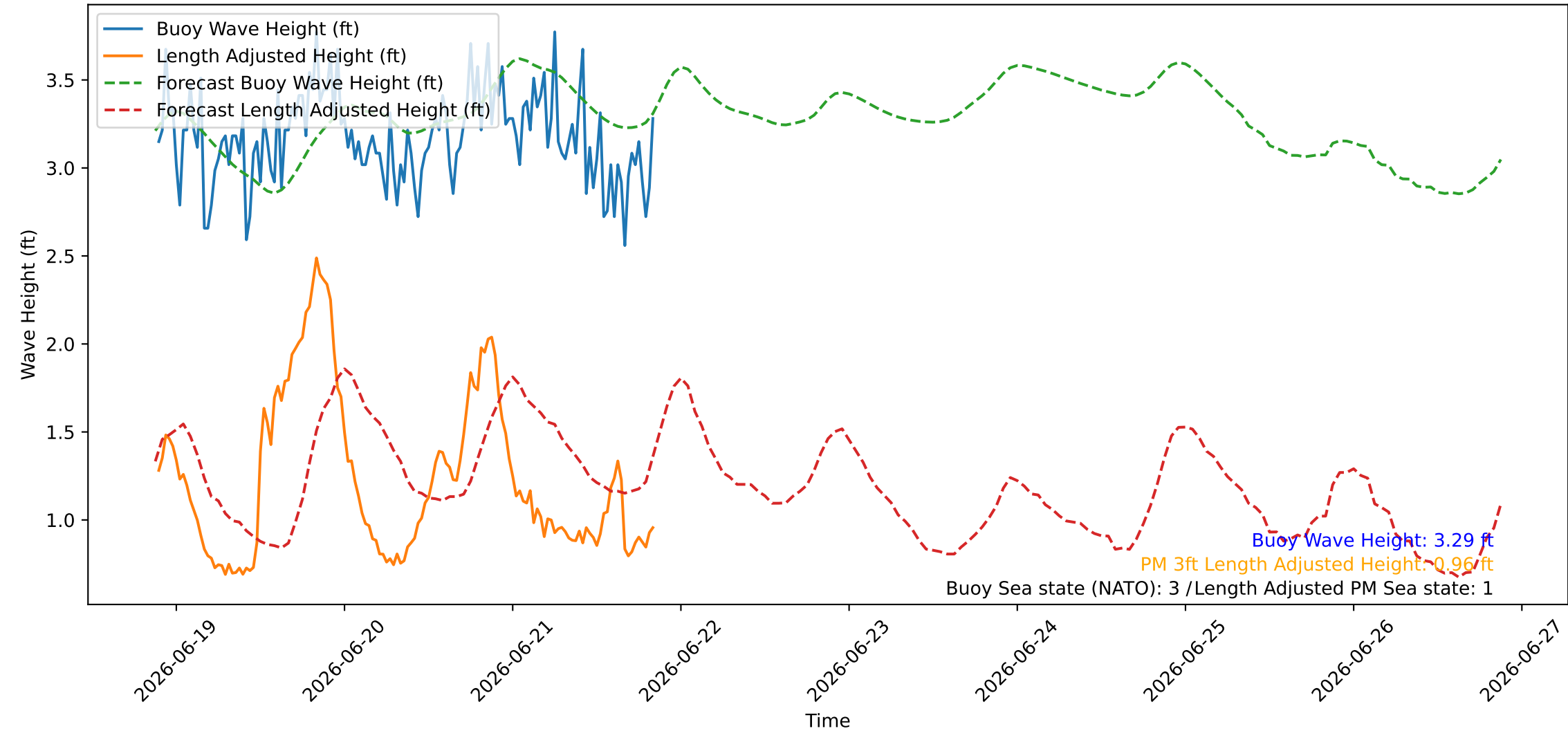
Wave Heights over Time for Red Beach at 2026-06-21 21:00:46
