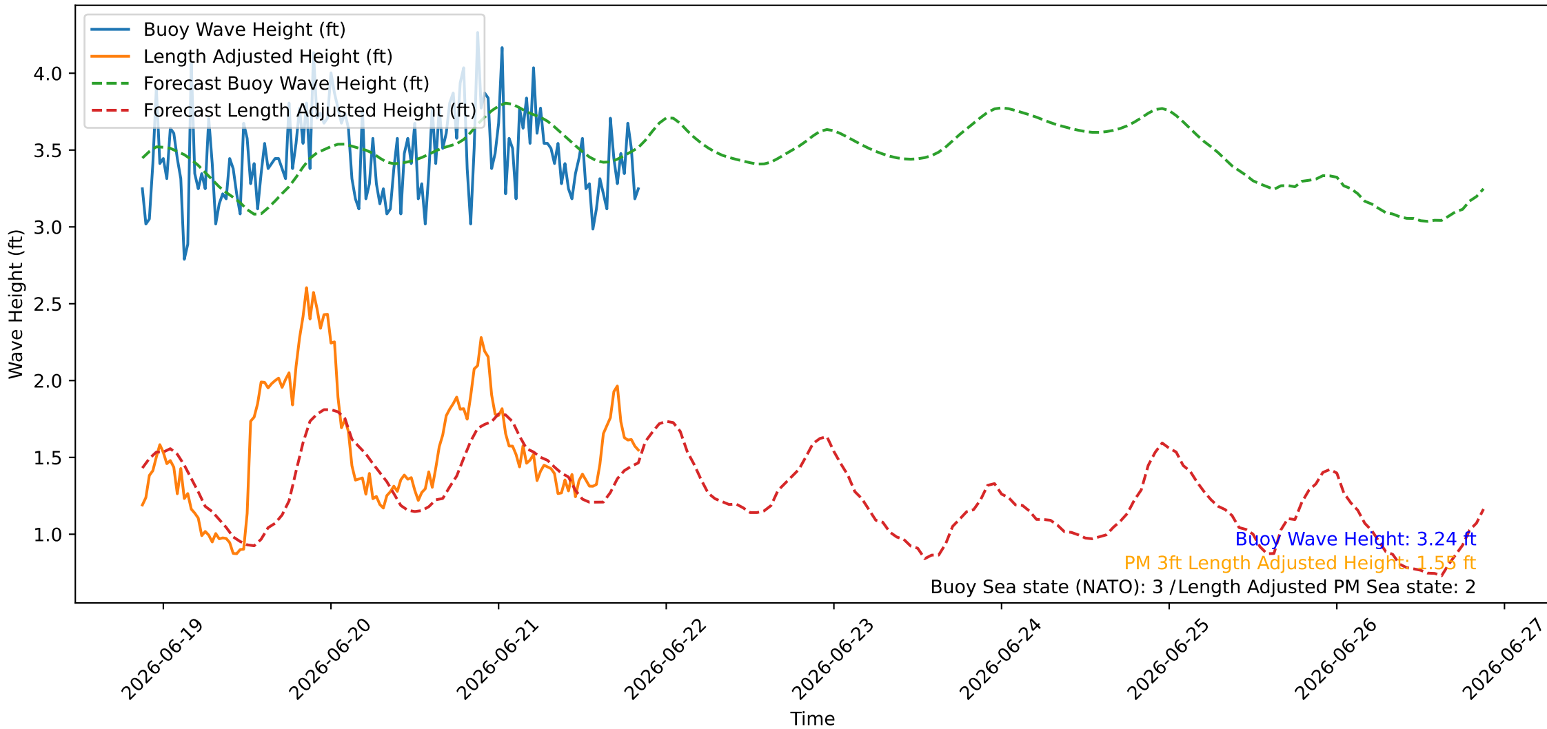
Wave Heights over Time for Oceanside Harbor at 2026-06-21 21:00:26
