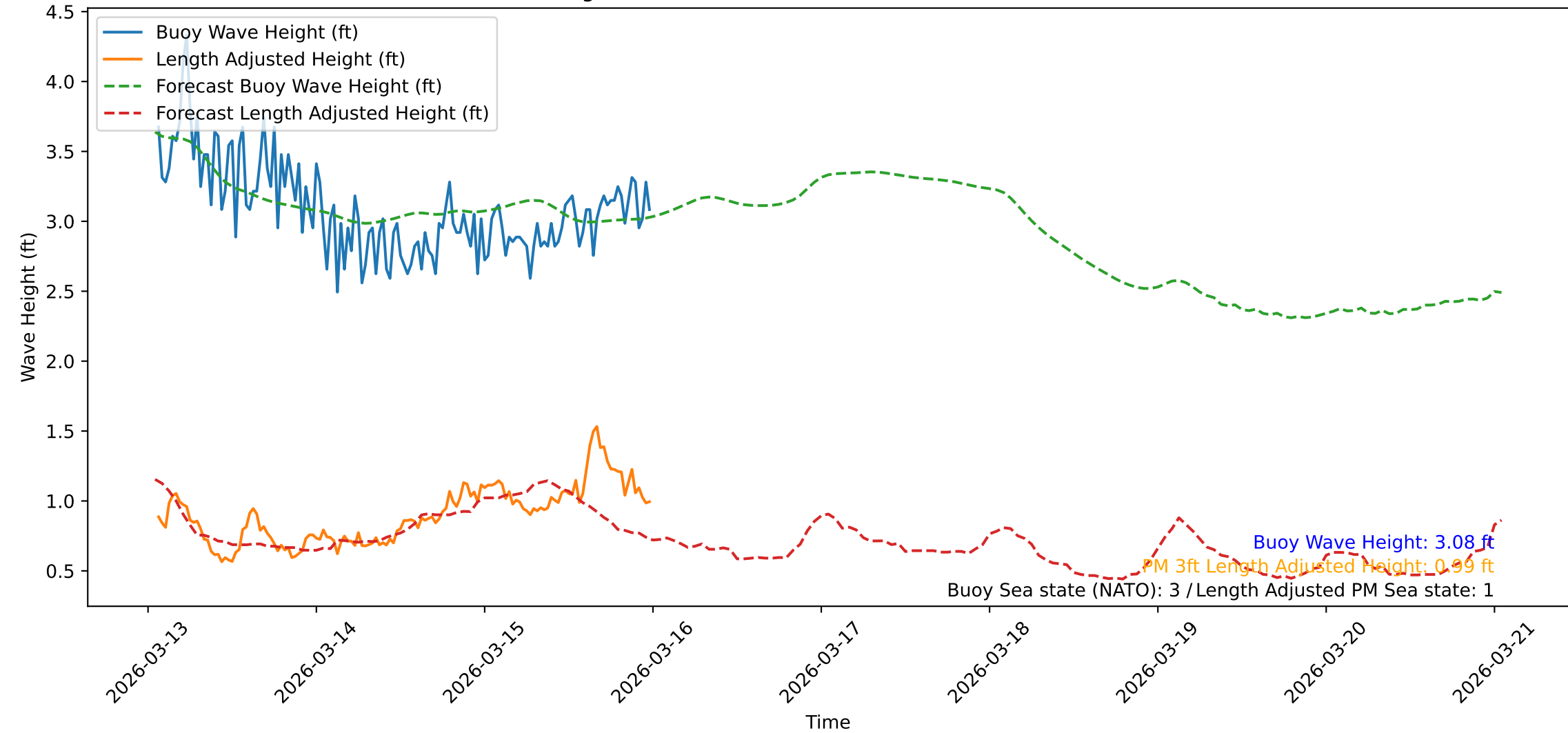
Wave Heights over Time for Red Beach at 2026-03-16 01:01:16
