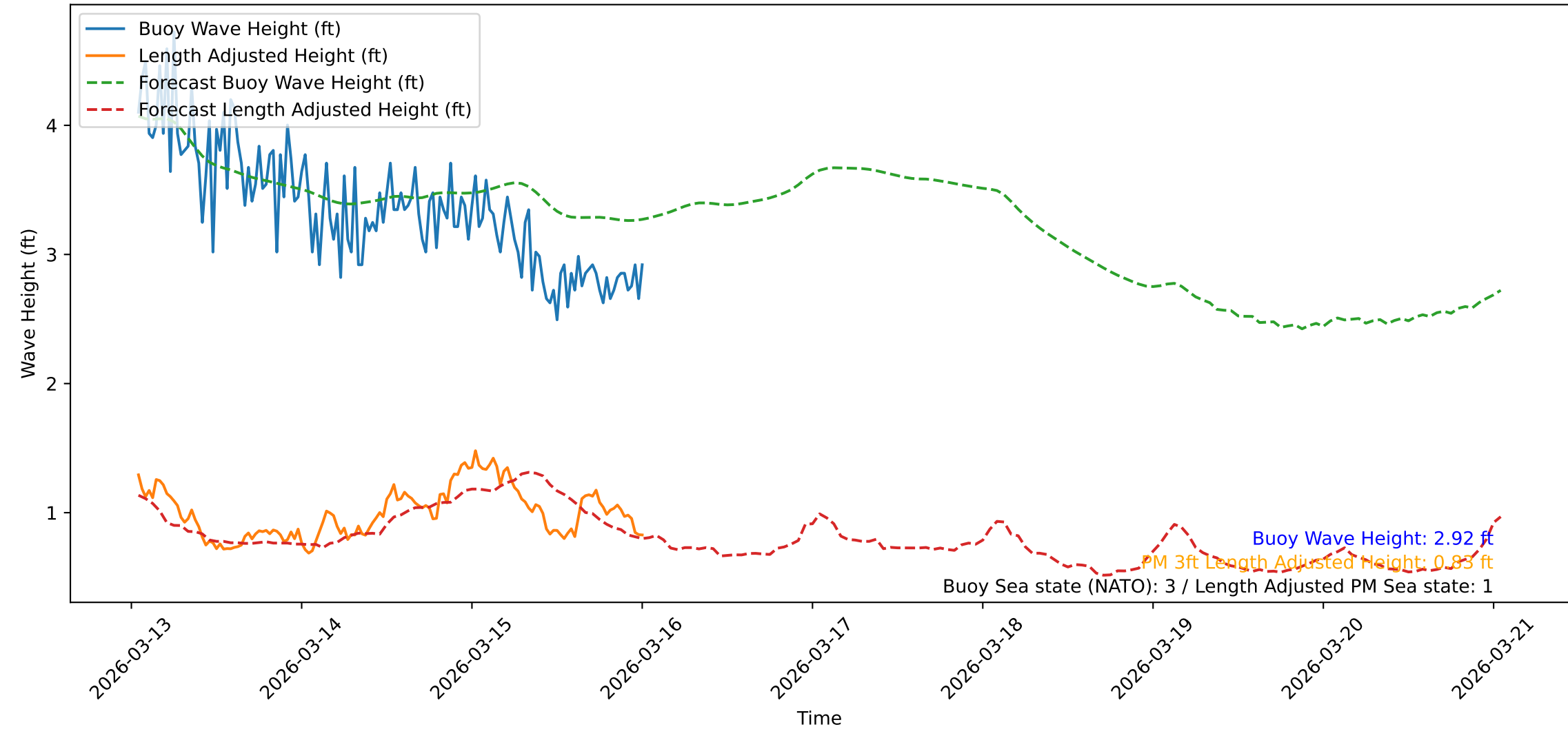
Wave Heights over Time for Oceanside Harbor at 2026-03-16 01:00:49
