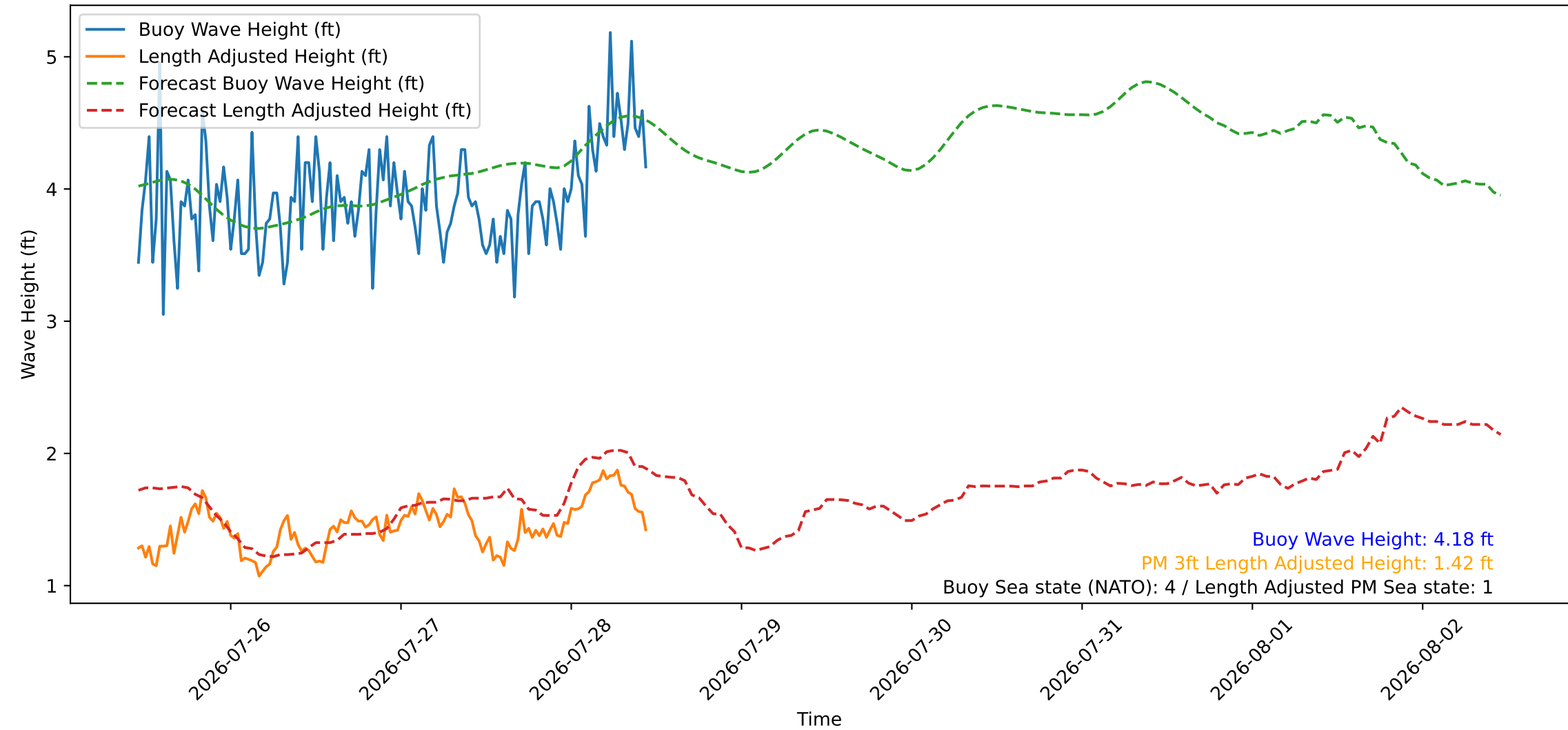
Wave Heights over Time for Oceanside Harbor at 2026-07-28 11:10:27
