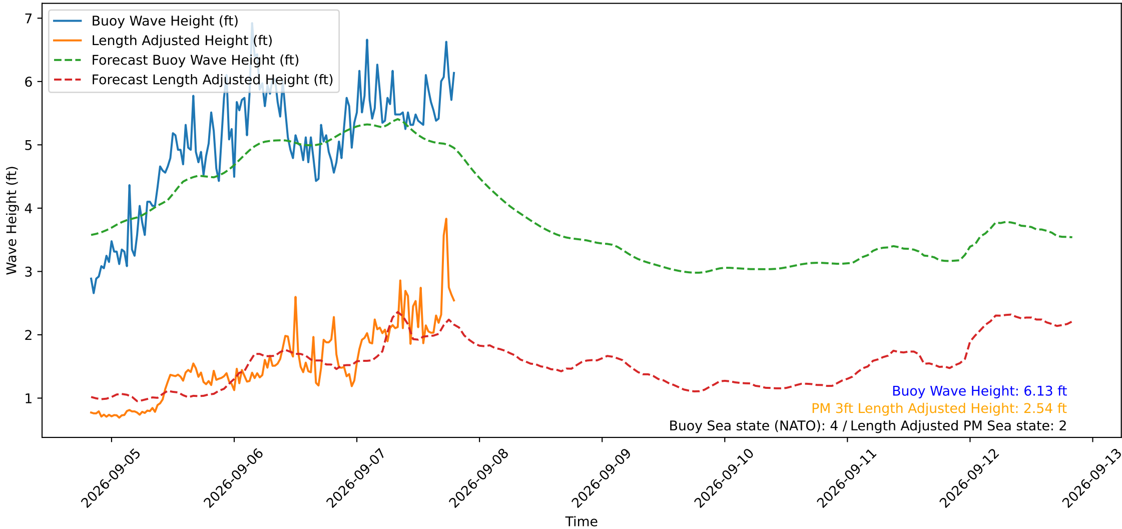
Wave Heights over Time for Red Beach at 2026-09-07 19:40:49
