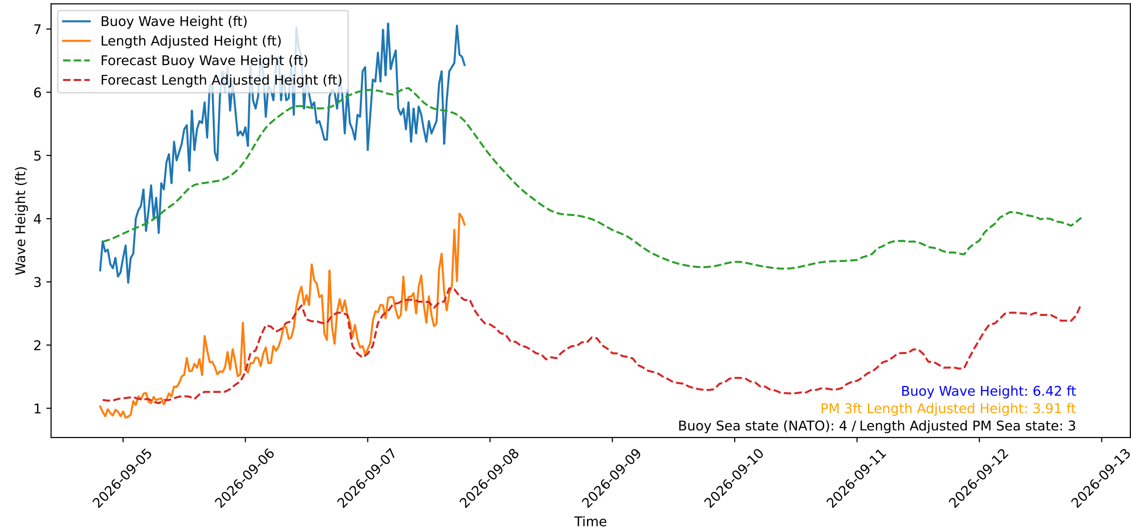
Wave Heights over Time for Oceanside Harbor at 2026-09-07 19:40:30
