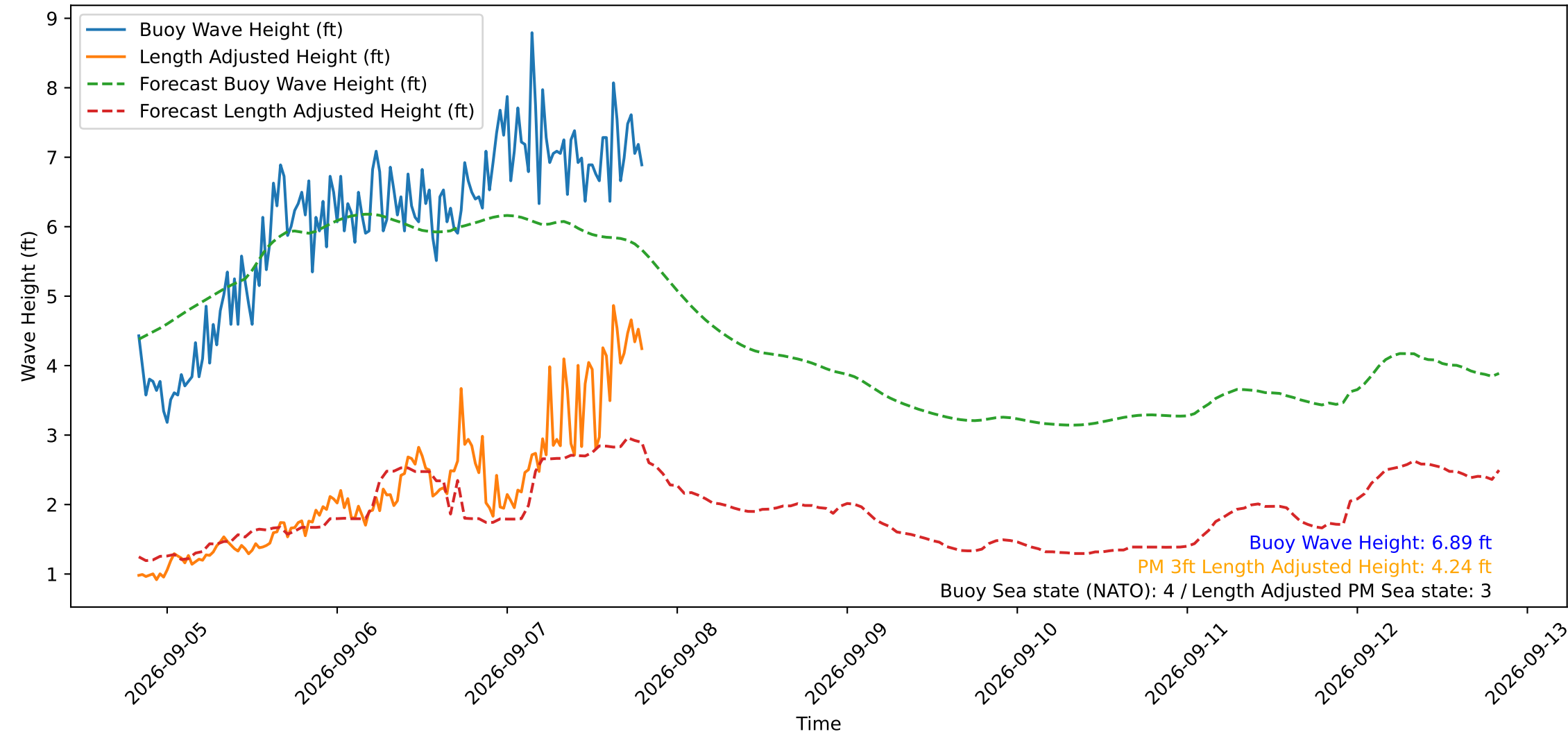
Wave Heights over Time for Green Beach at 2026-09-07 19:41:12
