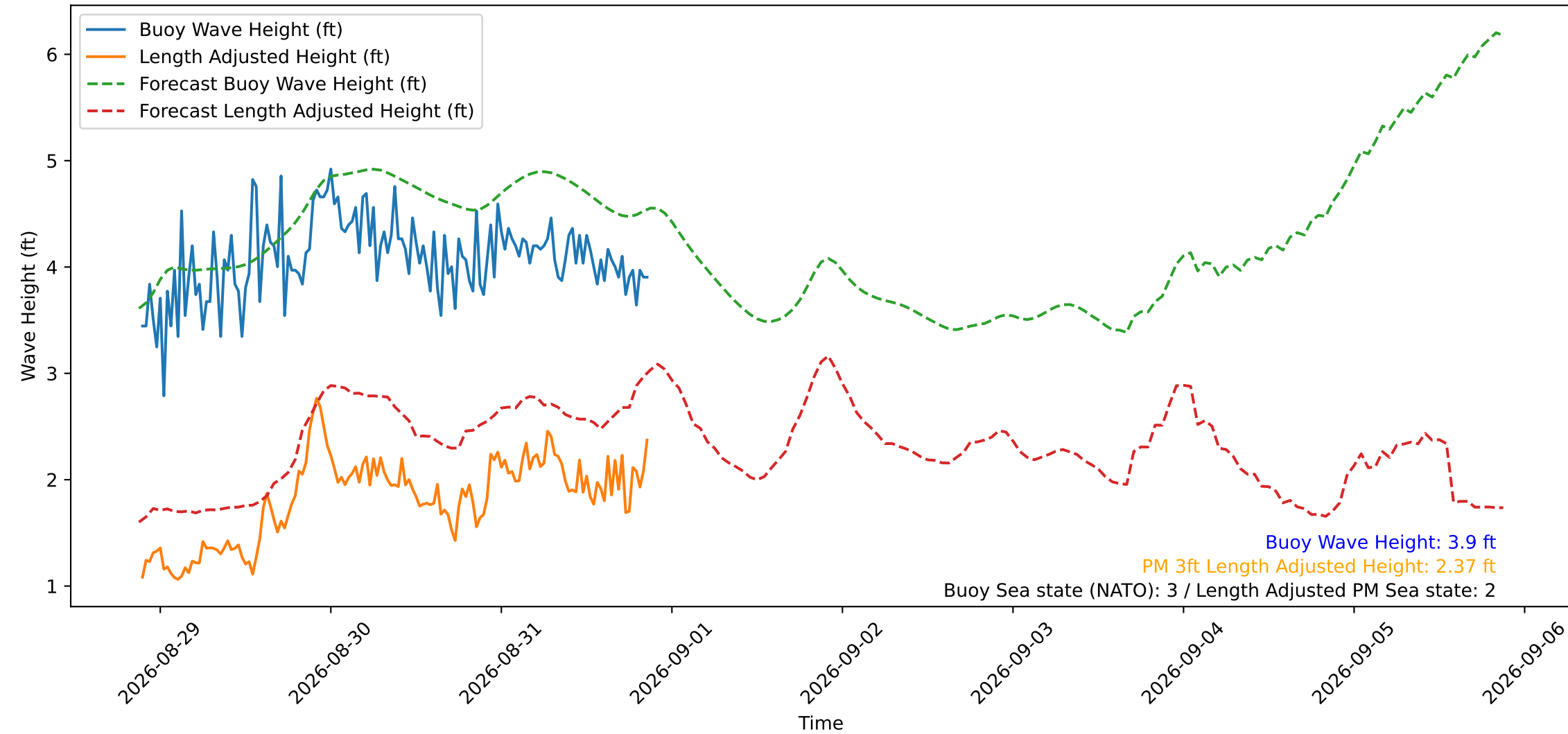
Wave Heights over Time for Green Beach at 2026-08-31 21:11:11
