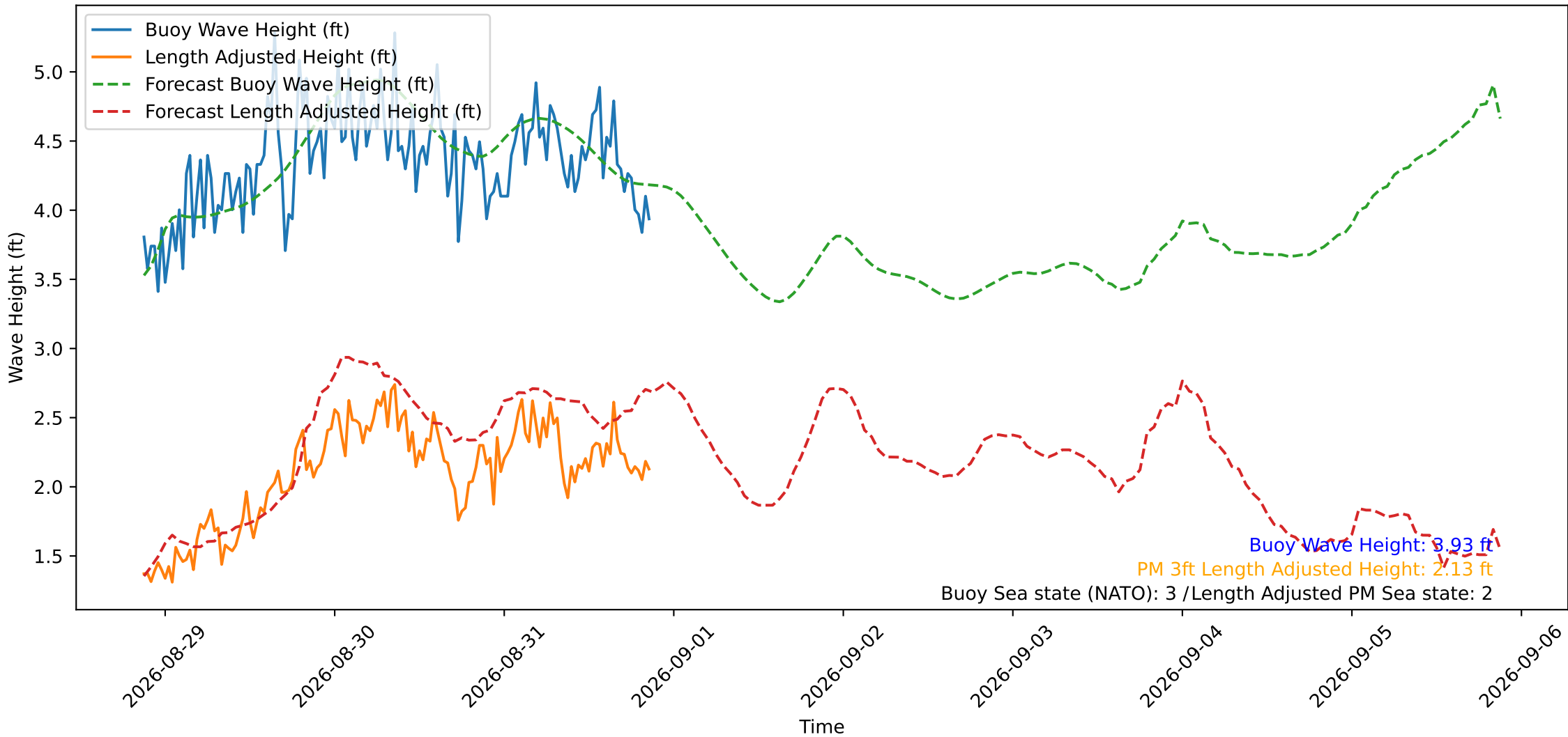
Wave Heights over Time for Oceanside Harbor at 2026-08-31 21:10:29
