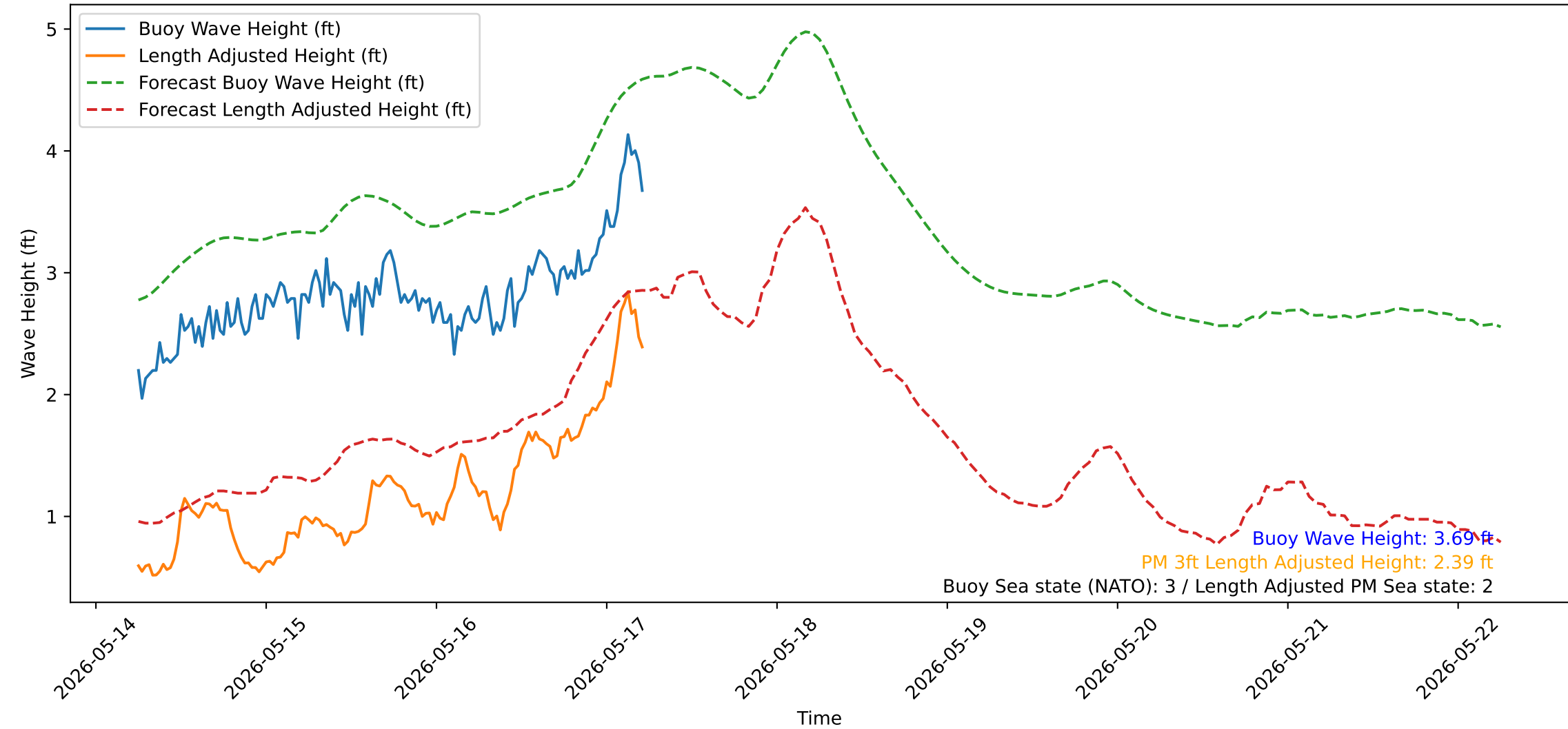
Wave Heights over Time for Red Beach at 2026-05-17 05:50:53
