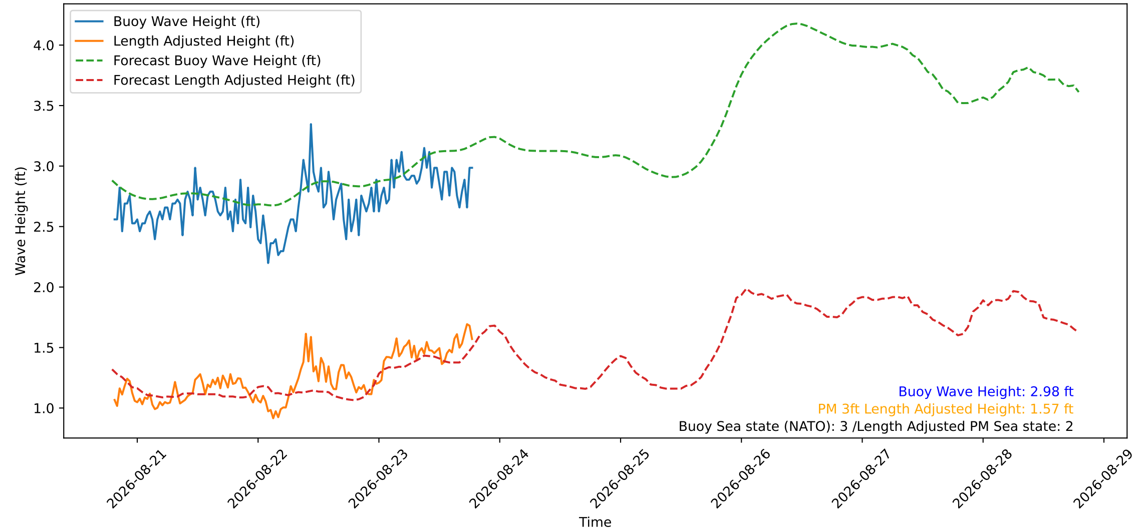
Wave Heights over Time for Oceanside Harbor at 2026-08-23 19:20:30
