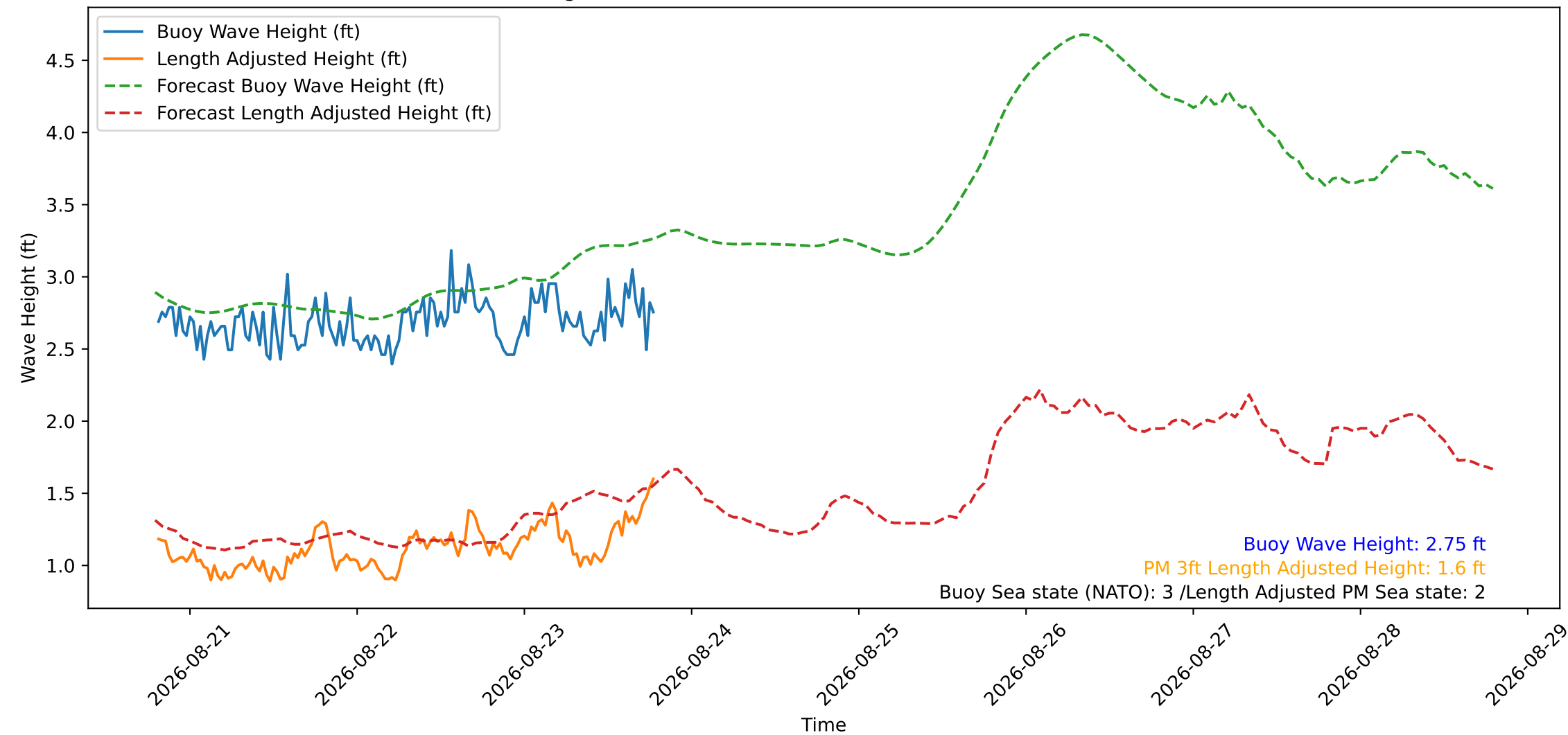
Wave Heights over Time for Green Beach at 2026-08-23 19:21:17
