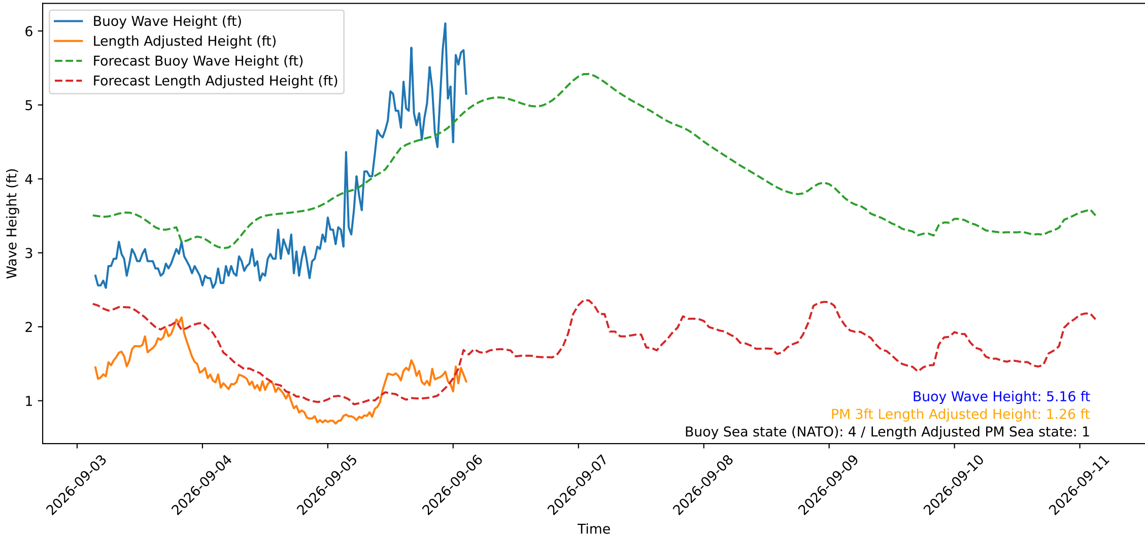
Wave Heights over Time for Red Beach at 2026-09-06 03:20:51
