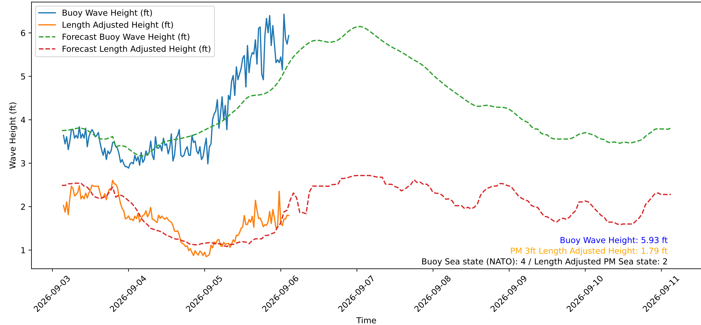
Wave Heights over Time for Oceanside Harbor at 2026-09-06 03:20:30
