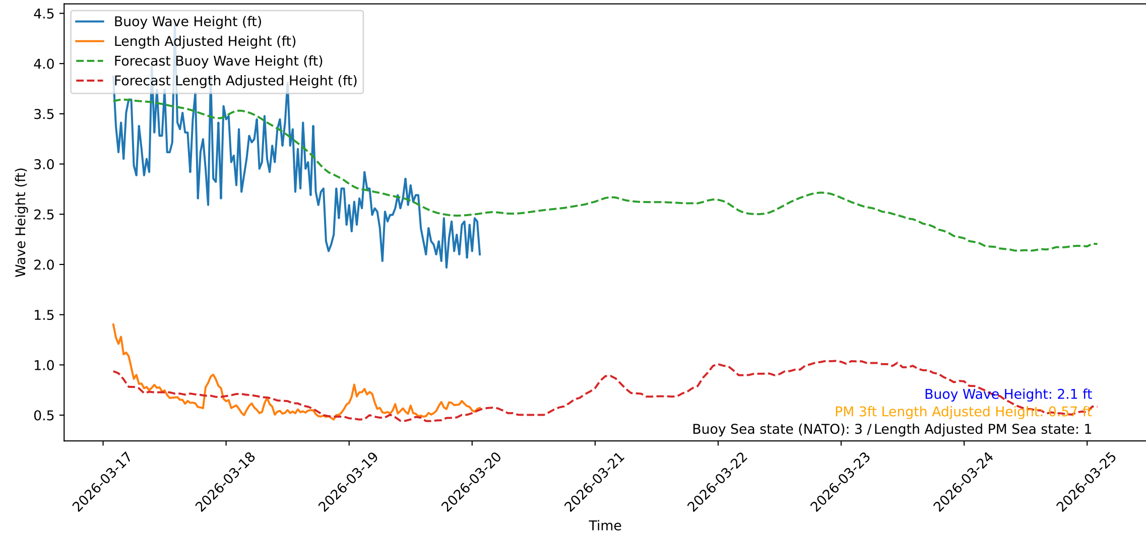
Wave Heights over Time for Oceanside Harbor at 2026-03-20 02:10:31
