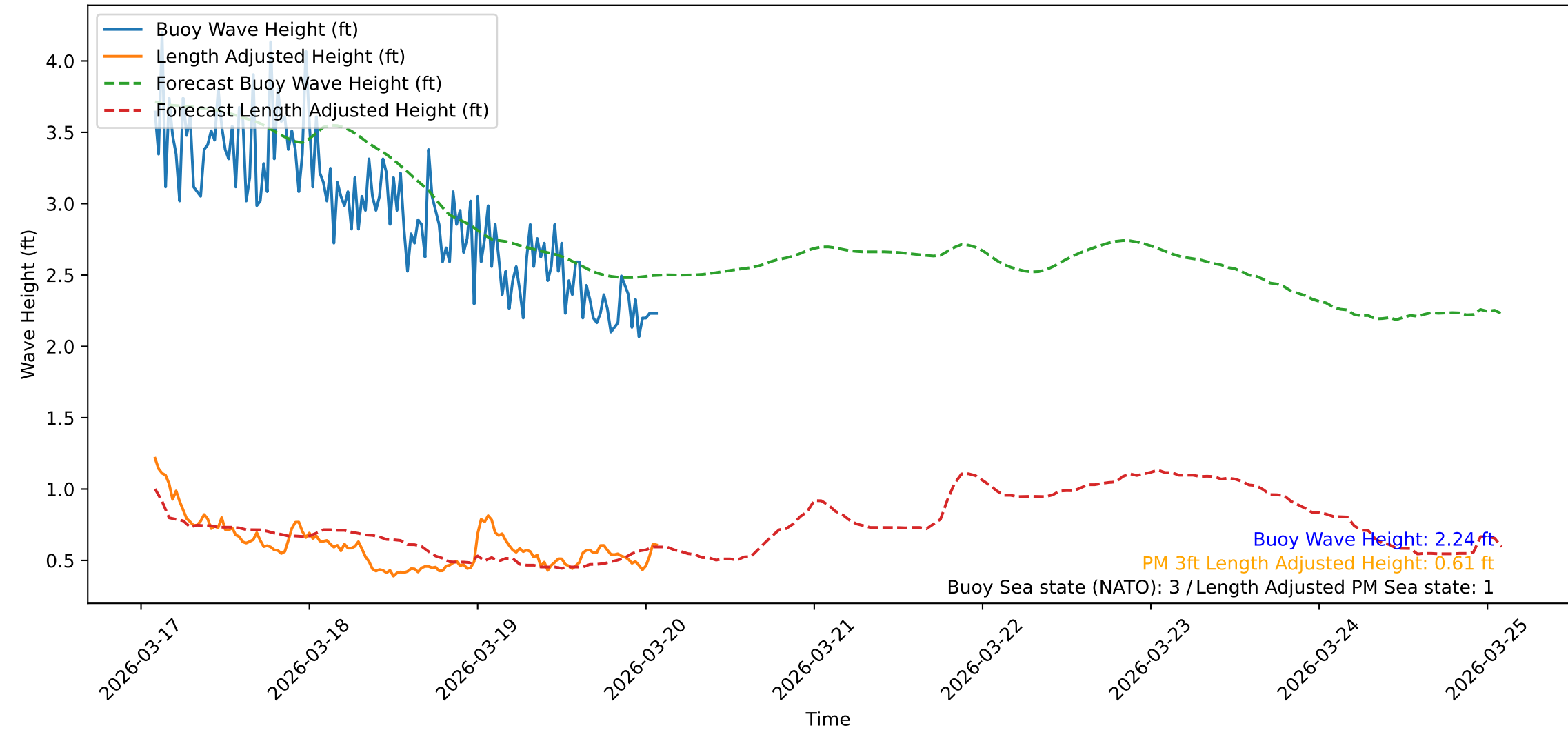
Wave Heights over Time for Green Beach at 2026-03-20 02:11:09
