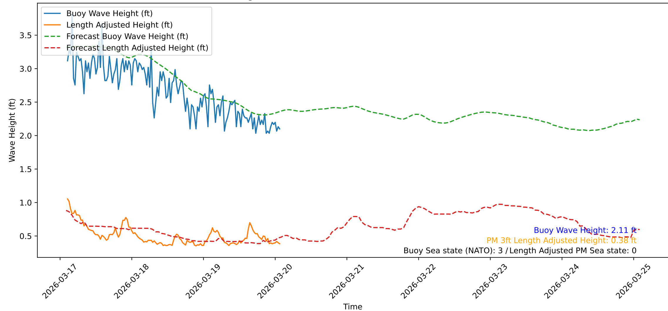
Wave Heights over Time for Red Beach at 2026-03-20 02:10:47
