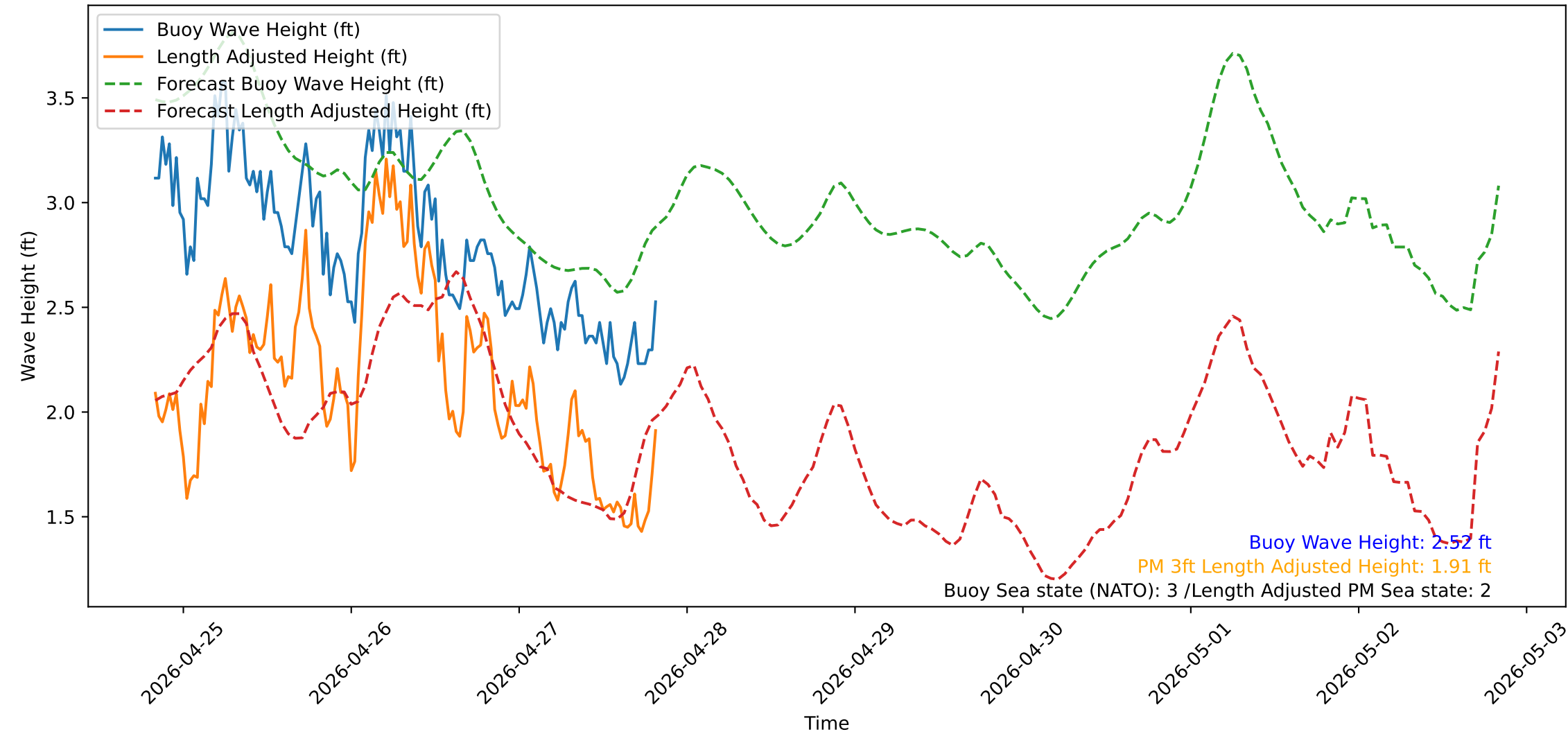
Wave Heights over Time for Green Beach at 2026-04-27 20:11:12
