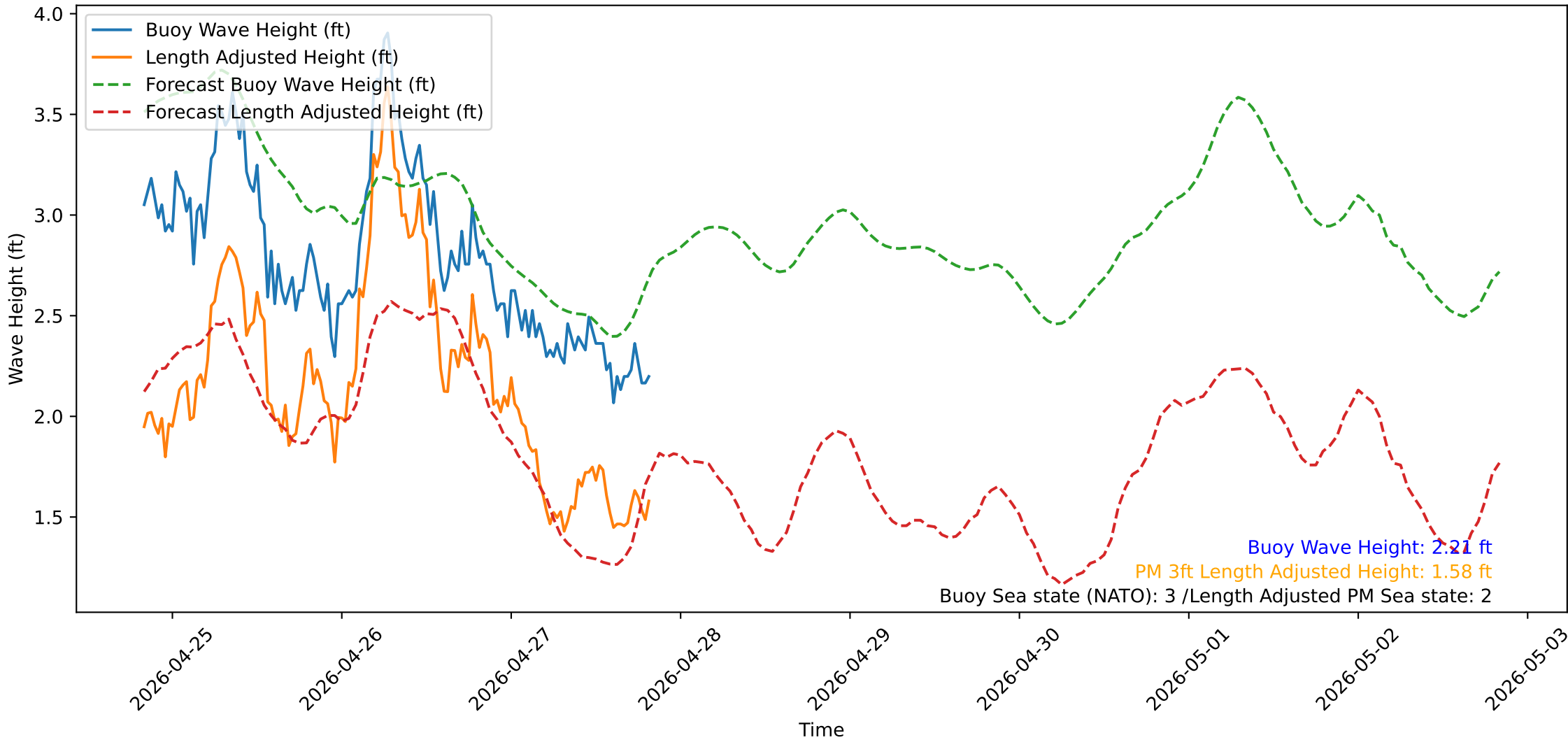
Wave Heights over Time for Oceanside Harbor at 2026-04-27 20:10:31
