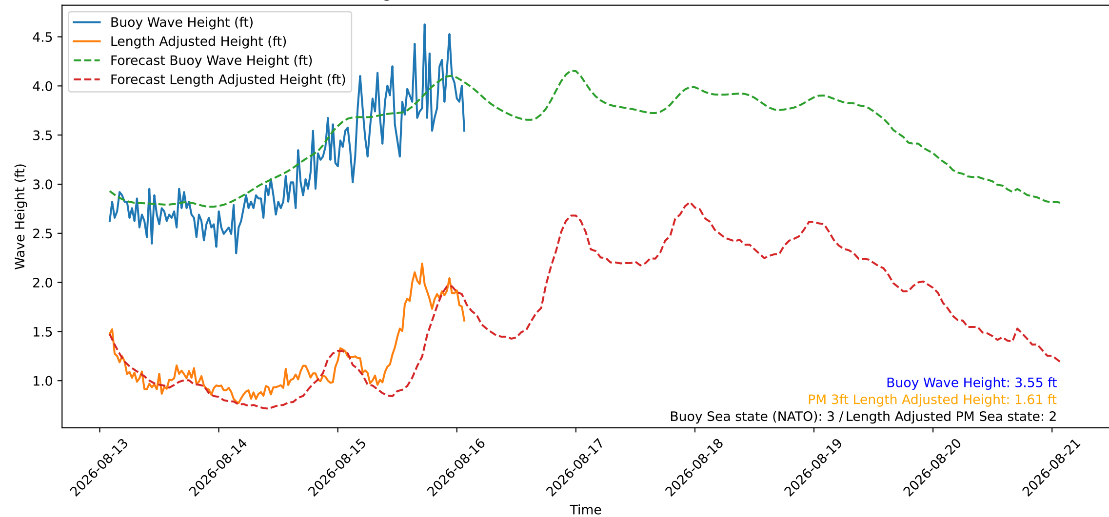
Wave Heights over Time for Oceanside Harbor at 2026-08-16 02:00:27
