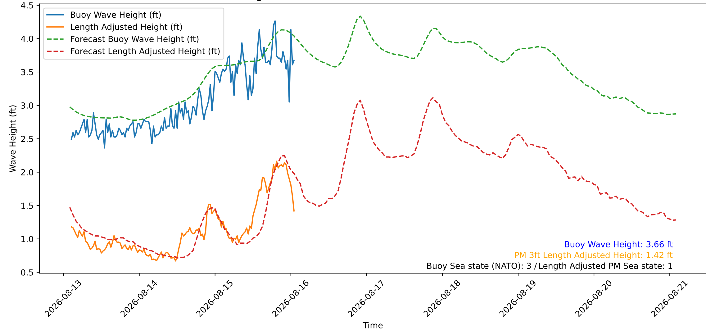
Wave Heights over Time for Green Beach at 2026-08-16 02:01:09
