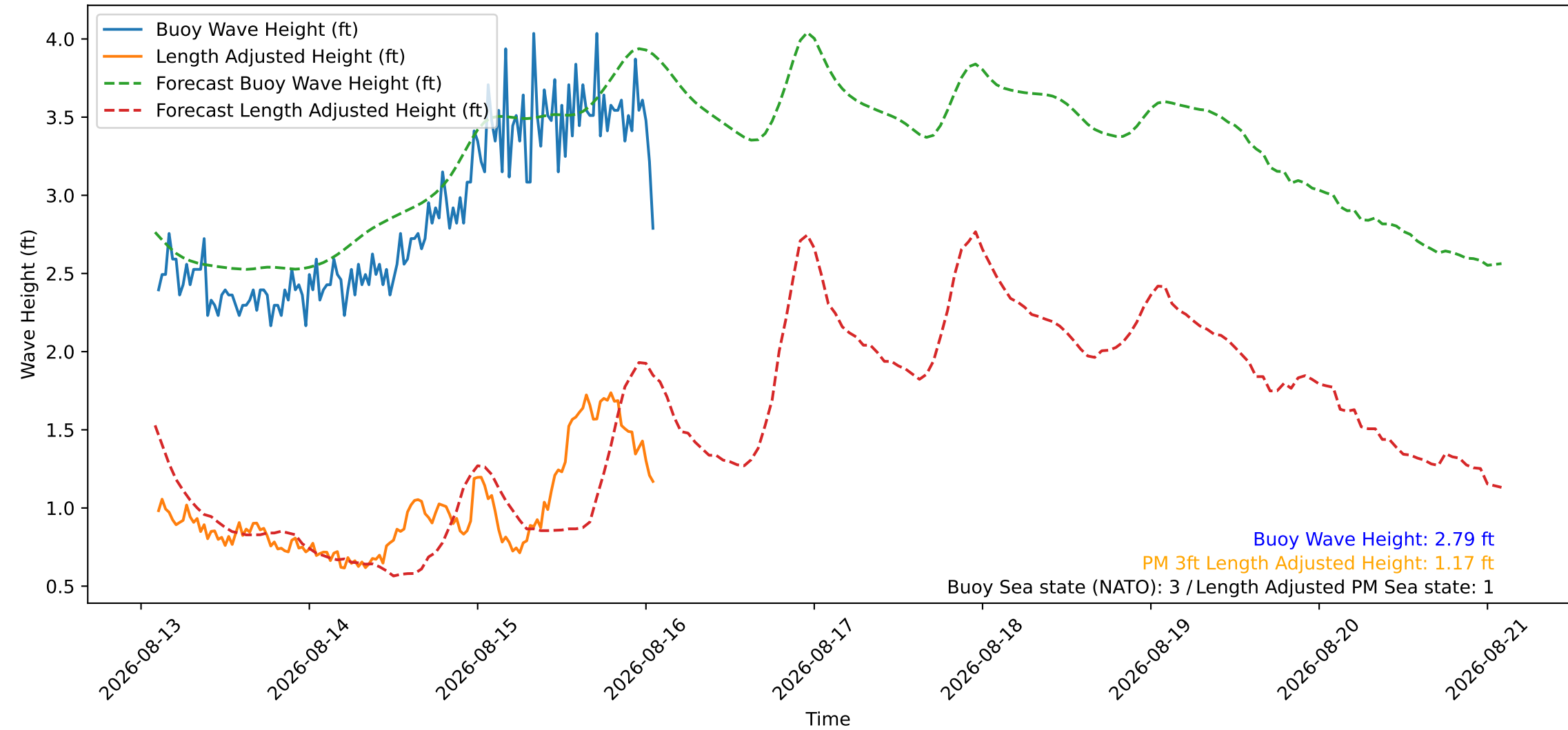
Wave Heights over Time for Red Beach at 2026-08-16 02:00:47
