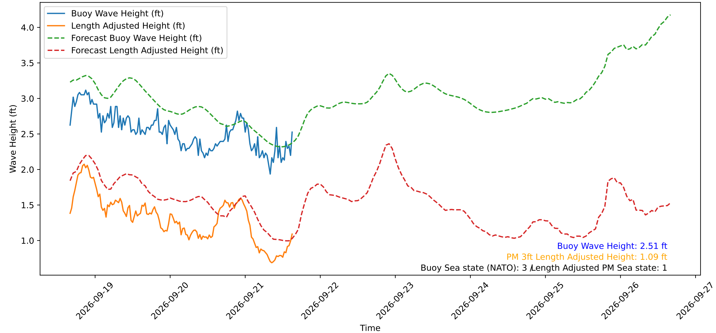
Wave Heights over Time for Green Beach at 2026-09-21 15:51:14
