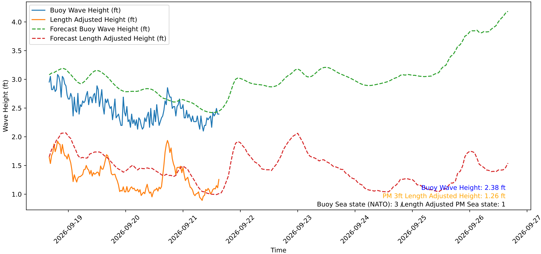
Wave Heights over Time for Oceanside Harbor at 2026-09-21 15:50:30
