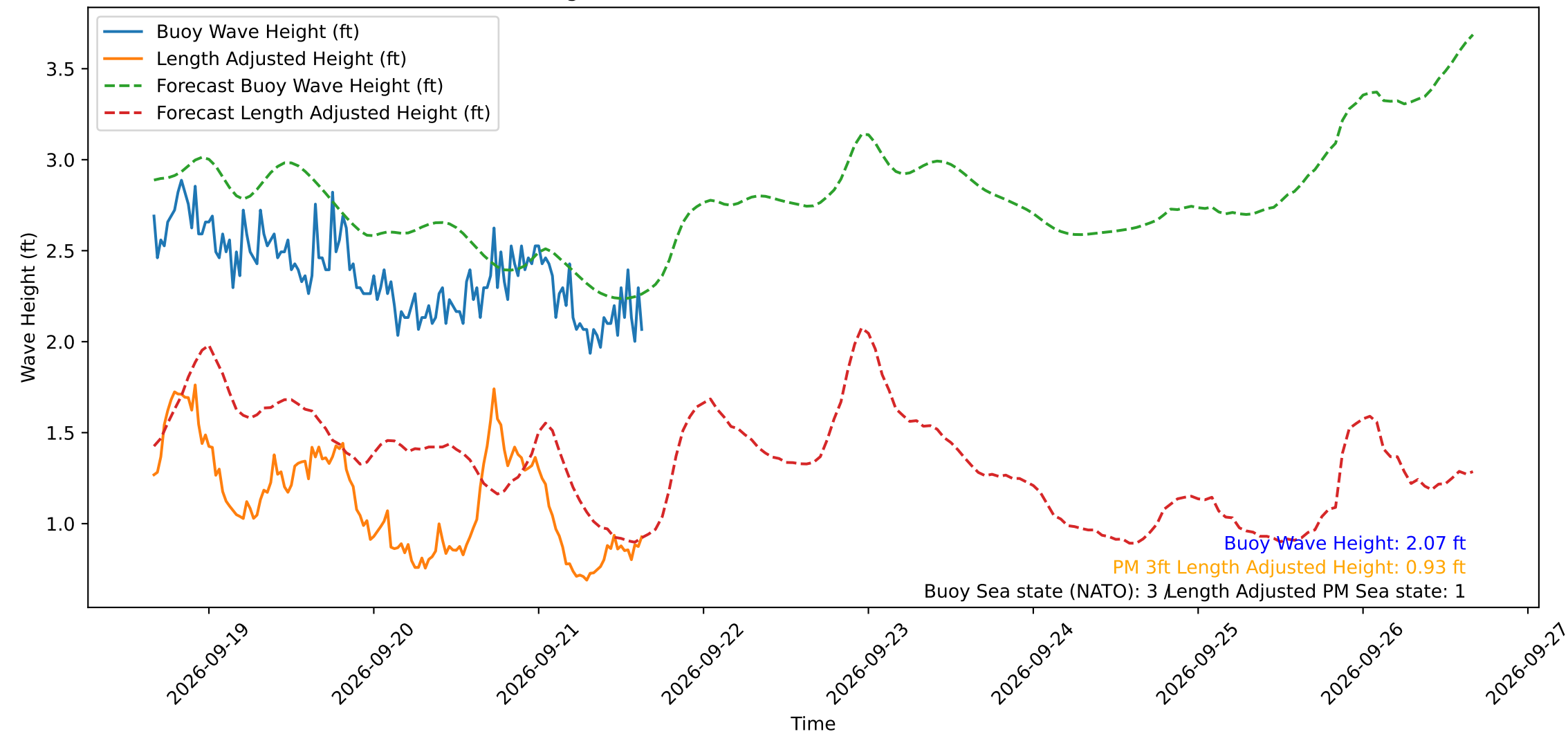
Wave Heights over Time for Red Beach at 2026-09-21 15:50:50
