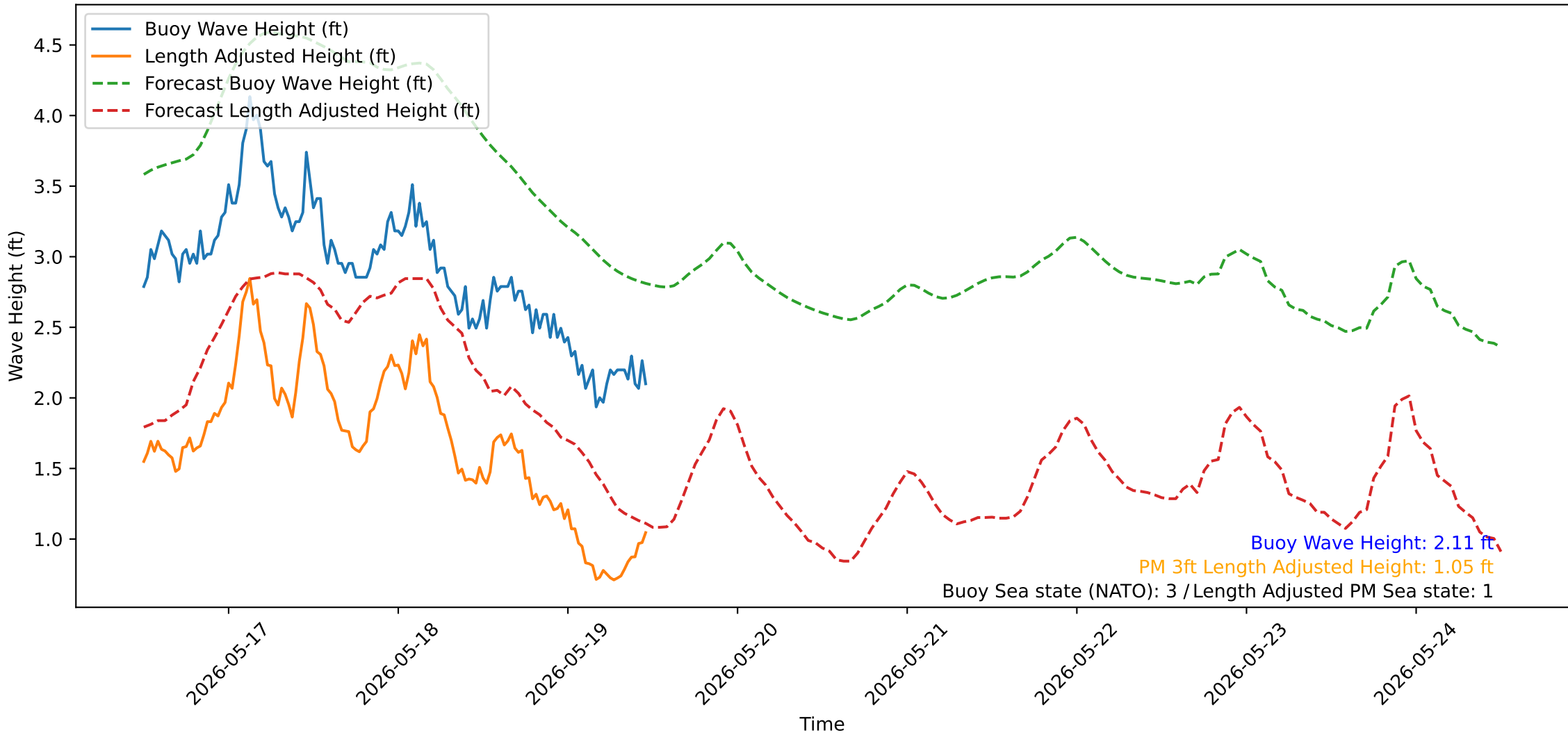
Wave Heights over Time for Red Beach at 2026-05-19 11:50:53
