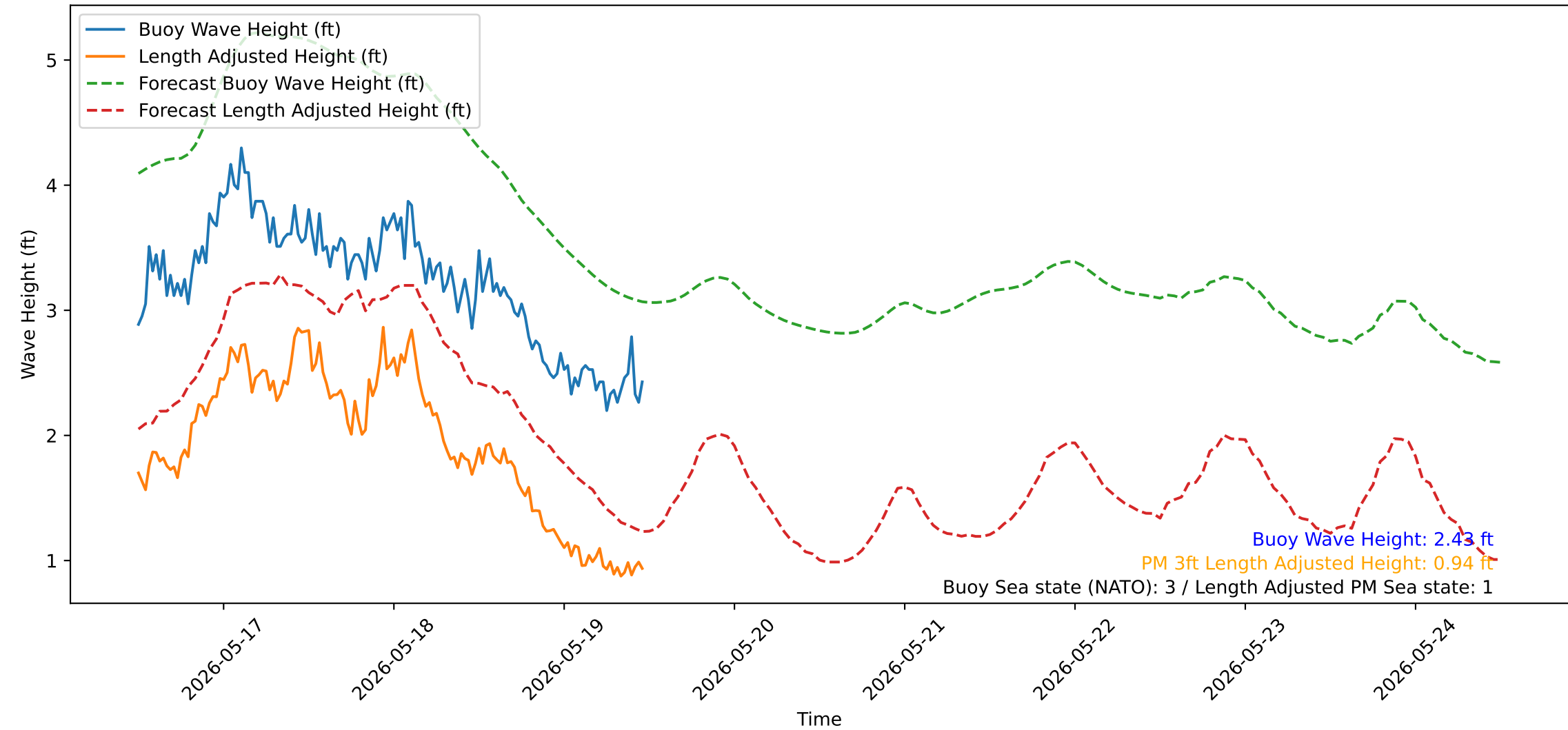
Wave Heights over Time for Oceanside Harbor at 2026-05-19 11:50:32
