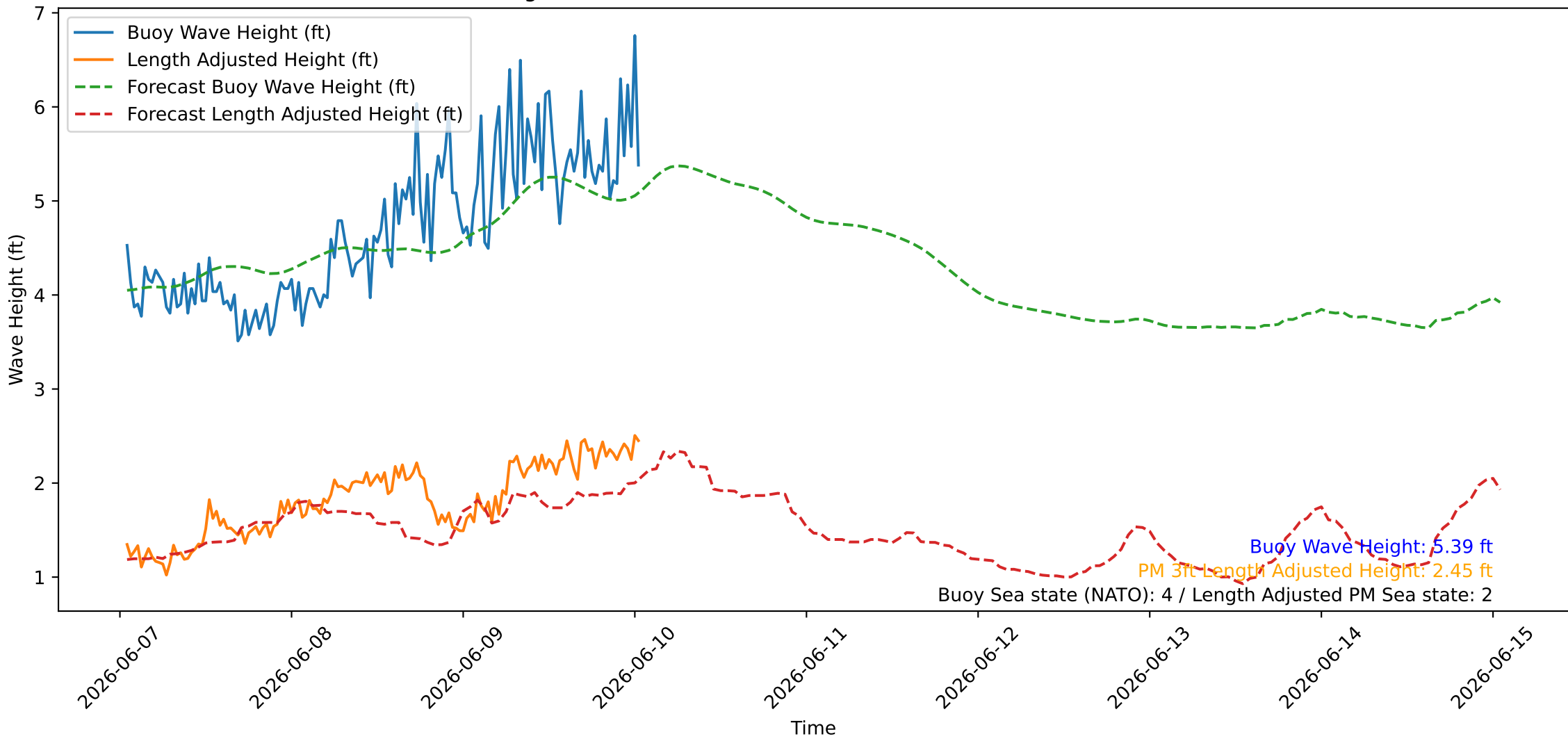
Wave Heights over Time for Oceanside Harbor at 2026-06-10 01:10:27
