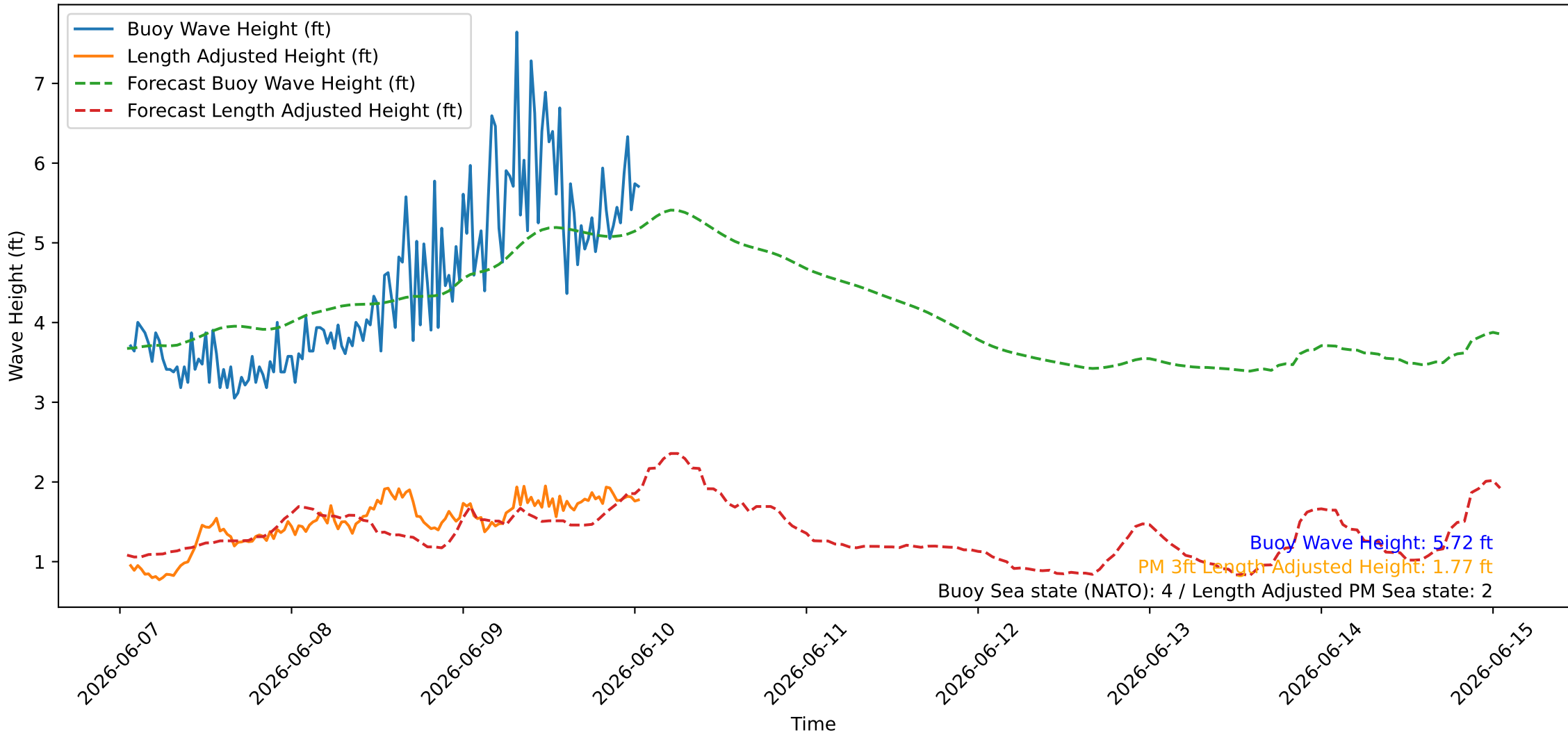
Wave Heights over Time for Red Beach at 2026-06-10 01:10:47
