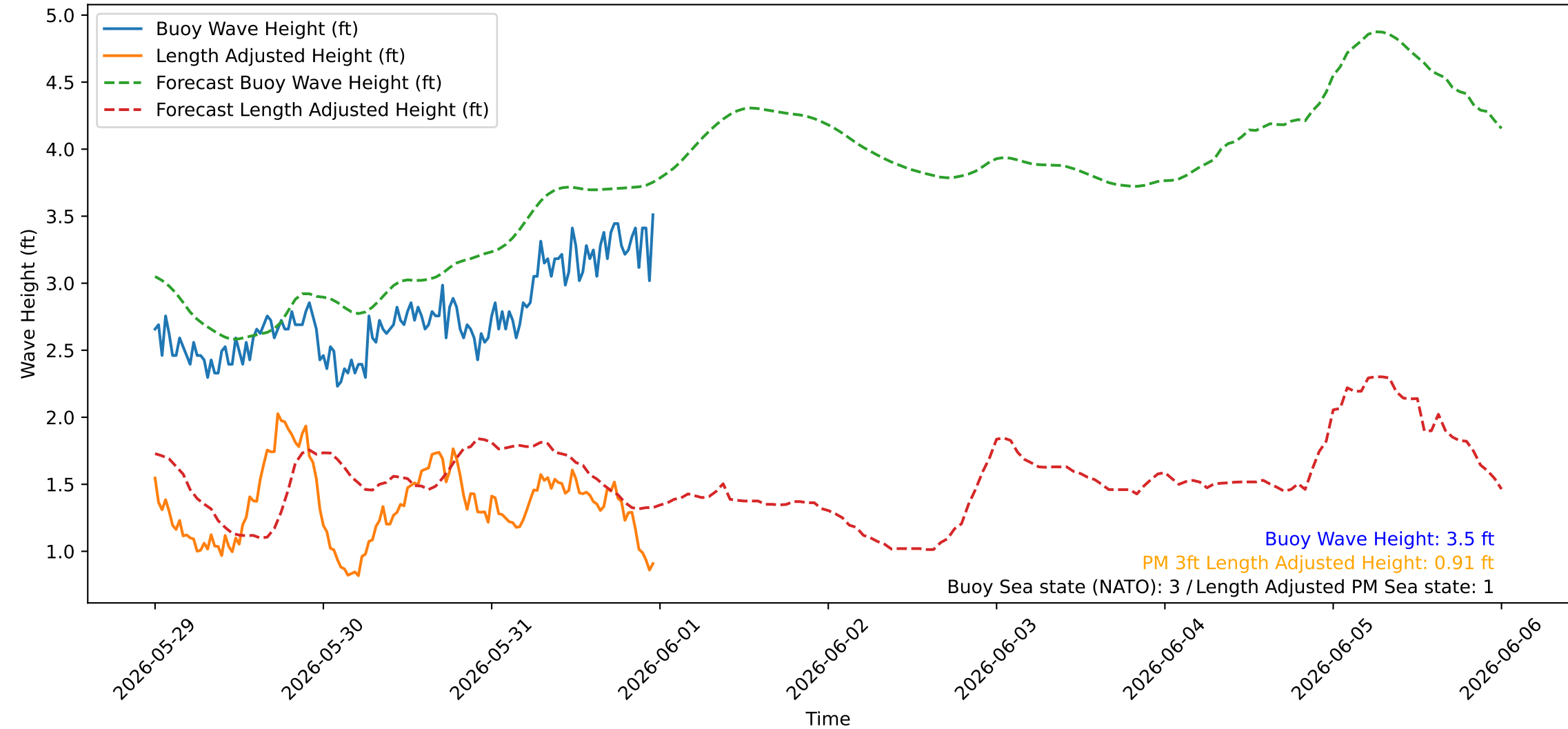
Wave Heights over Time for Red Beach at 2026-05-31 23:40:46
