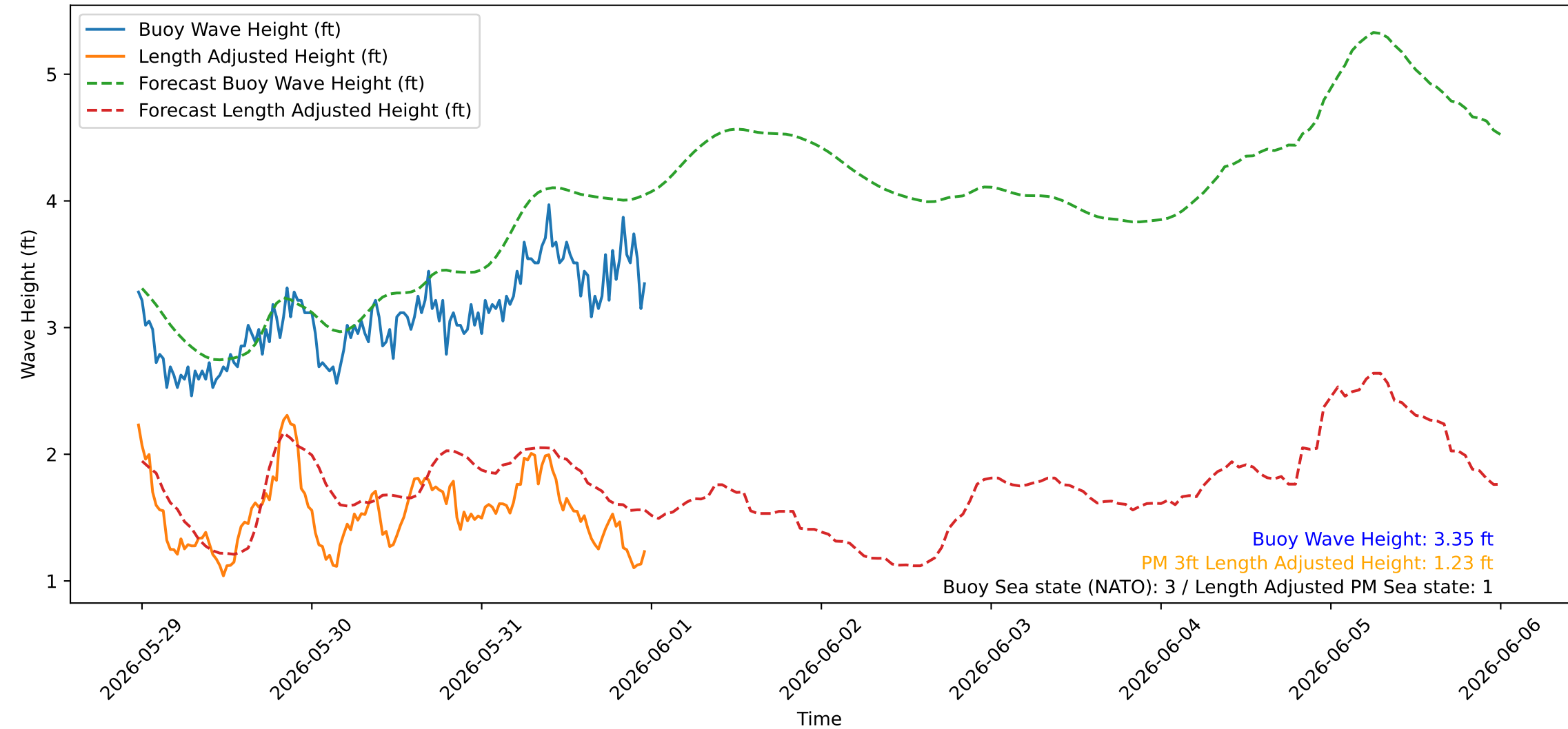
Wave Heights over Time for Green Beach at 2026-05-31 23:41:08
