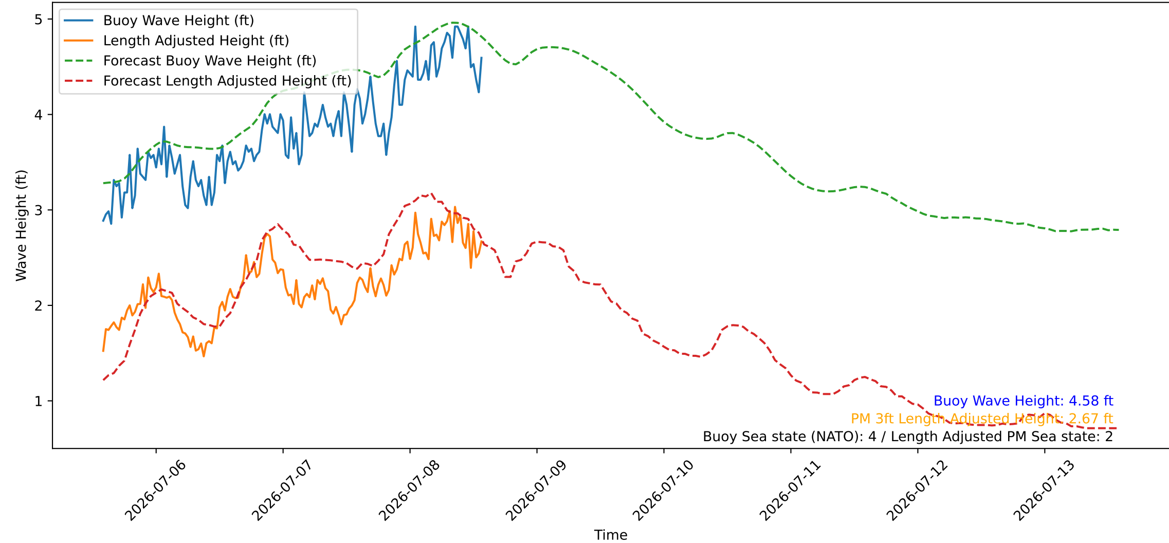
Wave Heights over Time for Oceanside Harbor at 2026-07-08 14:00:27
