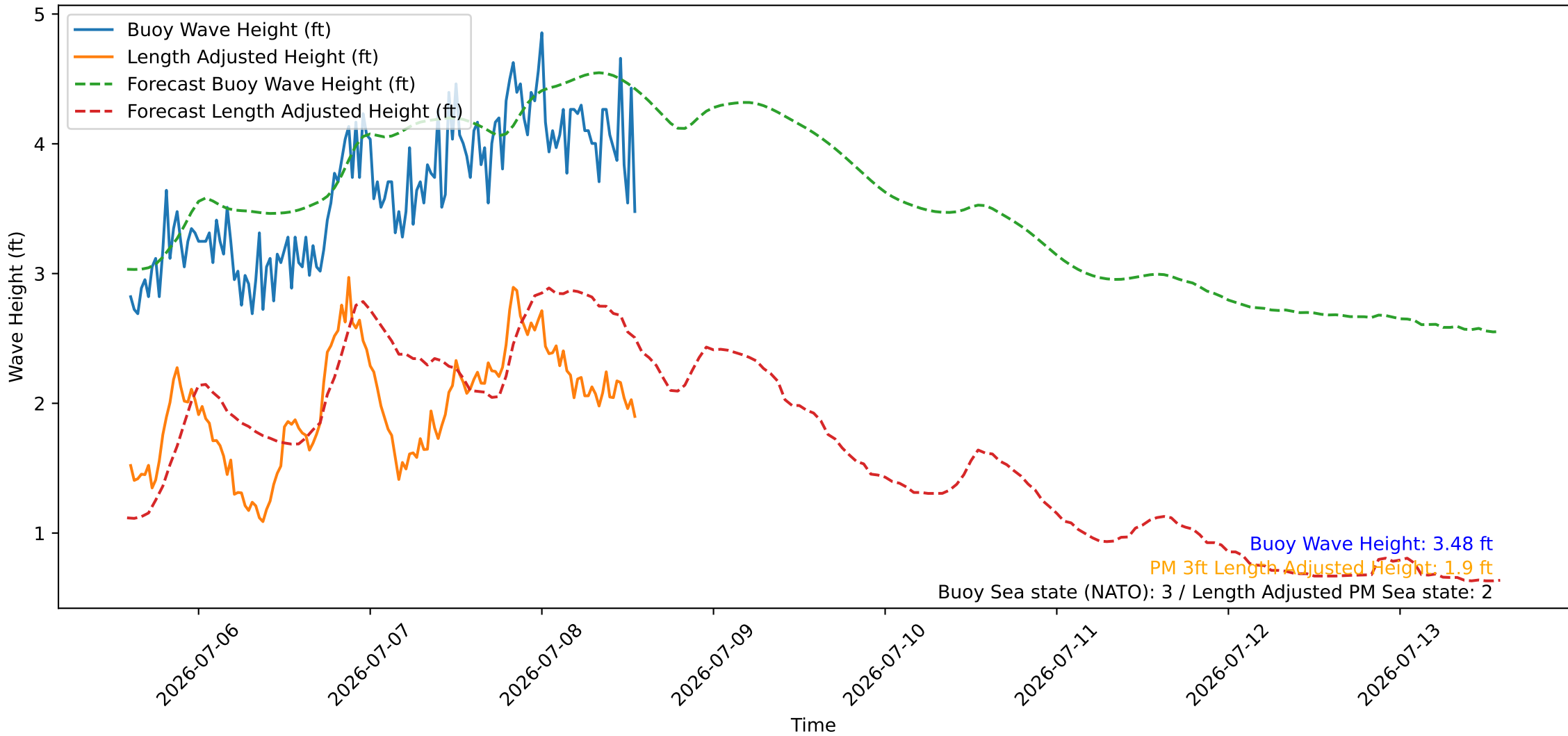
Wave Heights over Time for Red Beach at 2026-07-08 14:00:46
