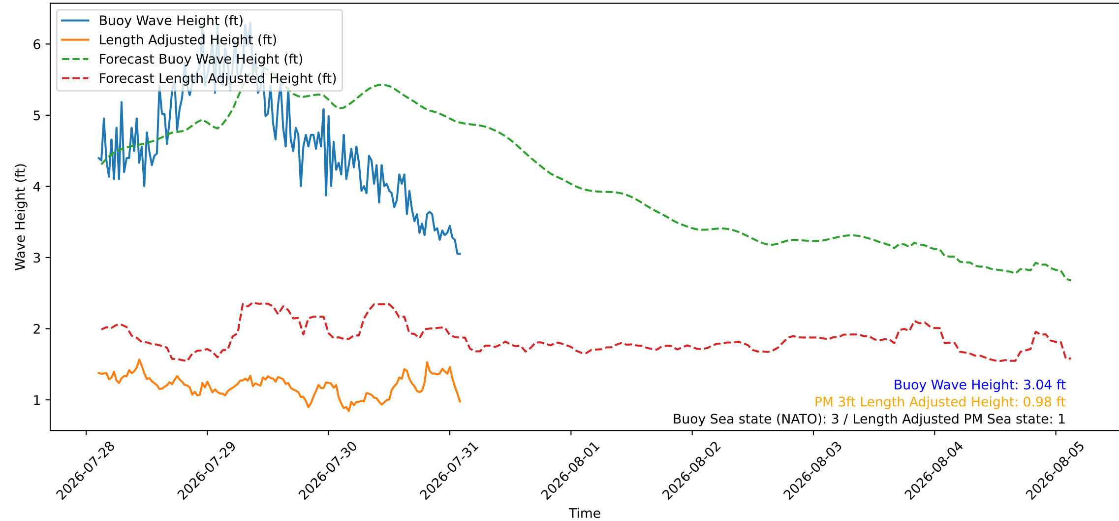
Wave Heights over Time for Green Beach at 2026-07-31 02:41:09
