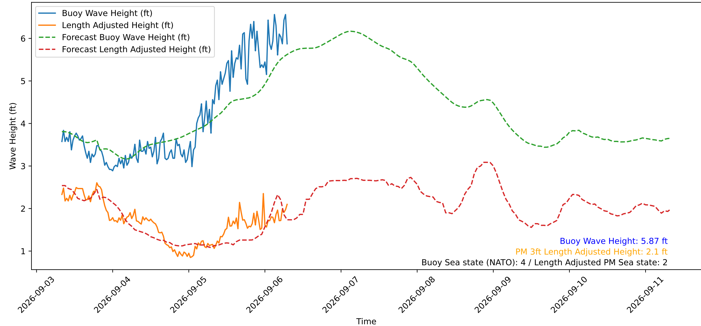
Wave Heights over Time for Oceanside Harbor at 2026-09-06 08:00:30
