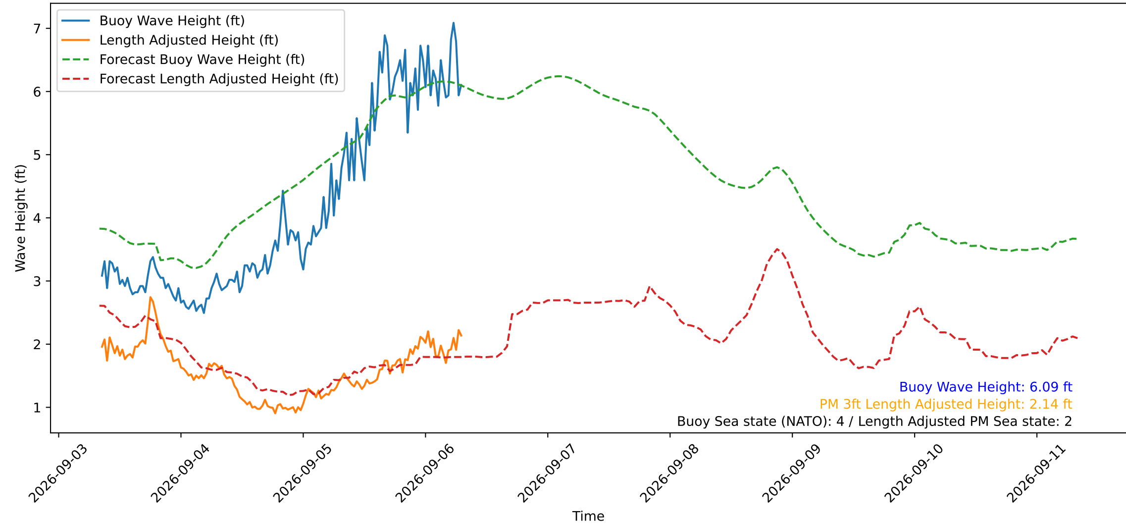
Wave Heights over Time for Green Beach at 2026-09-06 08:01:13
