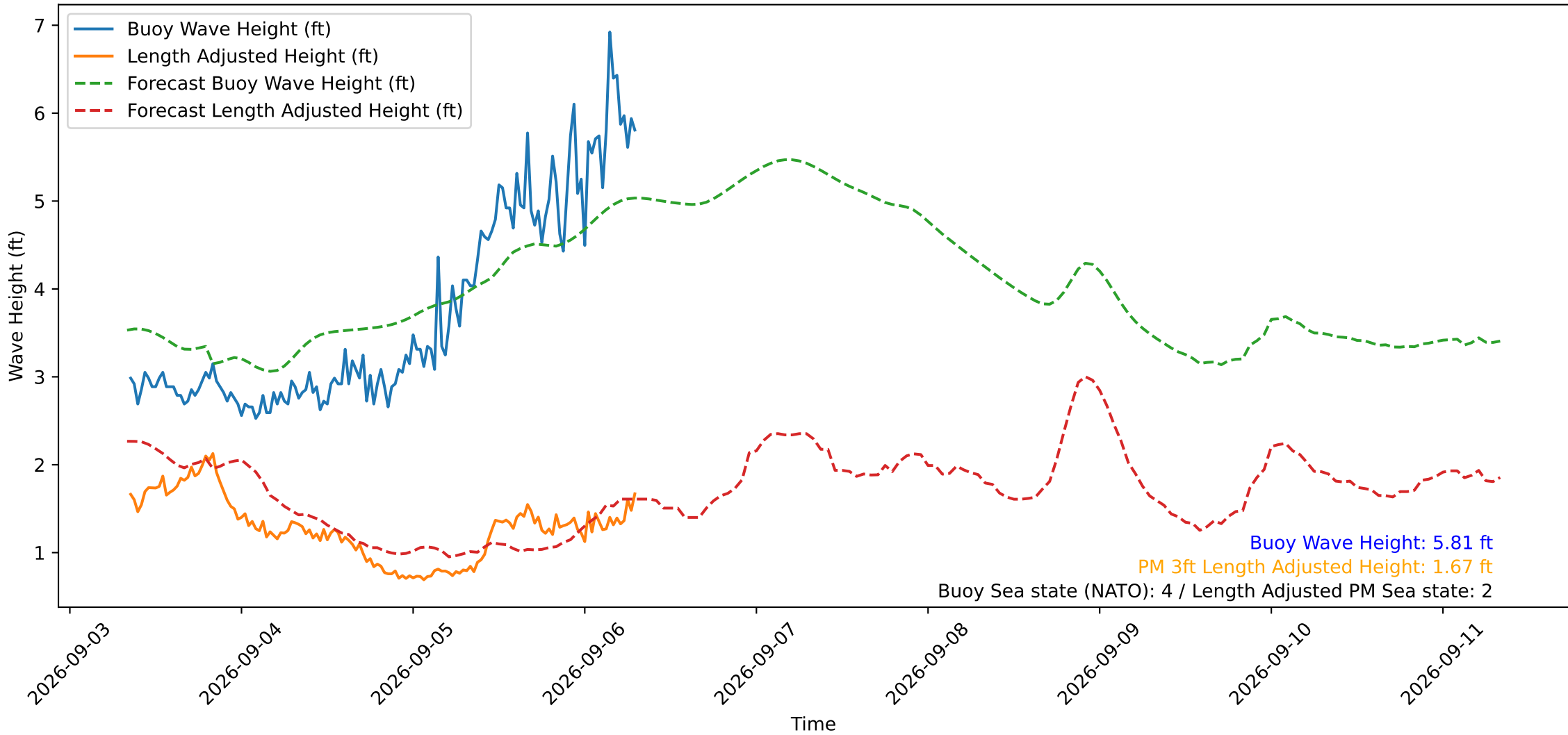
Wave Heights over Time for Red Beach at 2026-09-06 08:00:51
