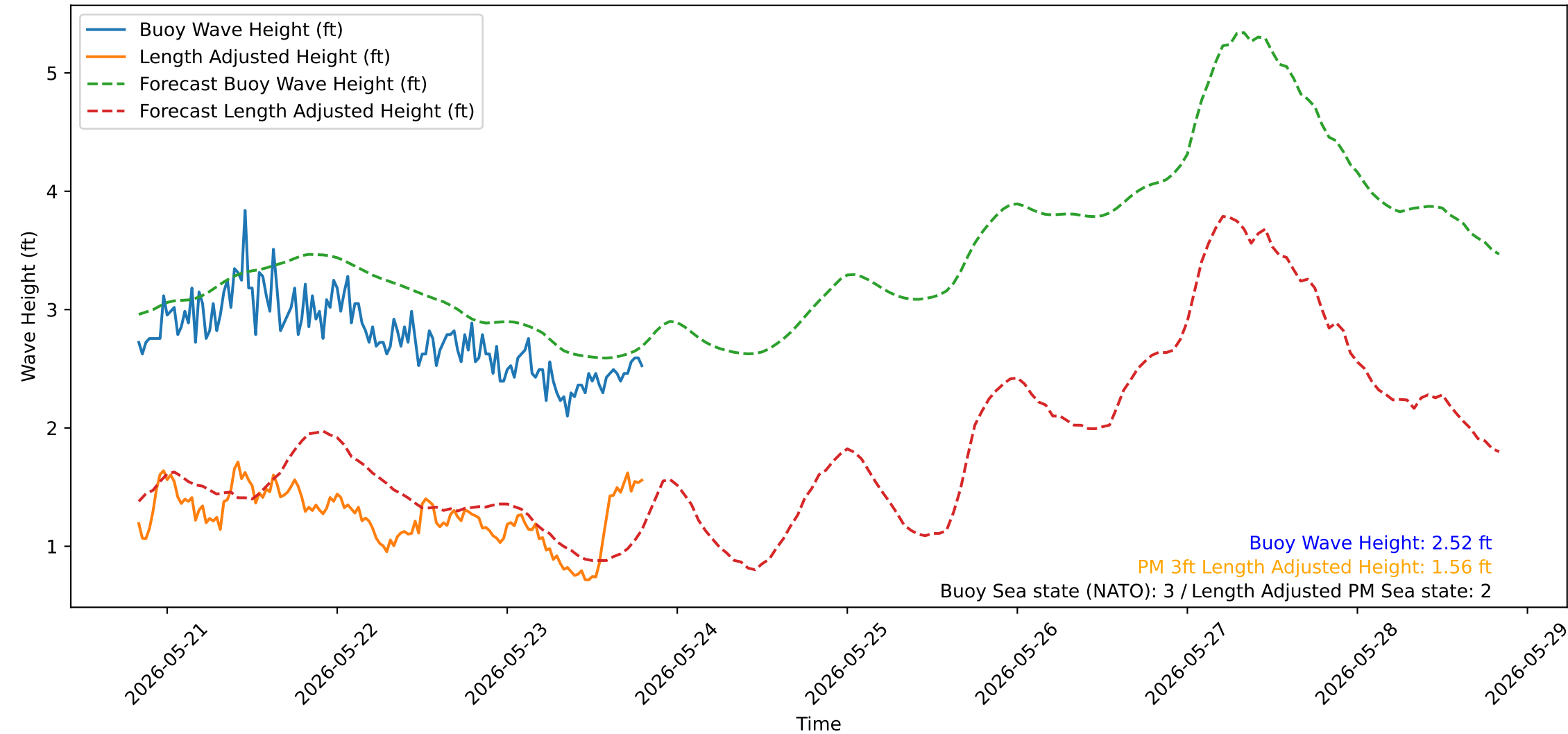
Wave Heights over Time for Oceanside Harbor at 2026-05-23 19:50:32
