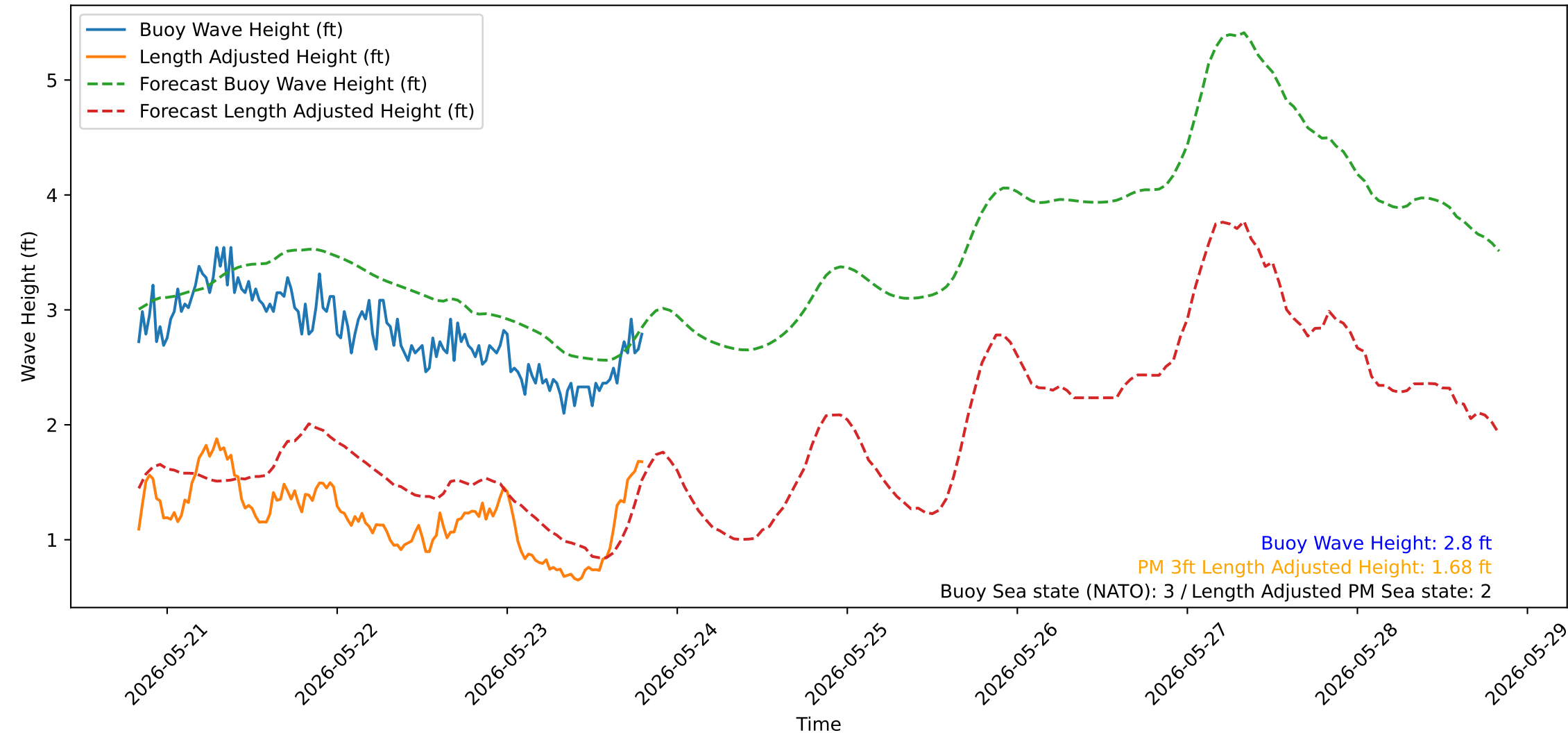
Wave Heights over Time for Green Beach at 2026-05-23 19:51:16
