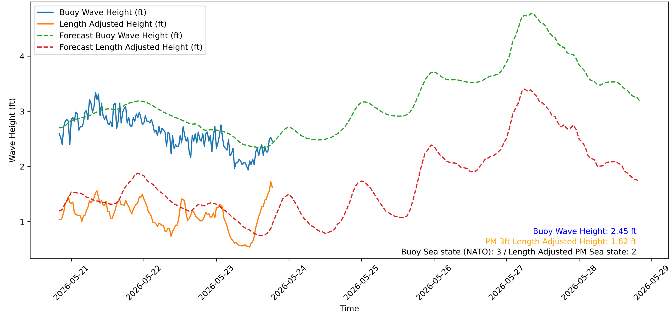
Wave Heights over Time for Red Beach at 2026-05-23 19:50:53
