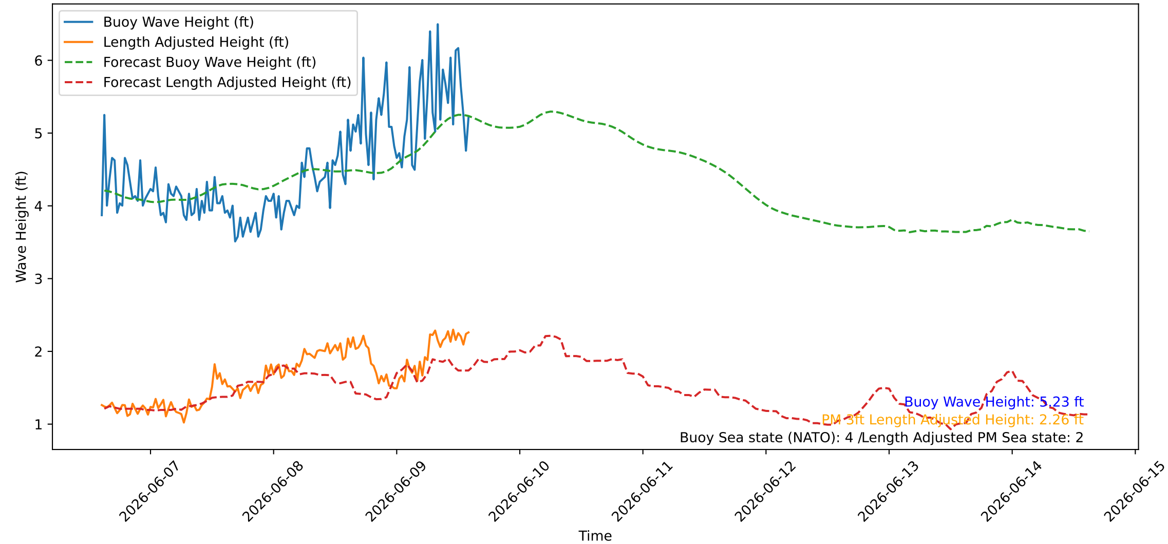
Wave Heights over Time for Oceanside Harbor at 2026-06-09 14:40:26
