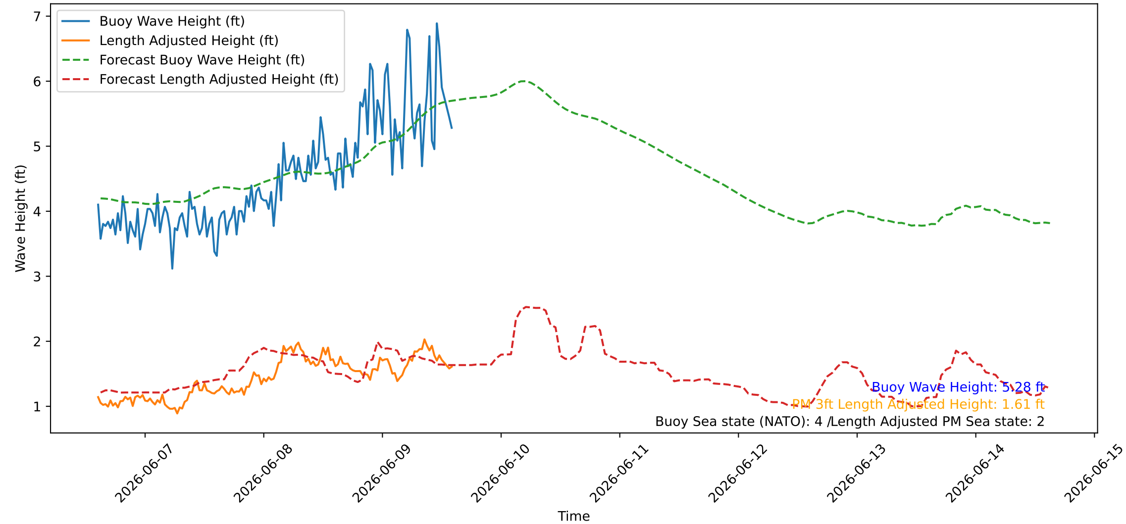
Wave Heights over Time for Green Beach at 2026-06-09 14:41:08
