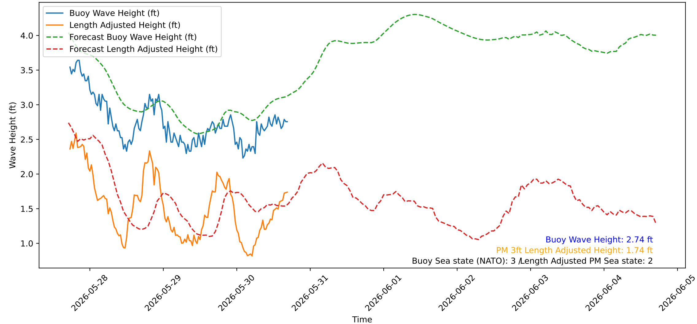
Wave Heights over Time for Red Beach at 2026-05-30 17:20:44
